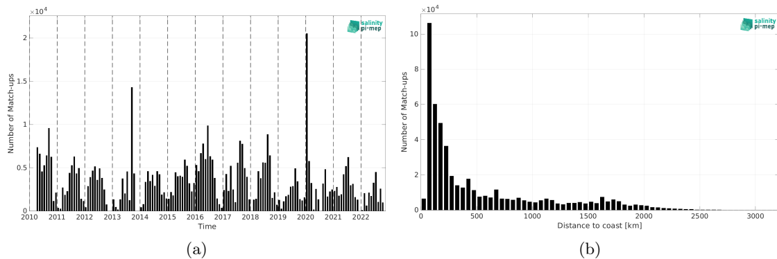
Figure 2: Number of match-ups between TSG (SAMOS) and CCI SSS L4 Merged-OI v4.41 - 30-day running (ESA) SSS as a function of time (a) and as function of the distance to coast (b) over the Pacific Ocean Pi-MEP region and for the full satellite product period.
