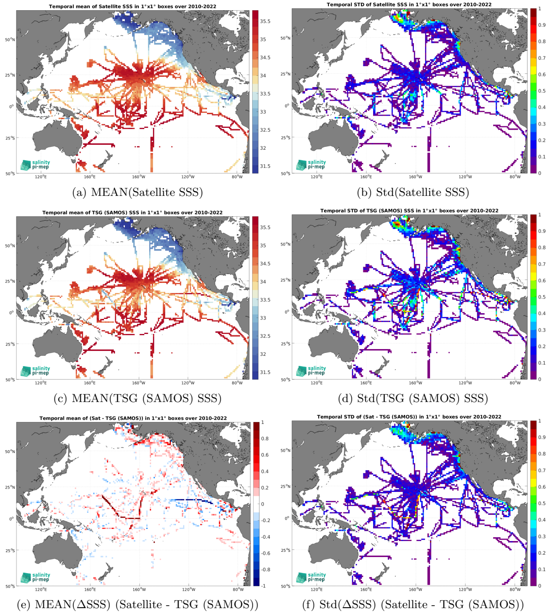
Figure 7: Temporal mean (left) and Std (right) of SSS from CCI SSS L4 Merged-OI v4.41 - 30-day running (ESA) (top), TSG (SAMOS) (middle), and of \Delta SSS (Satellite - TSG (SAMOS)). Only match-up pairs are used to generate these maps.
