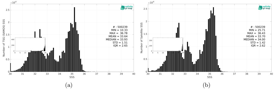
Figure 3: Histograms of SSS from TSG (SAMOS) (a) and CCI SSS L4 Merged-OI v4.41 - 30-day running (ESA) (b) considering all match-up pairs per bins of 0.1 over the Pacific Ocean Pi-MEP region and for the full satellite product period.
