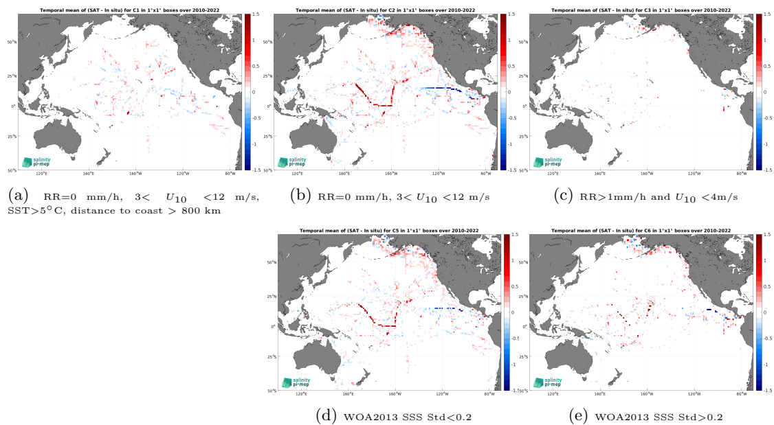
Figure 14: Temporal mean gridded over spatial boxes of size 1^\circ \times 1^\circ of \Delta SSS (CCI SSS L4 Merged-OI v4.41 - 30-day running (ESA) - TSG (SAMOS)) for 5 different subdatasets corresponding to:RR=0 mm/h, 3 < U_{10} < 12 m/s, SST > 5^\circ\text{C} , distance to coast > 800 km (a), RR=0 mm/h, 3 < U_{10} < 12 m/s (b), RR > 1 mm/h and U_{10} < 4 m/s (c), WOA2013 SSS Std < 0.2 (d), WOA2013 SSS Std > 0.2 (e).
