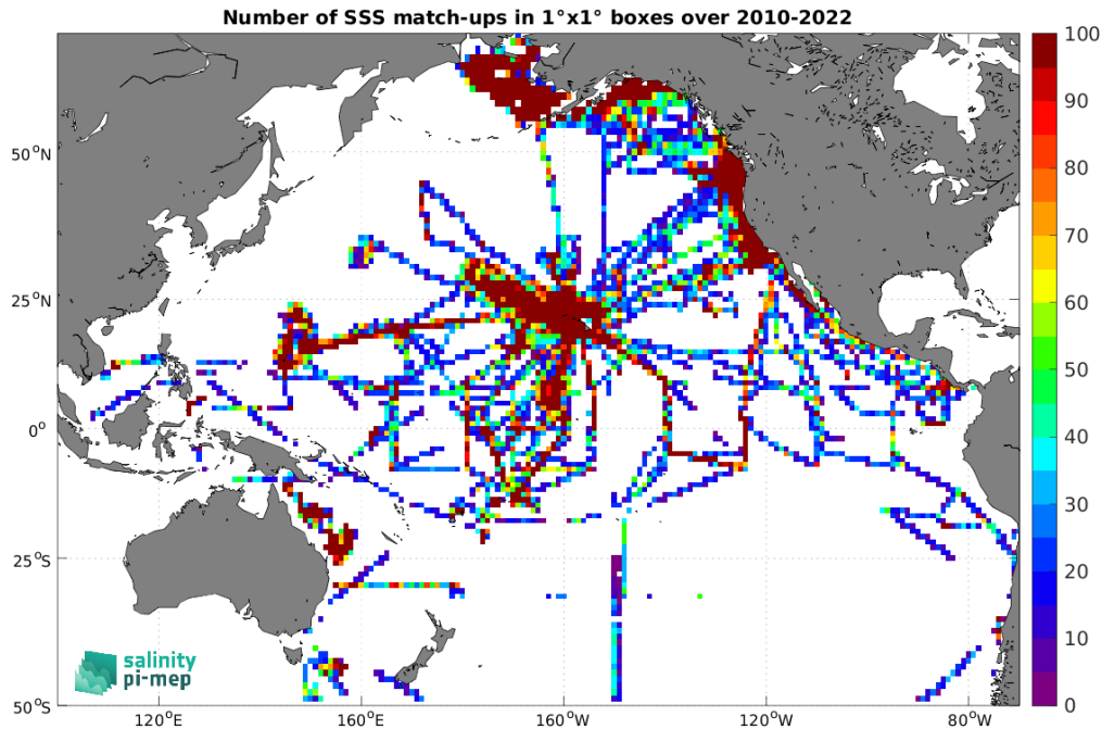
Figure 5: Number of SSS match-ups between TSG (SAMOS) SSS and the CCI SSS L4 Merged-OI v4.41 - 30-day running (ESA) SSS product for the Pacific Ocean Pi-MEP region over 1^\circ \times 1^\circ boxes and for the full satellite product period.
