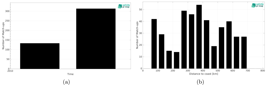
Figure 2: Number of match-ups between TSG (Polarstern) and CCI SSS L4 Merged-OI v4.41 - 30-day running (ESA) SSS as a function of time (a) and as function of the distance to coast (b) over the Pacific Ocean Pi-MEP region and for the full satellite product period.
