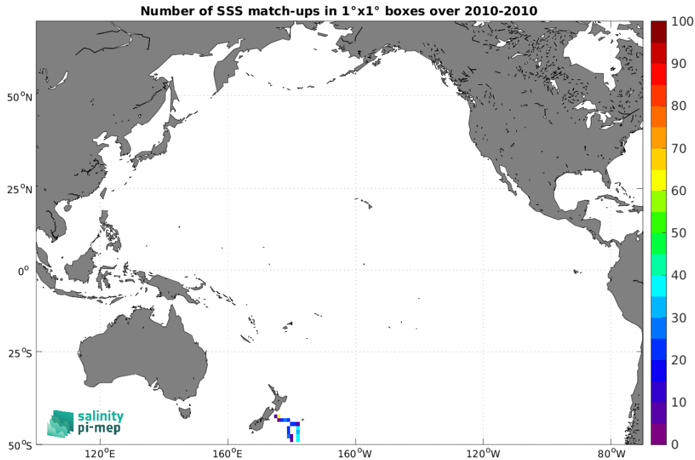
Figure 5: Number of SSS match-ups between TSG (Polarstern) SSS and the CCI SSS L4 Merged-OI v4.41 - 30-day running (ESA) SSS product for the Pacific Ocean Pi-MEP region over 1^\circ \times 1^\circ boxes and for the full satellite product period.
