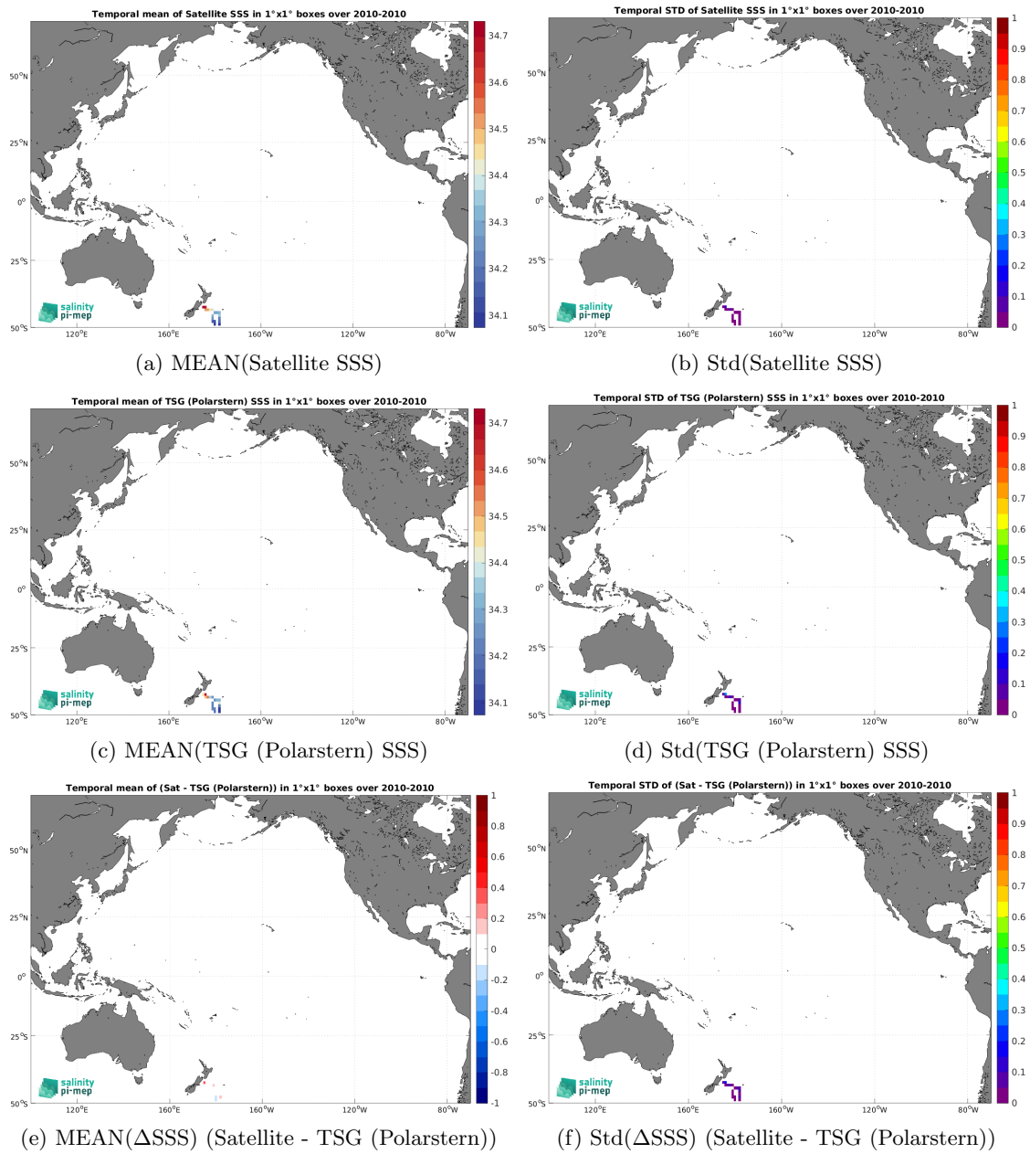
Figure 7: Temporal mean (left) and Std (right) of SSS from CCI SSS L4 Merged-OI v4.41 - 30-day running (ESA) (top), TSG (Polarstern) (middle), and of \Delta SSS (Satellite - TSG (Polarstern)). Only match-up pairs are used to generate these maps.
