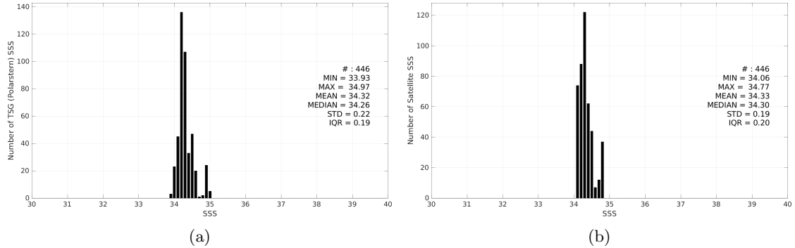
Figure 3: Histograms of SSS from TSG (Polarstern) (a) and CCI SSS L4 Merged-OI v4.41 - 30-day running (ESA) (b) considering all match-up pairs per bins of 0.1 over the Pacific Ocean Pi-MEP region and for the full satellite product period.
