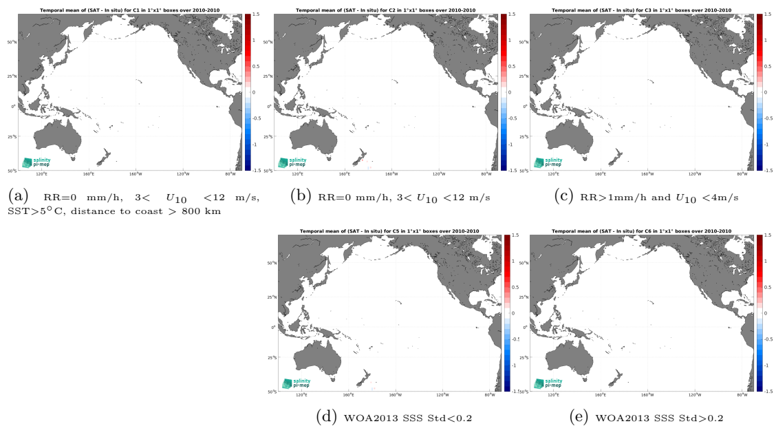
Figure 14: Temporal mean gridded over spatial boxes of size 1^\circ \times 1^\circ of \Delta SSS (CCI SSS L4 Merged-OI v4.41 - 30-day running (ESA) - TSG (Polarstern)) for 5 different subdatasets corresponding to:RR=0 mm/h, 3 < U_{10} < 12 m/s, SST >5^\circ C, distance to coast > 800 km (a), RR=0 mm/h, 3 < U_{10} < 12 m/s (b), RR >1 mm/h and U_{10} < 4 m/s (c), WOA2013 SSS Std <0.2 (d), WOA2013 SSS Std >0.2 (e).
