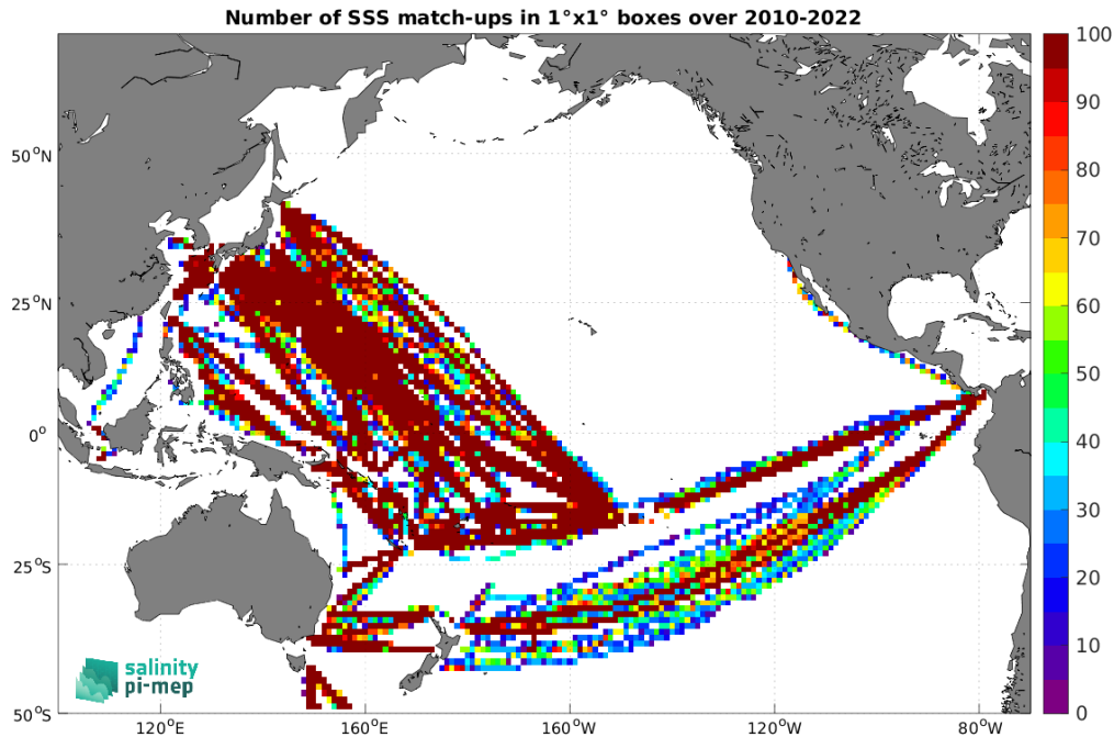
Figure 5: Number of SSS match-ups between TSG (LEGOS-DM) SSS and the CCI SSS L4 Merged-OI v4.41 - 30-day running (ESA) SSS product for the Pacific Ocean Pi-MEP region over 1^\circ \times 1^\circ boxes and for the full satellite product period.
