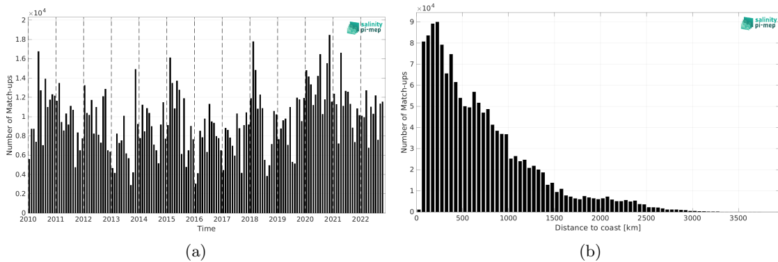
Figure 2: Number of match-ups between TSG (LEGOS-DM) and CCI SSS L4 Merged-OI v4.41 - 30-day running (ESA) SSS as a function of time (a) and as function of the distance to coast (b) over the Pacific Ocean Pi-MEP region and for the full satellite product period.
