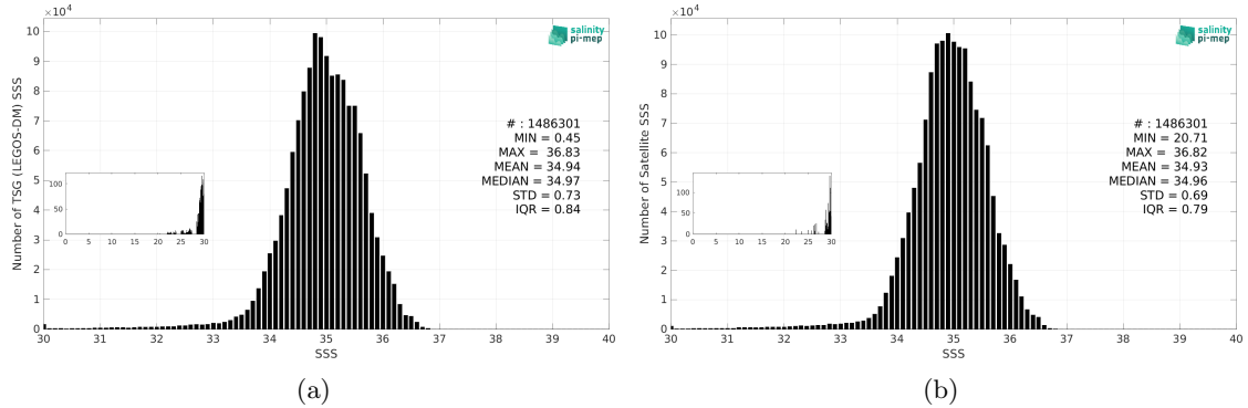
Figure 3: Histograms of SSS from TSG (LEGOS-DM) (a) and CCI SSS L4 Merged-OI v4.41 - 30-day running (ESA) (b) considering all match-up pairs per bins of 0.1 over the Pacific Ocean Pi-MEP region and for the full satellite product period.
