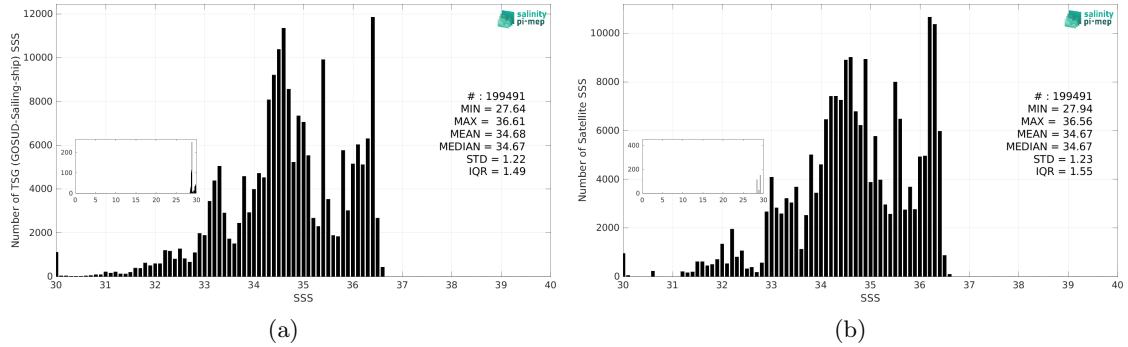
Figure 3: Histograms of SSS from TSG (GOSUD-Sailing-ship) (a) and CCI SSS L4 Merged-OI v4.41 - 30-day running (ESA) (b) considering all match-up pairs per bins of 0.1 over the Pacific Ocean Pi-MEP region and for the full satellite product period.
