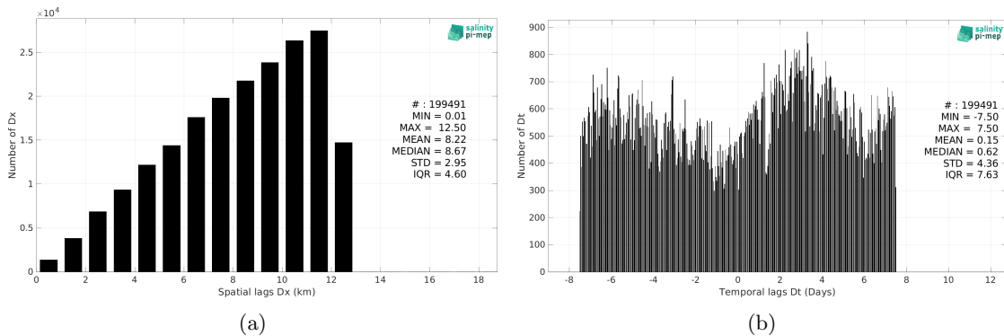
Figure 6: Histograms of the spatial (a) and temporal (b) lags between the location/time of the TSG (GOSUD-Sailing-ship) measurement and the date of the corresponding CCI SSS L4 Merged-OI v4.41 - 30-day running (ESA) SSS pixel.
