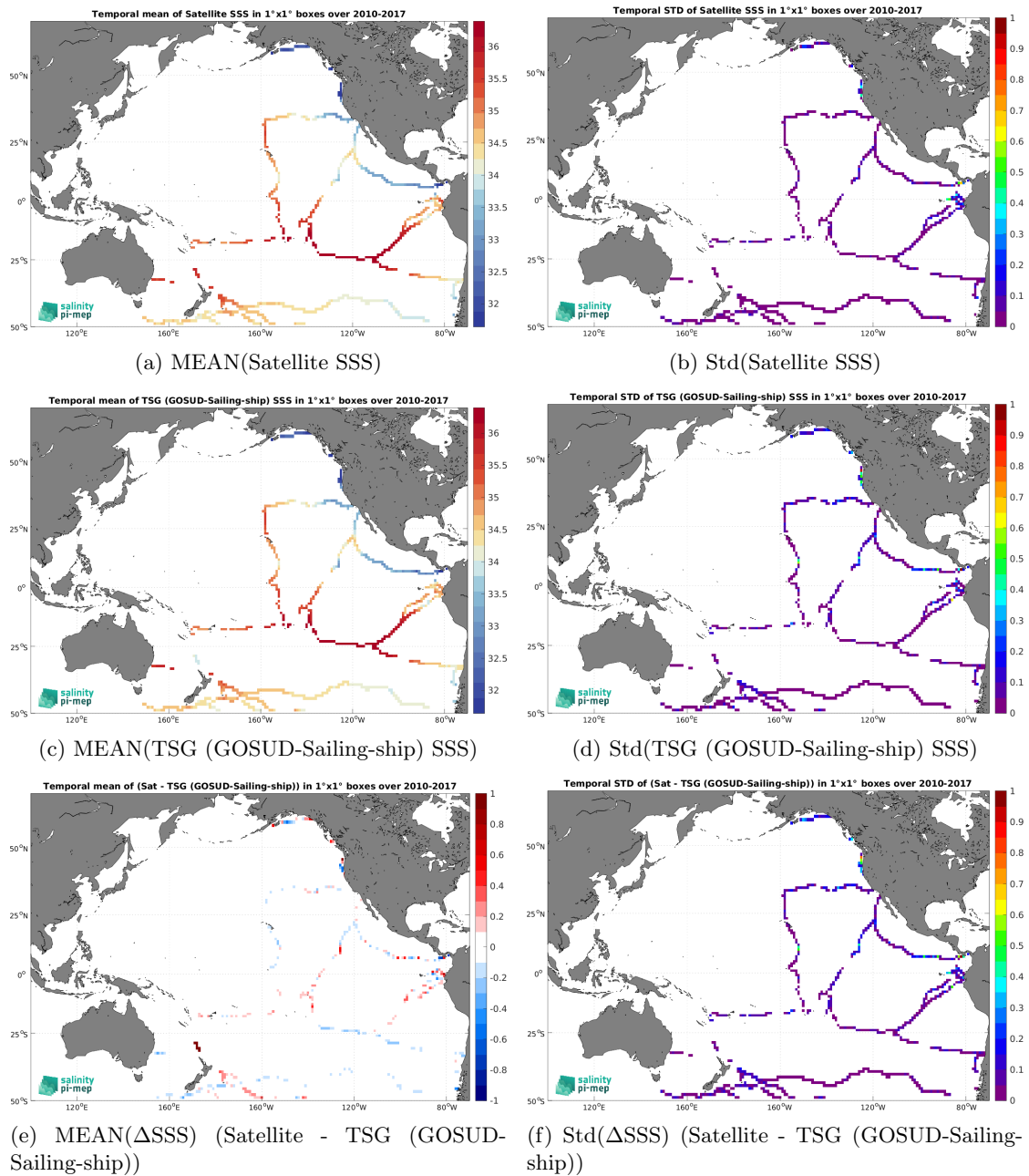
Figure 7: Temporal mean (left) and Std (right) of SSS from CCI SSS L4 Merged-OI v4.41 - 30-day running (ESA) (top), TSG (GOSUD-Sailing-ship) (middle), and of \Delta SSS (Satellite - TSG (GOSUD-Sailing-ship)). Only match-up pairs are used to generate these maps.
