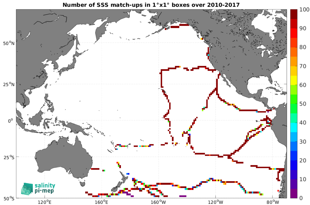
Figure 5: Number of SSS match-ups between TSG (GOSUD-Sailing-ship) SSS and the CCI SSS L4 Merged-OI v4.41 - 30-day running (ESA) SSS product for the Pacific Ocean Pi-MEP region over 1^\circ \times 1^\circ boxes and for the full satellite product period.
