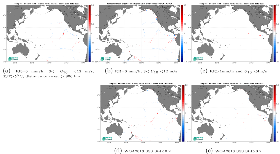
Figure 14: Temporal mean gridded over spatial boxes of size 1^\circ \times 1^\circ of \Delta SSS (CCI SSS L4 Merged-OI v4.41 - 30-day running (ESA) - TSG (GOSUD-Sailing-ship)) for 5 different subdatasets corresponding to:RR=0 mm/h, 3 < U_{10} < 12 m/s, SST >5^\circ C, distance to coast > 800 km (a), RR=0 mm/h, 3 < U_{10} < 12 m/s (b), RR >1 mm/h and U_{10} < 4 m/s (c), WOA2013 SSS Std <0.2 (d), WOA2013 SSS Std >0.2 (e).
