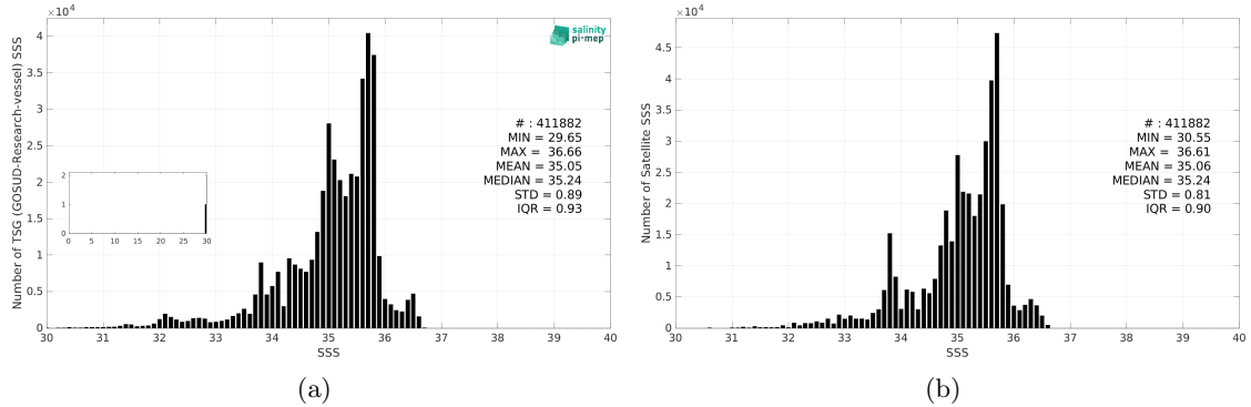
Figure 3: Histograms of SSS from TSG (GOSUD-Research-vessel) (a) and CCI SSS L4 Merged-OI v4.41 - 30-day running (ESA) (b) considering all match-up pairs per bins of 0.1 over the Pacific Ocean Pi-MEP region and for the full satellite product period.
