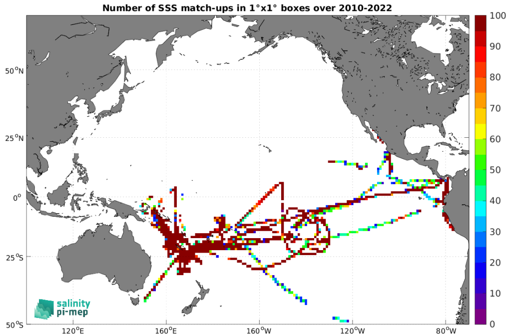
Figure 5: Number of SSS match-ups between TSG (GOSUD-Research-vessel) SSS and the CCI SSS L4 Merged-OI v4.41 - 30-day running (ESA) SSS product for the Pacific Ocean Pi-MEP region over 1^\circ \times 1^\circ boxes and for the full satellite product period.
