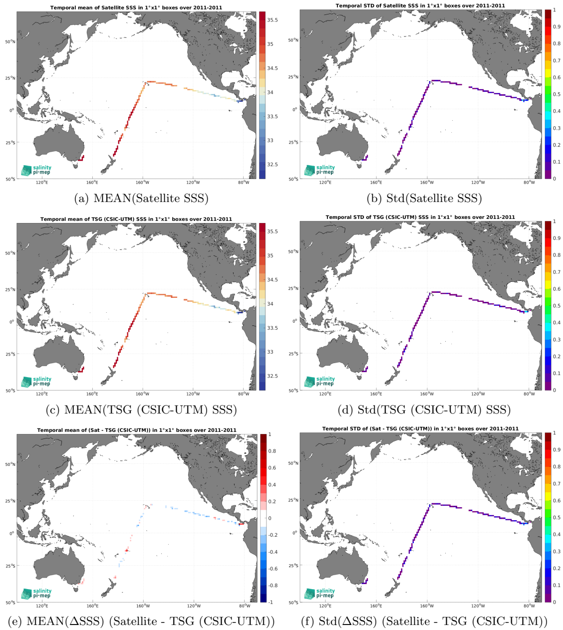
Figure 7: Temporal mean (left) and Std (right) of SSS from CCI SSS L4 Merged-OI v4.41 - 30-day running (ESA) (top), TSG (CSIC-UTM) (middle), and of \Delta SSS (Satellite - TSG (CSIC-UTM)). Only match-up pairs are used to generate these maps.
