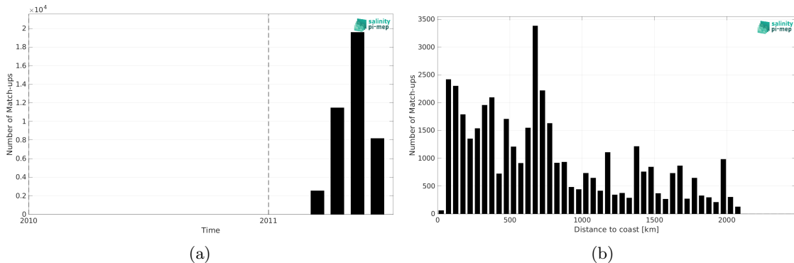
Figure 2: Number of match-ups between TSG (CSIC-UTM) and CCI SSS L4 Merged-OI v4.41 - 30-day running (ESA) SSS as a function of time (a) and as function of the distance to coast (b) over the Pacific Ocean Pi-MEP region and for the full satellite product period.
