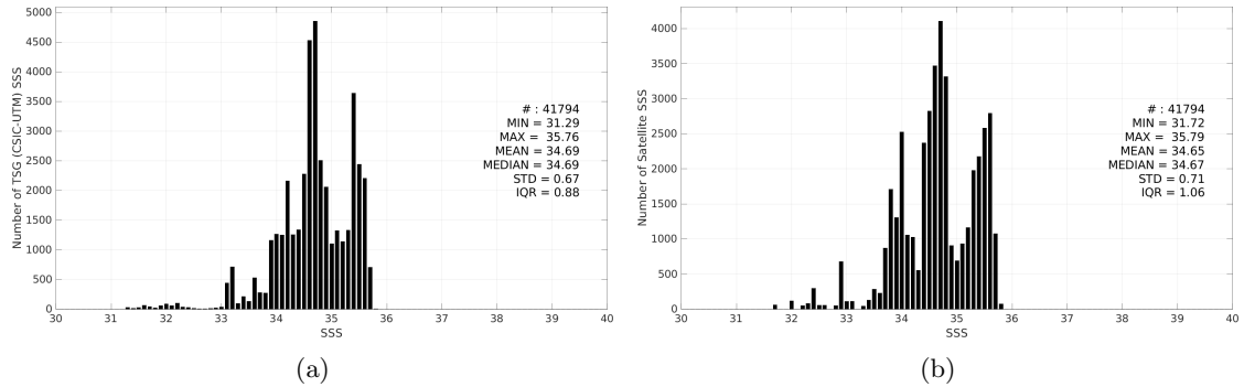
Figure 3: Histograms of SSS from TSG (CSIC-UTM) (a) and CCI SSS L4 Merged-OI v4.41 - 30-day running (ESA) (b) considering all match-up pairs per bins of 0.1 over the Pacific Ocean Pi-MEP region and for the full satellite product period.
