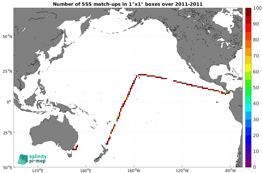
Figure 5: Number of SSS match-ups between TSG (CSIC-UTM) SSS and the CCI SSS L4 Merged-OI v4.41 - 30-day running (ESA) SSS product for the Pacific Ocean Pi-MEP region over 1^\circ \times 1^\circ boxes and for the full satellite product period.
