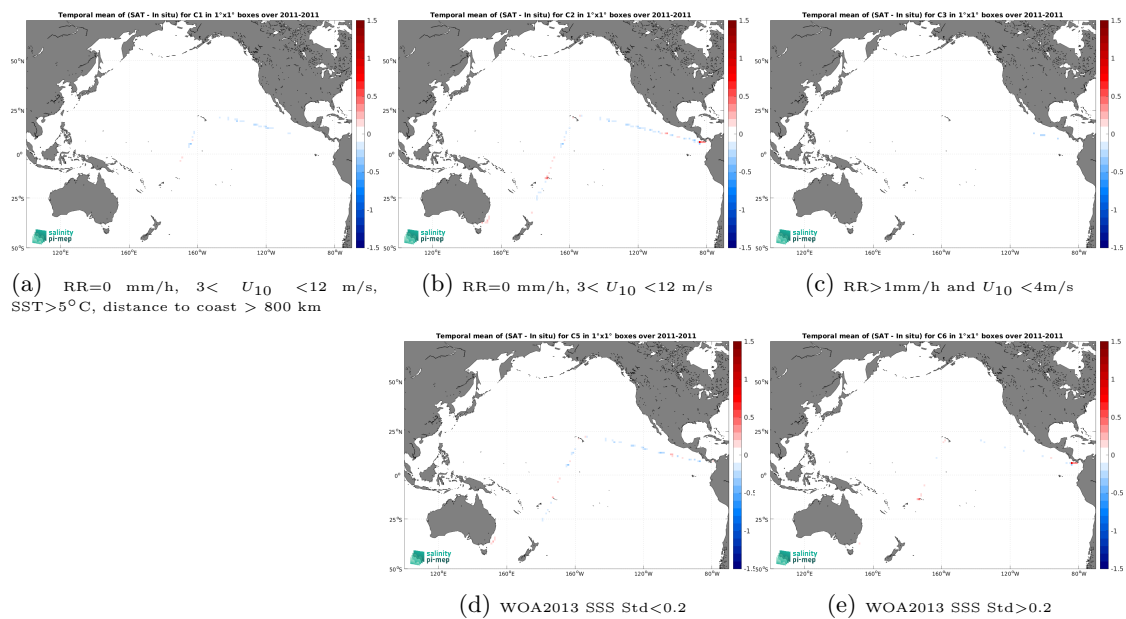
Figure 14: Temporal mean gridded over spatial boxes of size 1^\circ \times 1^\circ of \Delta SSS (CCI SSS L4 Merged-OI v4.41 - 30-day running (ESA) - TSG (CSIC-UTM)) for 5 different subdatasets corresponding to:RR=0 mm/h, 3 < U_{10} < 12 m/s, SST >5^\circ C, distance to coast > 800 km (a), RR=0 mm/h, 3 < U_{10} < 12 m/s (b), RR >1 mm/h and U_{10} < 4 m/s (c), WOA2013 SSS Std <0.2 (d), WOA2013 SSS Std >0.2 (e).
