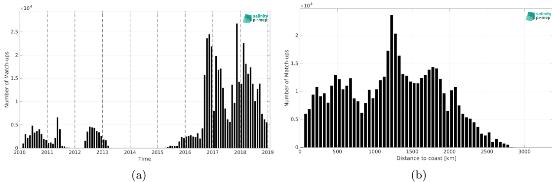
Figure 2: Number of match-ups between Surface drifters and CCI SSS L4 Merged-OI v4.41 - 30-day running (ESA) SSS as a function of time (a) and as function of the distance to coast (b) over the Pacific Ocean Pi-MEP region and for the full satellite product period.
