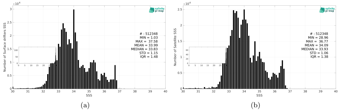
Figure 3: Histograms of SSS from Surface drifters (a) and CCI SSS L4 Merged-OI v4.41 - 30-day running (ESA) (b) considering all match-up pairs per bins of 0.1 over the Pacific Ocean Pi-MEP region and for the full satellite product period.
