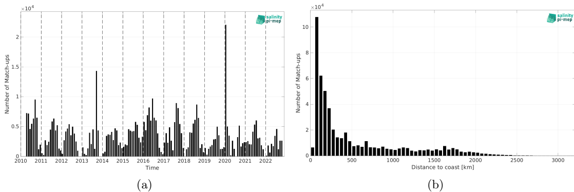
Figure 1: Number of match-ups between TSG (SAMOS) and CCI SSS L4 Merged-OI v4.4 - 7-day running (ESA) SSS as a function of time (a) and as function of the distance to coast (b) over the Pacific Ocean Pi-MEP region and for the full satellite product period.
