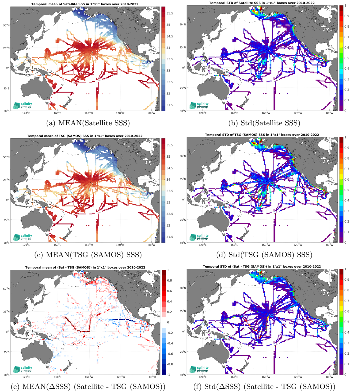
Figure 6: Temporal mean (left) and Std (right) of SSS from CCI SSS L4 Merged-OI v4.4 - 7-day running (ESA) (top), TSG (SAMOS) (middle), and of \Delta SSS (Satellite - TSG (SAMOS)). Only match-up pairs are used to generate these maps.
