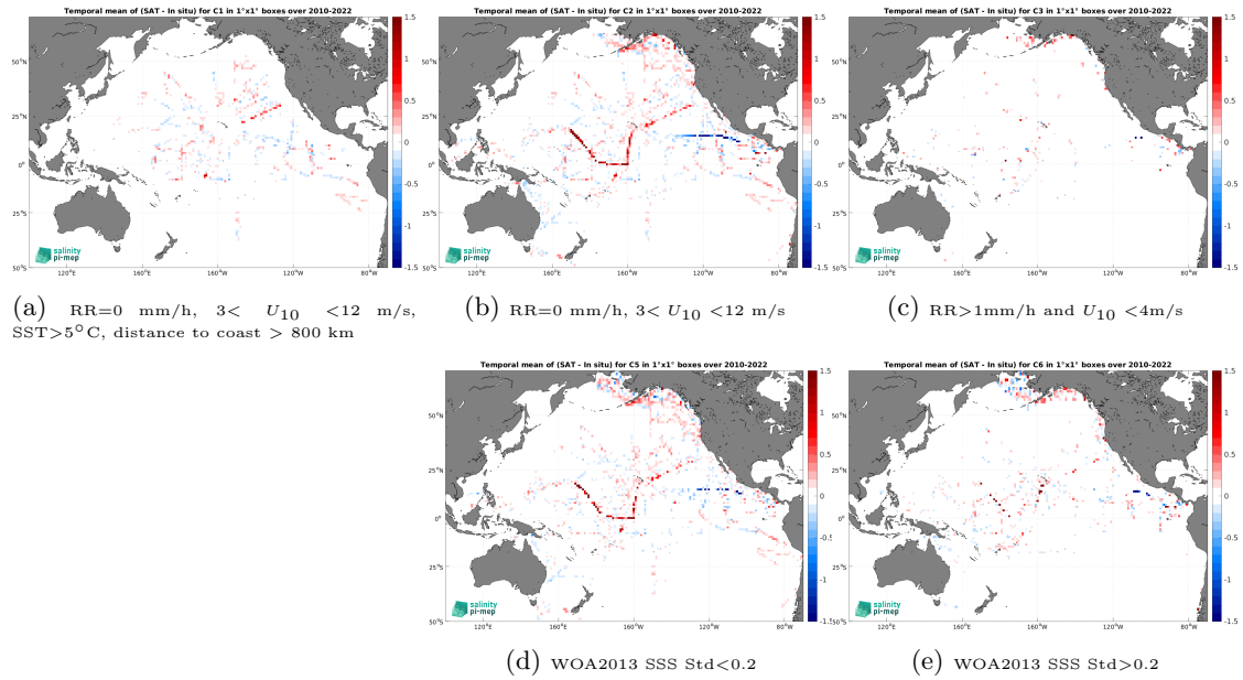
Figure 12: Temporal mean gridded over spatial boxes of size 1^\circ \times 1^\circ of \Delta SSS (CCI SSS L4 Merged-OI v4.4 - 7-day running (ESA) - TSG (SAMOS)) for 5 different subdatasets corresponding to: RR=0 mm/h, 3 < U_{10} < 12 m/s, SST > 5^\circ\text{C} , distance to coast > 800 km (a), RR=0 mm/h, 3 < U_{10} < 12 m/s (b), RR > 1 mm/h and U_{10} < 4 m/s (c), WOA2013 SSS Std < 0.2 (d), WOA2013 SSS Std > 0.2 (e).
