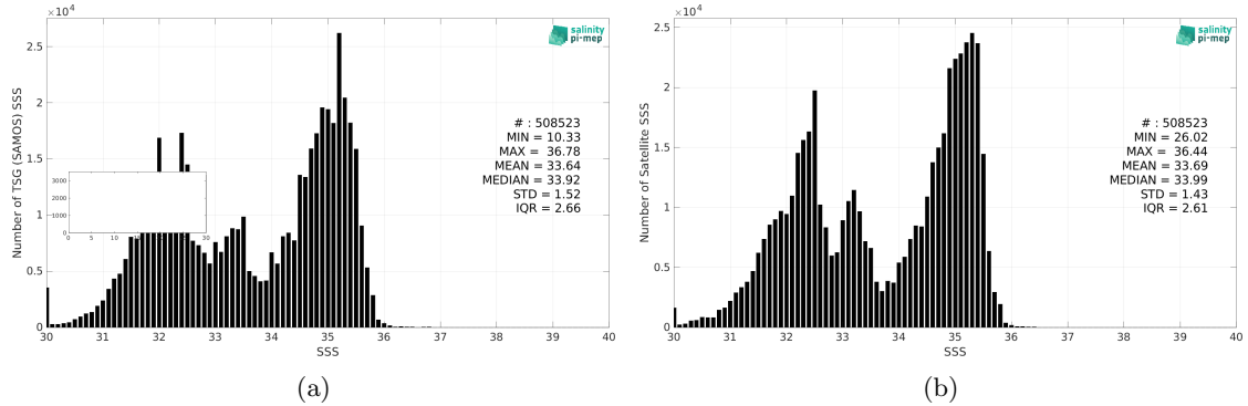
Figure 2: Histograms of SSS from TSG (SAMOS) (a) and CCI SSS L4 Merged-OI v4.4 - 7-day running (ESA) (b) considering all match-up pairs per bins of 0.1 over the Pacific Ocean Pi-MEP region and for the full satellite product period.
