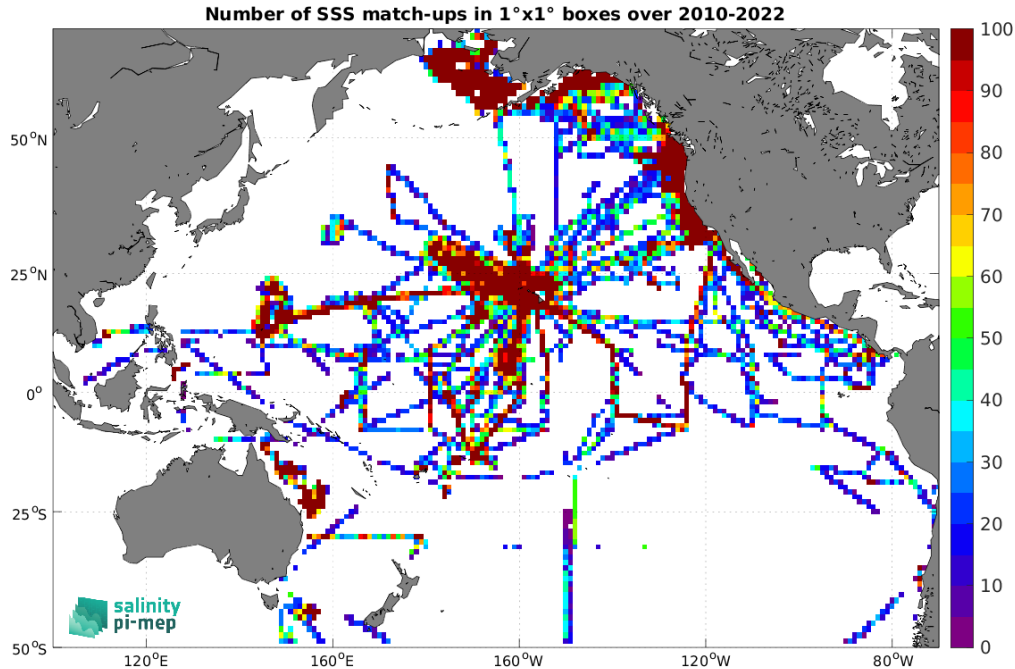
Figure 4: Number of SSS match-ups between TSG (SAMOS) SSS and the CCI SSS L4 Merged-OI v4.4 - 7-day running (ESA) SSS product for the Pacific Ocean Pi-MEP region over 1^\circ \times 1^\circ boxes and for the full satellite product period.
