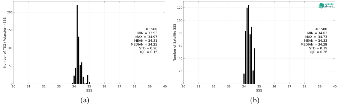
Figure 2: Histograms of SSS from TSG (Polarstern) (a) and CCI SSS L4 Merged-OI v4.4 - 7-day running (ESA) (b) considering all match-up pairs per bins of 0.1 over the Pacific Ocean Pi-MEP region and for the full satellite product period.
