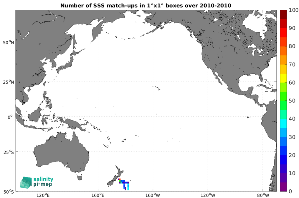
Figure 4: Number of SSS match-ups between TSG (Polarstern) SSS and the CCI SSS L4 Merged-OI v4.4 - 7-day running (ESA) SSS product for the Pacific Ocean Pi-MEP region over 1^\circ \times 1^\circ boxes and for the full satellite product period.
