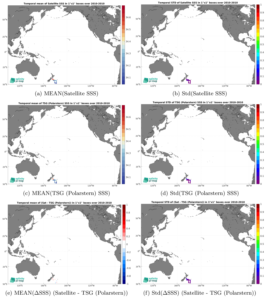
Figure 6: Temporal mean (left) and Std (right) of SSS from CCI SSS L4 Merged-OI v4.4 - 7-day running (ESA) (top), TSG (Polarstern) (middle), and of \Delta SSS (Satellite - TSG (Polarstern)). Only match-up pairs are used to generate these maps.
