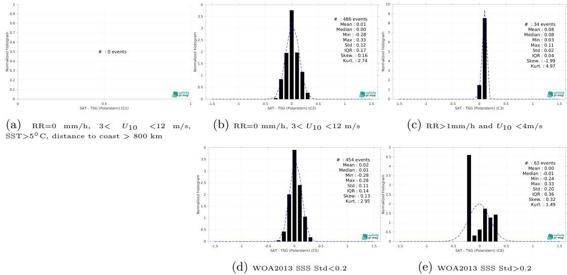
Figure 13: Normalized histogram of \Delta SSS (CCI SSS L4 Merged-OI v4.4 - 7-day running (ESA) - TSG (Polarstern)) for 5 different subdatasets corresponding to: RR=0 mm/h, 3 < U_{10} < 12 m/s, SST > 5°C, distance to coast > 800 km (a), RR=0 mm/h, 3 < U_{10} < 12 m/s (b), RR > 1mm/h and U_{10} < 4 m/s (c), WOA2013 SSS Std < 0.2 (d), WOA2013 SSS Std > 0.2 (e).
