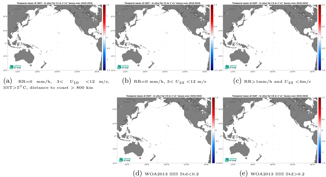
Figure 12: Temporal mean gridded over spatial boxes of size 1^{\circ}\times 1^{\circ} of \Delta\text{SSS} (CCI SSS L4 Merged-OI v4.4 - 7-day running (ESA) - TSG (Polarstern)) for 5 different subdatasets corresponding to:RR=0 mm/h, 3 < U_{10} < 12 m/s, SST >5^{\circ}\text{C} , distance to coast > 800 km (a), RR=0 mm/h, 3 < U_{10} < 12 m/s (b), RR >1 mm/h and U_{10} < 4 m/s (c), WOA2013 SSS Std <0.2 (d), WOA2013 SSS Std >0.2 (e).
