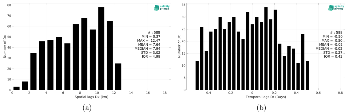
Figure 5: Histograms of the spatial (a) and temporal (b) lags between the location/time of the TSG (Polarstern) measurement and the date of the corresponding CCI SSS L4 Merged-OI v4.4 - 7-day running (ESA) SSS pixel.
