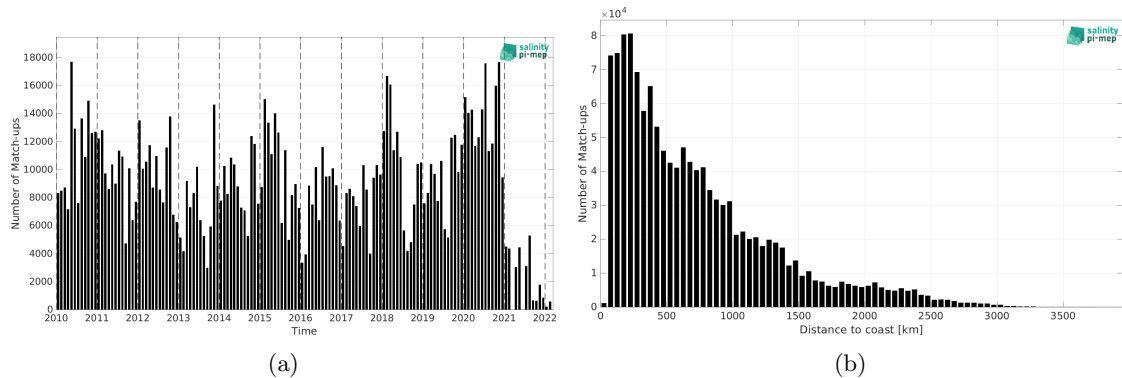
Figure 1: Number of match-ups between TSG (LEGOS-DM) and CCI SSS L4 Merged-OI v4.4 - 7-day running (ESA) SSS as a function of time (a) and as function of the distance to coast (b) over the Pacific Ocean Pi-MEP region and for the full satellite product period.
