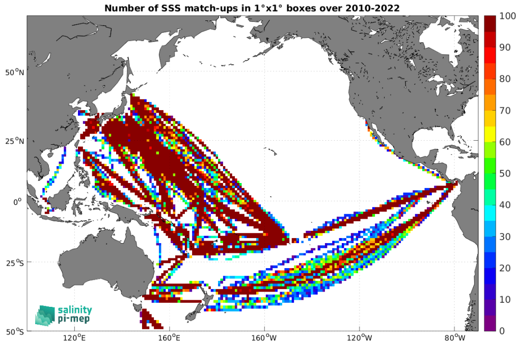
Figure 4: Number of SSS match-ups between TSG (LEGOS-DM) SSS and the CCI SSS L4 Merged-OI v4.4 - 7-day running (ESA) SSS product for the Pacific Ocean Pi-MEP region over 1^\circ \times 1^\circ boxes and for the full satellite product period.
