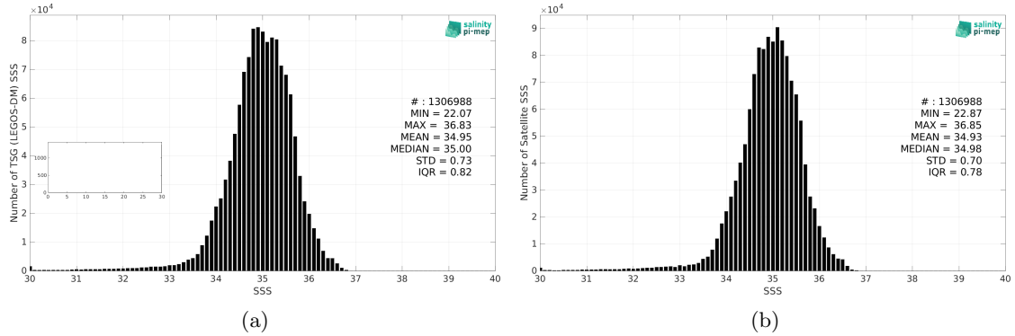
Figure 2: Histograms of SSS from TSG (LEGOS-DM) (a) and CCI SSS L4 Merged-OI v4.4 - 7-day running (ESA) (b) considering all match-up pairs per bins of 0.1 over the Pacific Ocean Pi-MEP region and for the full satellite product period.
