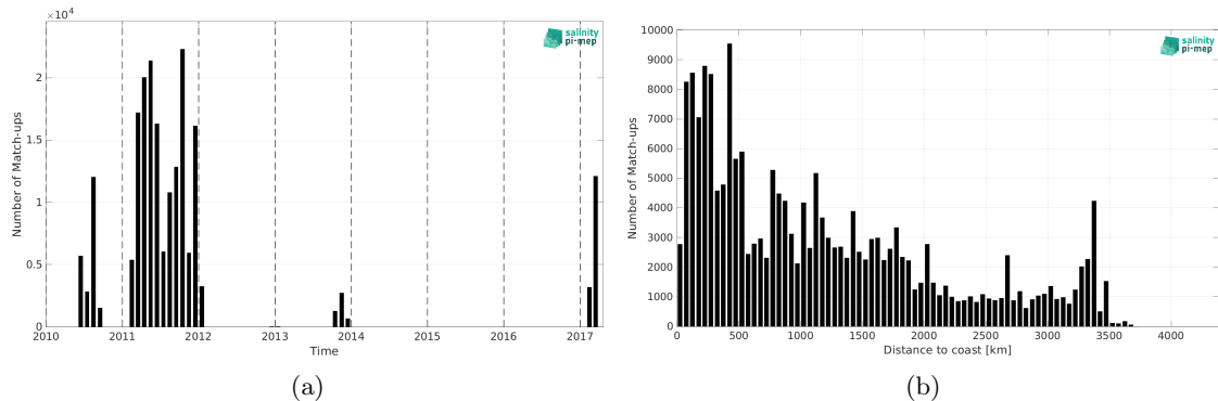
Figure 1: Number of match-ups between TSG (GOSUD-Sailing-ship) and CCI SSS L4 Merged-OI v4.4 - 7-day running (ESA) SSS as a function of time (a) and as function of the distance to coast (b) over the Pacific Ocean Pi-MEP region and for the full satellite product period.
