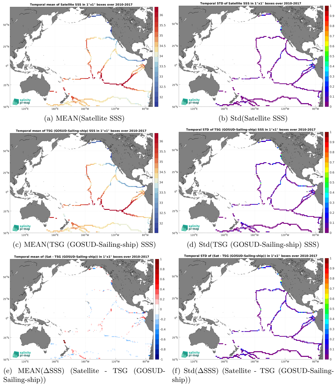
Figure 6: Temporal mean (left) and Std (right) of SSS from CCI SSS L4 Merged-OI v4.4 - 7-day running (ESA) (top), TSG (GOSUD-Sailing-ship) (middle), and of \Delta SSS (Satellite - TSG (GOSUD-Sailing-ship)). Only match-up pairs are used to generate these maps.
