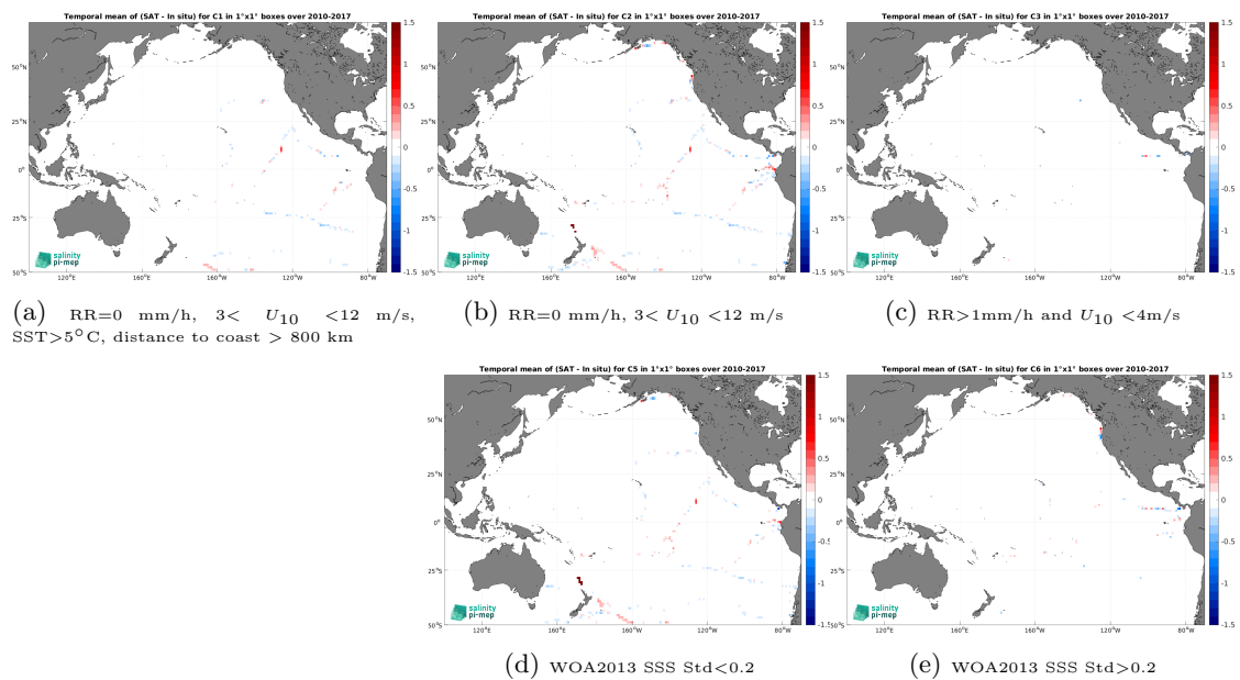
Figure 12: Temporal mean gridded over spatial boxes of size 1^\circ \times 1^\circ of \Delta\text{SSS} (CCI SSS L4 Merged-OI v4.4 - 7-day running (ESA) - TSG (GOSUD-Sailing-ship)) for 5 different subdatasets corresponding to:RR=0 mm/h, 3 < U_{10} < 12 m/s, SST >5^\circ\text{C} , distance to coast > 800 km (a), RR=0 mm/h, 3 < U_{10} < 12 m/s (b), RR >1 mm/h and U_{10} < 4 m/s (c), WOA2013 SSS Std <0.2 (d), WOA2013 SSS Std >0.2 (e).
