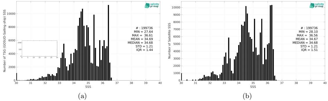
Figure 2: Histograms of SSS from TSG (GOSUD-Sailing-ship) (a) and CCI SSS L4 Merged-OI v4.4 - 7-day running (ESA) (b) considering all match-up pairs per bins of 0.1 over the Pacific Ocean Pi-MEP region and for the full satellite product period.
