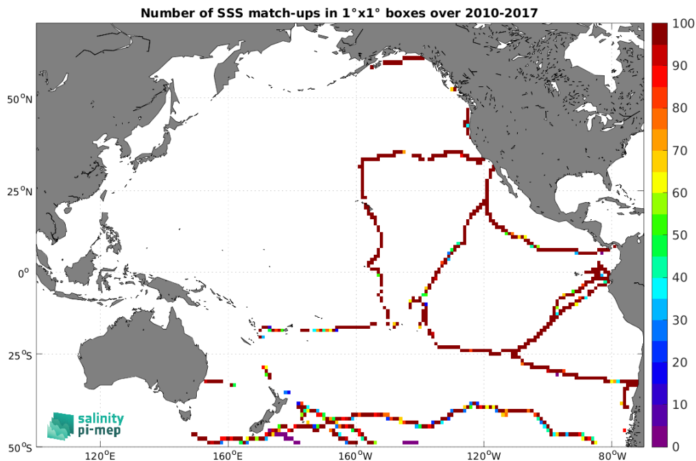
Figure 4: Number of SSS match-ups between TSG (GOSUD-Sailing-ship) SSS and the CCI SSS L4 Merged-OI v4.4 - 7-day running (ESA) SSS product for the Pacific Ocean Pi-MEP region over 1^\circ \times 1^\circ boxes and for the full satellite product period.
