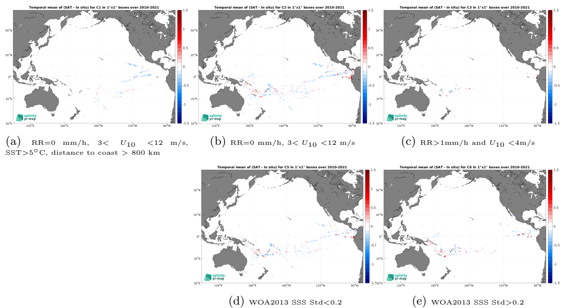
Figure 12: Temporal mean gridded over spatial boxes of size 1^\circ \times 1^\circ of \Delta SSS (CCI SSS L4 Merged-OI v4.4 - 7-day running (ESA) - TSG (GOSUD-Research-vessel)) for 5 different subdatasets corresponding to:RR=0 mm/h, 3 < U_{10} < 12 m/s, SST > 5^\circ\text{C} , distance to coast > 800 km (a), RR=0 mm/h, 3 < U_{10} < 12 m/s (b), RR > 1 mm/h and U_{10} < 4 m/s (c), WOA2013 SSS Std < 0.2 (d), WOA2013 SSS Std > 0.2 (e).
