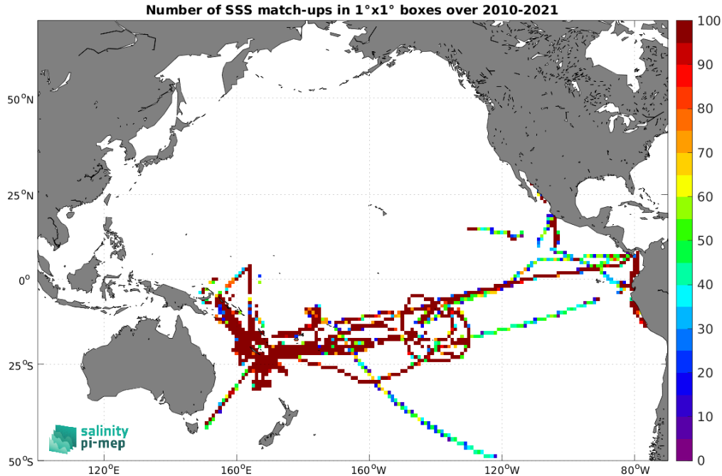
Figure 4: Number of SSS match-ups between TSG (GOSUD-Research-vessel) SSS and the CCI SSS L4 Merged-OI v4.4 - 7-day running (ESA) SSS product for the Pacific Ocean Pi-MEP region over 1^\circ \times 1^\circ boxes and for the full satellite product period.
