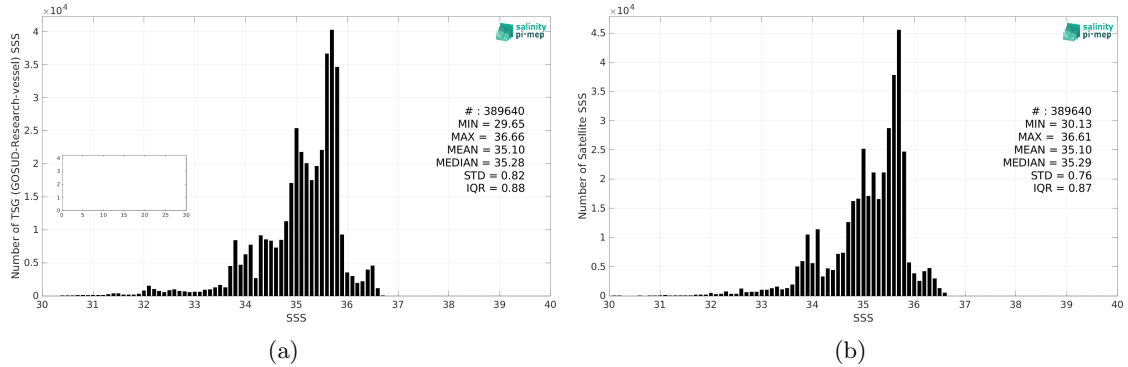
Figure 2: Histograms of SSS from TSG (GOSUD-Research-vessel) (a) and CCI SSS L4 Merged-OI v4.4 - 7-day running (ESA) (b) considering all match-up pairs per bins of 0.1 over the Pacific Ocean Pi-MEP region and for the full satellite product period.
