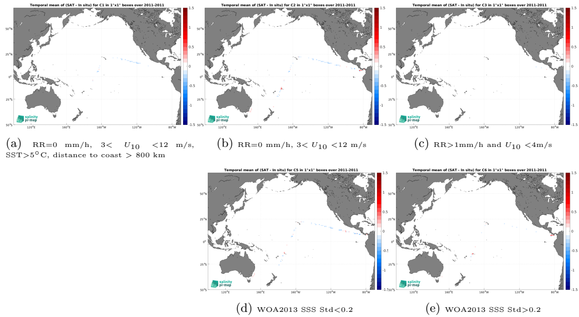
Figure 12: Temporal mean gridded over spatial boxes of size 1^\circ \times 1^\circ of \Delta SSS (CCI SSS L4 Merged-OI v4.4 - 7-day running (ESA) - TSG (CSIC-UTM)) for 5 different subdatasets corresponding to:RR=0 mm/h, 3 < U_{10} < 12 m/s, SST >5^\circ C, distance to coast > 800 km (a), RR=0 mm/h, 3 < U_{10} < 12 m/s (b), RR >1 mm/h and U_{10} < 4 m/s (c), WOA2013 SSS Std <0.2 (d), WOA2013 SSS Std >0.2 (e).
