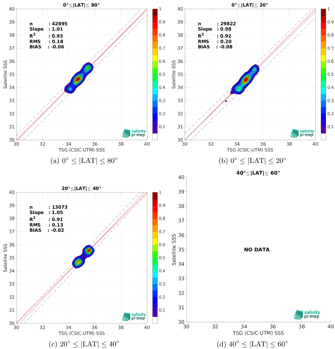
Figure 9: Contour maps of the concentration of CCI SSS L4 Merged-OI v4.4 - 7-day running (ESA) SSS (y-axis) versus TSG (CSIC-UTM) SSS (x-axis) at match-up pairs for different latitude bands. For each plot, the red line shows x=y . The black thin and dashed lines indicate a linear fit through the data cloud and the \pm 95\% confidence levels, respectively. The number match-up pairs n , the slope and R^2 coefficient of the linear fit, the root mean square (RMS) and the mean bias between satellite and in situ data are indicated for each latitude band in each plots.
