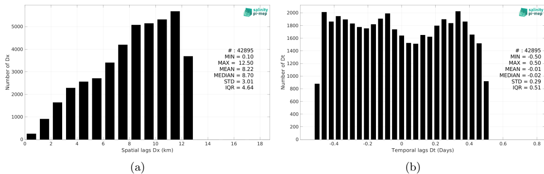
Figure 5: Histograms of the spatial (a) and temporal (b) lags between the location/time of the TSG (CSIC-UTM) measurement and the date of the corresponding CCI SSS L4 Merged-OI v4.4 - 7-day running (ESA) SSS pixel.
