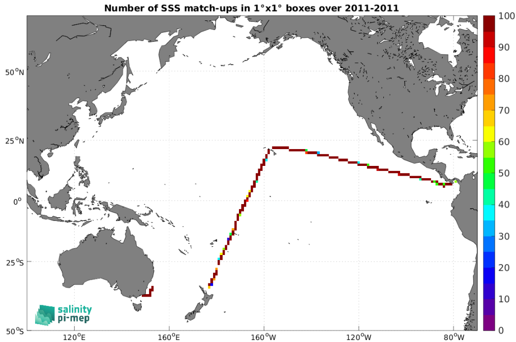
Figure 4: Number of SSS match-ups between TSG (CSIC-UTM) SSS and the CCI SSS L4 Merged-OI v4.4 - 7-day running (ESA) SSS product for the Pacific Ocean Pi-MEP region over 1^\circ \times 1^\circ boxes and for the full satellite product period.
