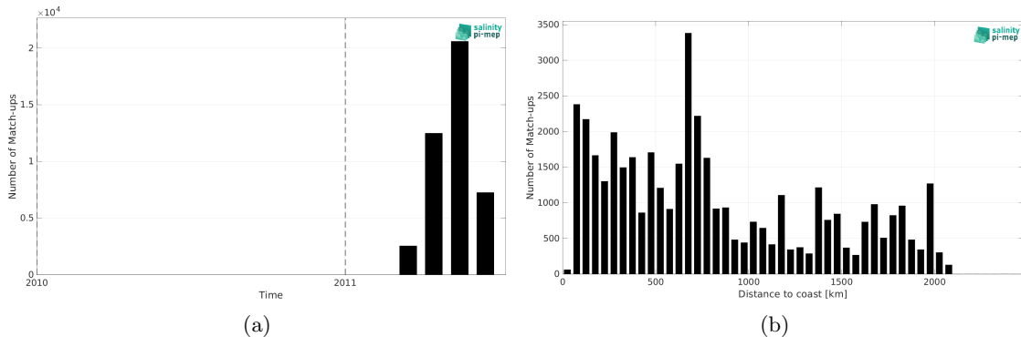
Figure 1: Number of match-ups between TSG (CSIC-UTM) and CCI SSS L4 Merged-OI v4.4 - 7-day running (ESA) SSS as a function of time (a) and as function of the distance to coast (b) over the Pacific Ocean Pi-MEP region and for the full satellite product period.
