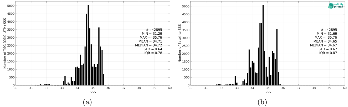
Figure 2: Histograms of SSS from TSG (CSIC-UTM) (a) and CCI SSS L4 Merged-OI v4.4 - 7-day running (ESA) (b) considering all match-up pairs per bins of 0.1 over the Pacific Ocean Pi-MEP region and for the full satellite product period.
