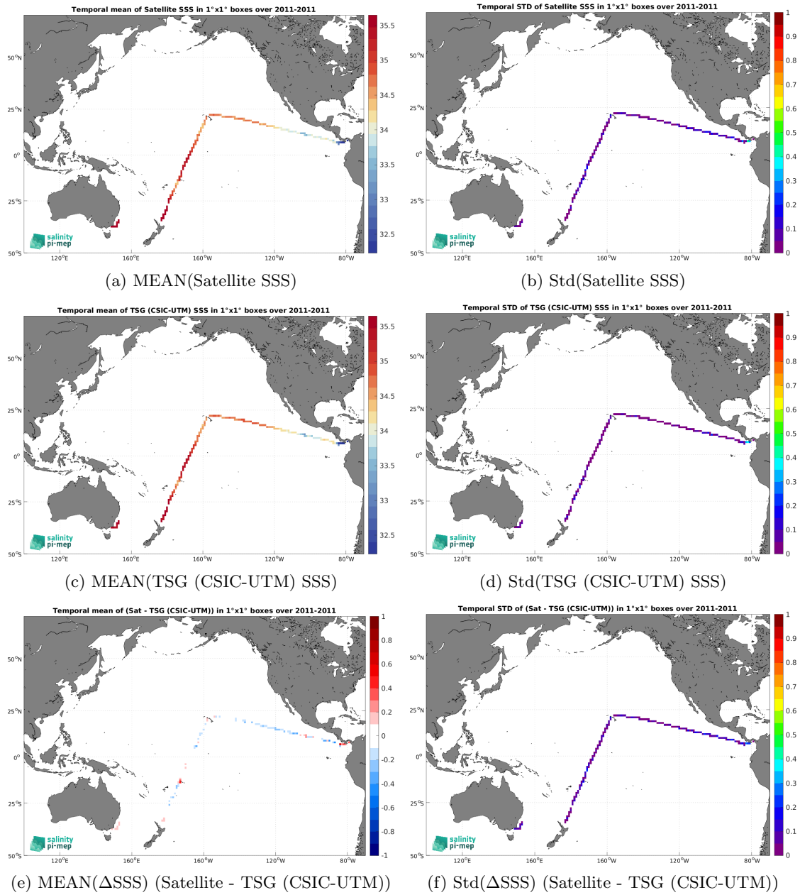
Figure 6: Temporal mean (left) and Std (right) of SSS from CCI SSS L4 Merged-OI v4.4 - 7-day running (ESA) (top), TSG (CSIC-UTM) (middle), and of \Delta SSS (Satellite - TSG (CSIC-UTM)). Only match-up pairs are used to generate these maps.
