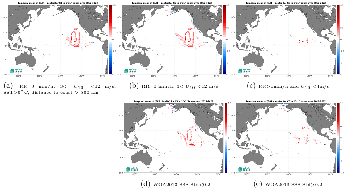
Figure 12: Temporal mean gridded over spatial boxes of size 1^\circ \times 1^\circ of \Delta SSS (CCI SSS L4 Merged-OI v4.4 - 7-day running (ESA) - Saildrone) for 5 different subdatasets corresponding to:RR=0 mm/h, 3 < U_{10} < 12 m/s, SST >5^\circ C, distance to coast > 800 km (a), RR=0 mm/h, 3 < U_{10} < 12 m/s (b), RR >1 mm/h and U_{10} < 4 m/s (c), WOA2013 SSS Std <0.2 (d), WOA2013 SSS Std >0.2 (e).
