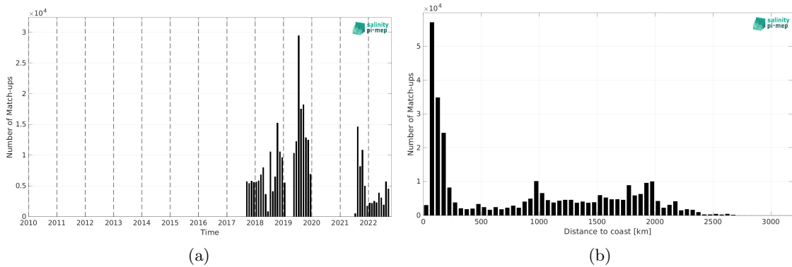
Figure 1: Number of match-ups between Saildrone and CCI SSS L4 Merged-OI v4.4 - 7-day running (ESA) SSS as a function of time (a) and as function of the distance to coast (b) over the Pacific Ocean Pi-MEP region and for the full satellite product period.
