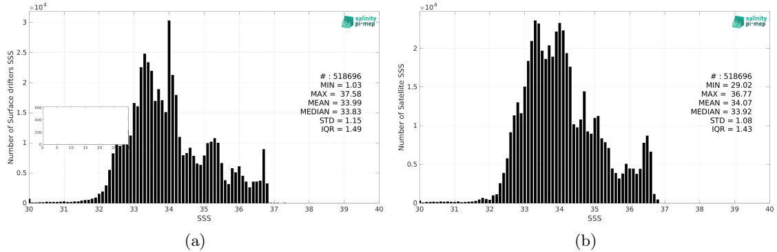
Figure 2: Histograms of SSS from Surface drifters (a) and CCI SSS L4 Merged-OI v4.4 - 7-day running (ESA) (b) considering all match-up pairs per bins of 0.1 over the Pacific Ocean Pi-MEP region and for the full satellite product period.
