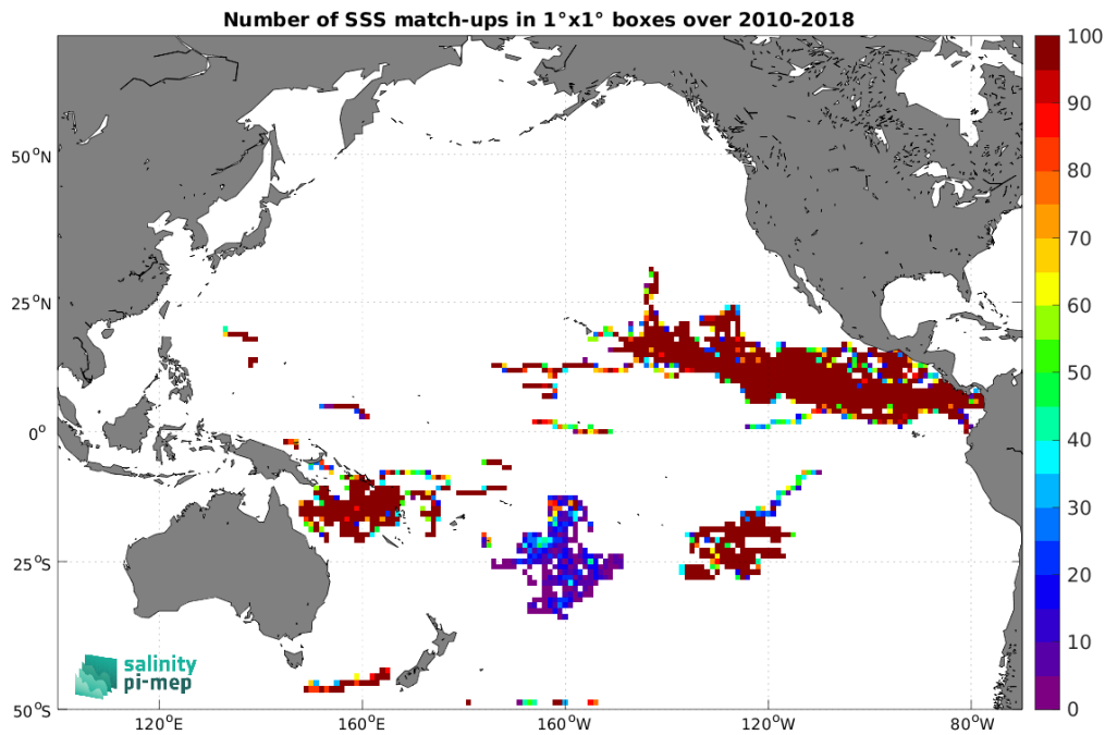
Figure 3: Number of SSS match-ups between Surface drifters SSS and the CCI SSS L4 Merged-OI v4.4 - 7-day running (ESA) SSS product for the Pacific Ocean Pi-MEP region over 1^\circ \times 1^\circ boxes and for the full satellite product period.
