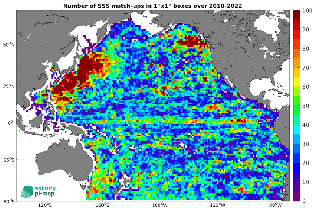
Figure 4: Number of SSS match-ups between Argo SSS and the CCI SSS L4 Merged-OI v4.4 - 7-day running (ESA) SSS product for the Pacific Ocean Pi-MEP region over 1^\circ \times 1^\circ boxes and for the full satellite product period.
