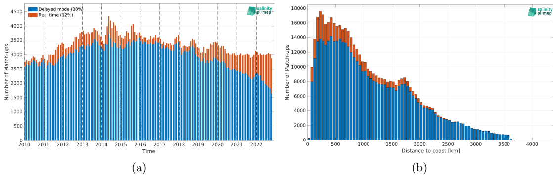
Figure 1: Number of match-ups between Argo and CCI SSS L4 Merged-OI v4.4 - 7-day running (ESA) SSS as a function of time (a) and as function of the distance to coast (b) over the Pacific Ocean Pi-MEP region and for the full satellite product period.
