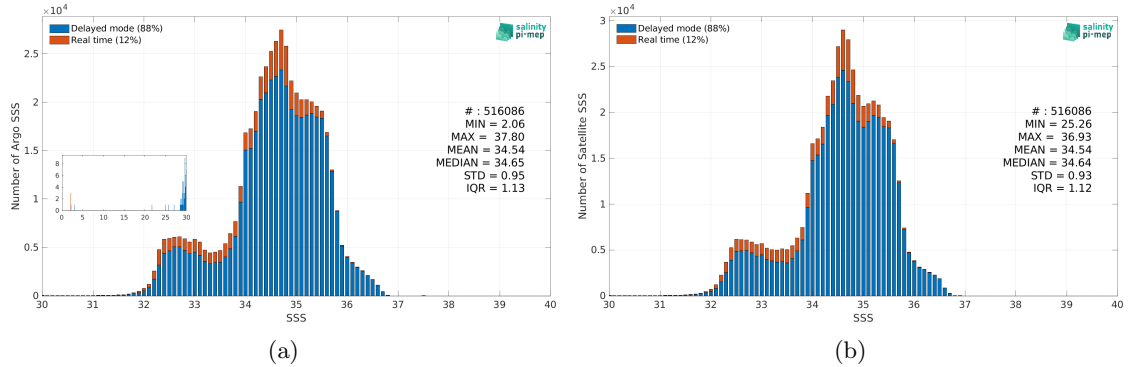
Figure 2: Histograms of SSS from Argo (a) and CCI SSS L4 Merged-OI v4.4 - 7-day running (ESA) (b) considering all match-up pairs per bins of 0.1 over the Pacific Ocean Pi-MEP region and for the full satellite product period.
