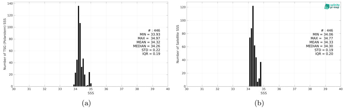
Figure 2: Histograms of SSS from TSG (Polarstern) (a) and CCI SSS L4 Merged-OI v4.4 - 30-day running (ESA) (b) considering all match-up pairs per bins of 0.1 over the Pacific Ocean Pi-MEP region and for the full satellite product period.
