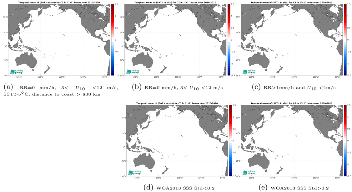
Figure 12: Temporal mean gridded over spatial boxes of size 1^{\circ}\times 1^{\circ} of \Delta\text{SSS} (CCI SSS L4 Merged-OI v4.4 - 30-day running (ESA) - TSG (Polarstern)) for 5 different subdatasets corresponding to:RR=0 mm/h, 3 < U_{10} < 12 m/s, SST >5^{\circ}\text{C} , distance to coast > 800 km (a), RR=0 mm/h, 3 < U_{10} < 12 m/s (b), RR >1 mm/h and U_{10} < 4 m/s (c), WOA2013 SSS Std <0.2 (d), WOA2013 SSS Std >0.2 (e).
