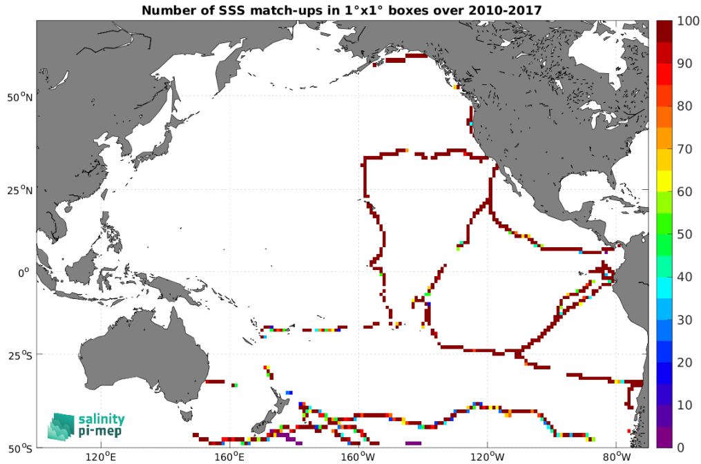
Figure 4: Number of SSS match-ups between TSG (GOSUD-Sailing-ship) SSS and the CCI SSS L4 Merged-OI v4.4 - 30-day running (ESA) SSS product for the Pacific Ocean Pi-MEP region over 1^\circ \times 1^\circ boxes and for the full satellite product period.
