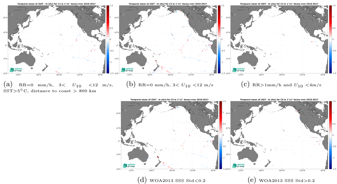
Figure 12: Temporal mean gridded over spatial boxes of size 1^\circ \times 1^\circ of \Delta SSS (CCI SSS L4 Merged-OI v4.4 - 30-day running (ESA) - TSG (GOSUD-Sailing-ship)) for 5 different subdatasets corresponding to:RR=0 mm/h, 3 < U_{10} < 12 m/s, SST >5^\circ\text{C} , distance to coast > 800 km (a), RR=0 mm/h, 3 < U_{10} < 12 m/s (b), RR >1 mm/h and U_{10} < 4 m/s (c), WOA2013 SSS Std <0.2 (d), WOA2013 SSS Std >0.2 (e).
