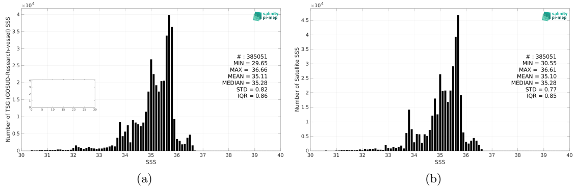
Figure 2: Histograms of SSS from TSG (GOSUD-Research-vessel) (a) and CCI SSS L4 Merged-OI v4.4 - 30-day running (ESA) (b) considering all match-up pairs per bins of 0.1 over the Pacific Ocean Pi-MEP region and for the full satellite product period.
