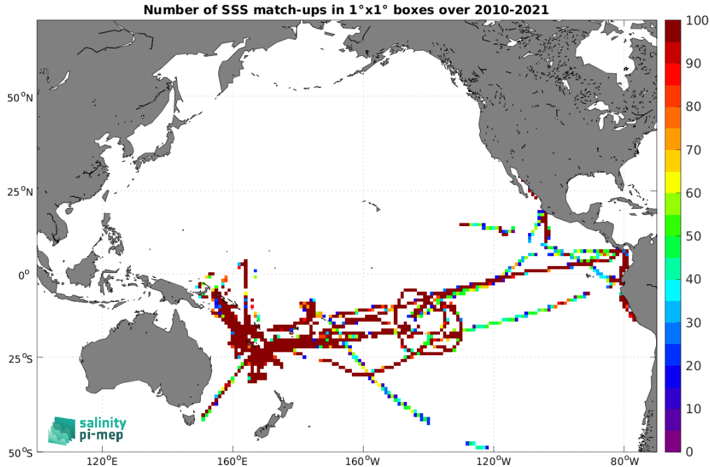
Figure 4: Number of SSS match-ups between TSG (GOSUD-Research-vessel) SSS and the CCI SSS L4 Merged-OI v4.4 - 30-day running (ESA) SSS product for the Pacific Ocean Pi-MEP region over 1^\circ \times 1^\circ boxes and for the full satellite product period.
