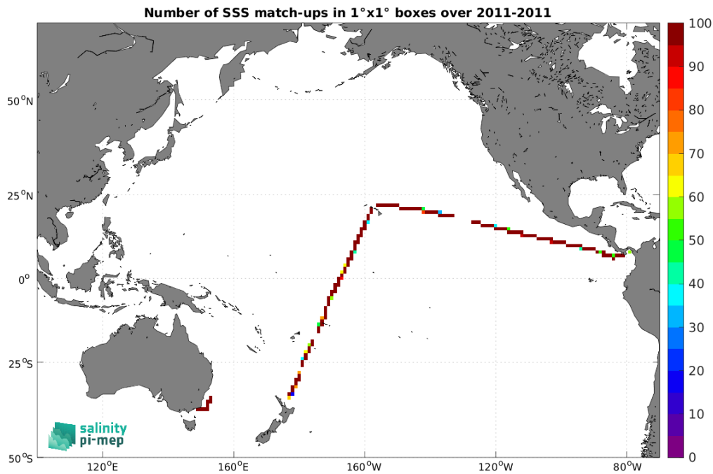
Figure 4: Number of SSS match-ups between TSG (CSIC-UTM) SSS and the CCI SSS L4 Merged-OI v4.4 - 30-day running (ESA) SSS product for the Pacific Ocean Pi-MEP region over 1^\circ \times 1^\circ boxes and for the full satellite product period.
