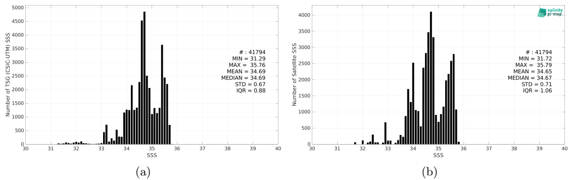
Figure 2: Histograms of SSS from TSG (CSIC-UTM) (a) and CCI SSS L4 Merged-OI v4.4 - 30-day running (ESA) (b) considering all match-up pairs per bins of 0.1 over the Pacific Ocean Pi-MEP region and for the full satellite product period.
