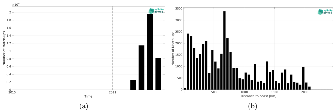
Figure 1: Number of match-ups between TSG (CSIC-UTM) and CCI SSS L4 Merged-OI v4.4 - 30-day running (ESA) SSS as a function of time (a) and as function of the distance to coast (b) over the Pacific Ocean Pi-MEP region and for the full satellite product period.
