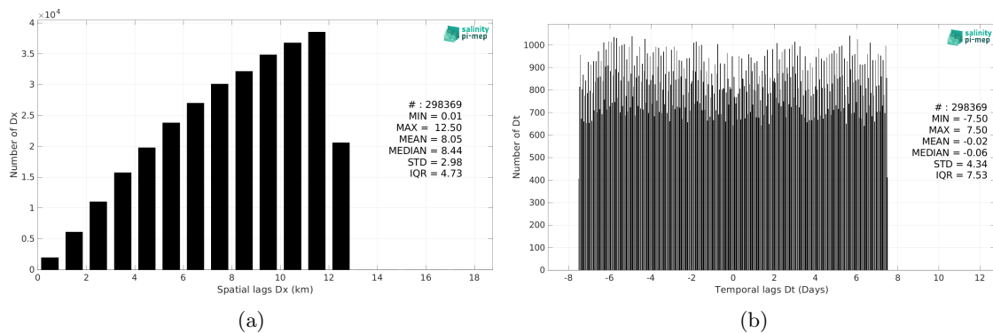
Figure 5: Histograms of the spatial (a) and temporal (b) lags between the location/time of the Saildrone measurement and the date of the corresponding CCI SSS L4 Merged-OI v4.4 - 30-day running (ESA) SSS pixel.
