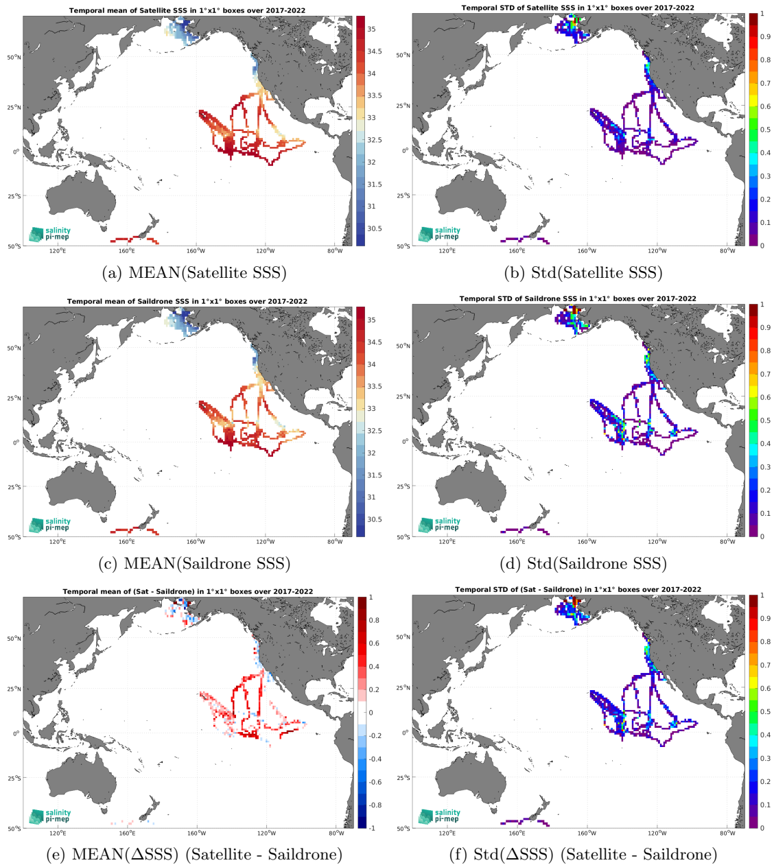
Figure 6: Temporal mean (left) and Std (right) of SSS from CCI SSS L4 Merged-OI v4.4 - 30-day running (ESA) (top), Saildrone (middle), and of \Delta SSS (Satellite - Saildrone). Only match-up pairs are used to generate these maps.
