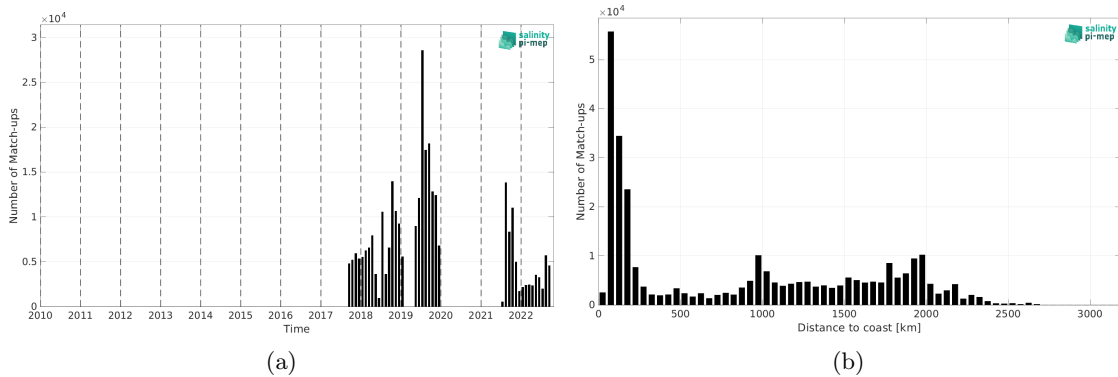
Figure 1: Number of match-ups between Saildrone and CCI SSS L4 Merged-OI v4.4 - 30-day running (ESA) SSS as a function of time (a) and as function of the distance to coast (b) over the Pacific Ocean Pi-MEP region and for the full satellite product period.
