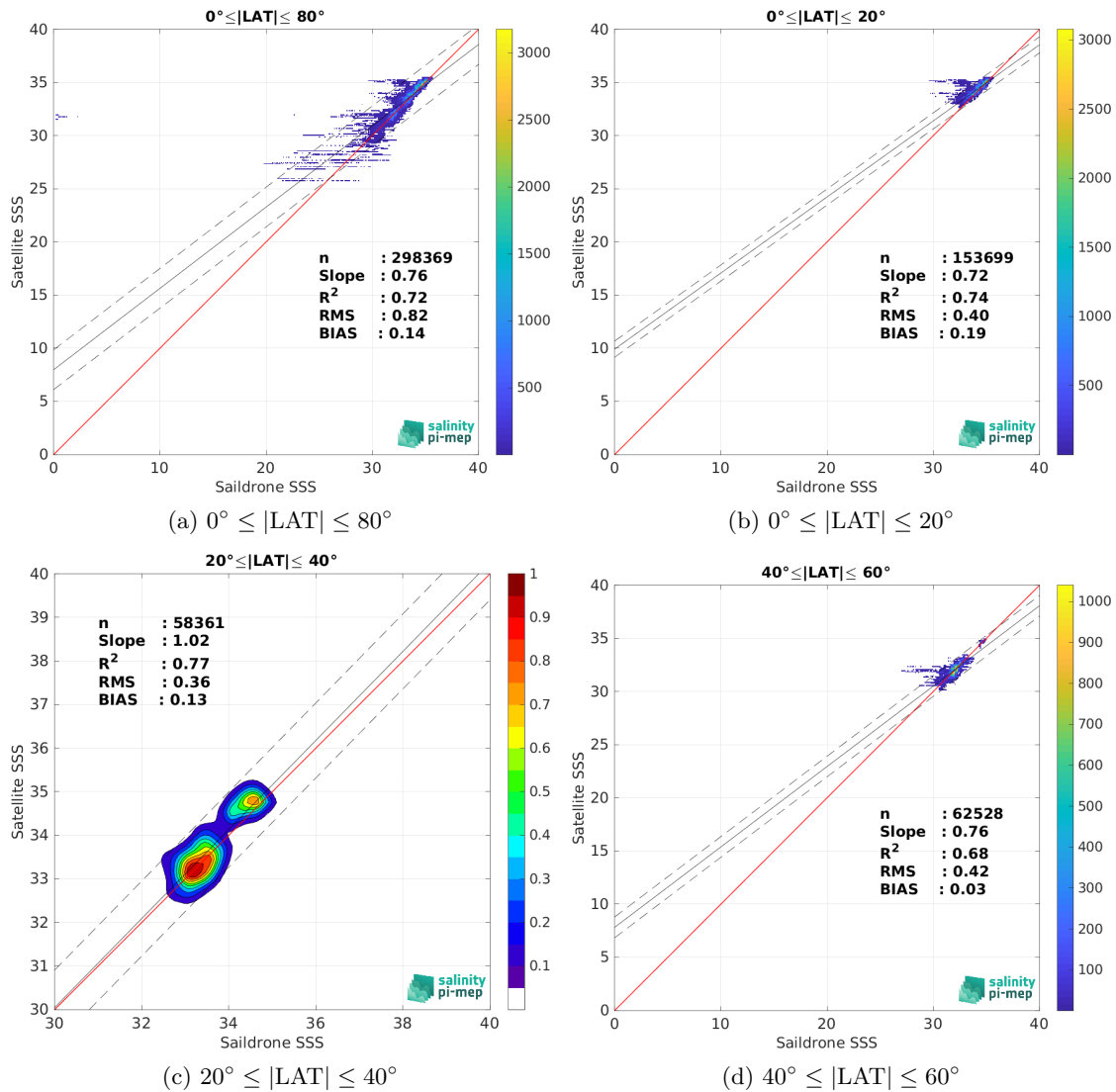
Figure 9: Contour maps of the concentration of CCI SSS L4 Merged-OI v4.4 - 30-day running (ESA) SSS (y-axis) versus Saildrone SSS (x-axis) at match-up pairs for different latitude bands. For each plot, the red line shows x=y . The black thin and dashed lines indicate a linear fit through the data cloud and the \pm 95\% confidence levels, respectively. The number match-up pairs n , the slope and R^2 coefficient of the linear fit, the root mean square (RMS) and the mean bias between satellite and in situ data are indicated for each latitude band in each plots.
