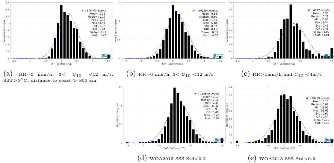
Figure 13: Normalized histogram of \Delta\text{SSS} (CCI SSS L4 Merged-OI v4.4 - 30-day running (ESA) - Saildrone) for 5 different subdatasets corresponding to: RR=0 mm/h, 3 < U_{10} < 12 m/s, SST>5°C, distance to coast > 800 km (a), RR=0 mm/h, 3 < U_{10} < 12 m/s (b), RR>1mm/h and U_{10} < 4 m/s (c), WOA2013 SSS Std<0.2 (d), WOA2013 SSS Std>0.2 (e).
