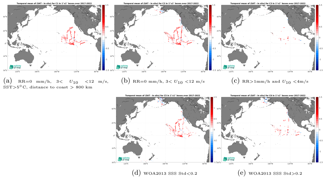
Figure 12: Temporal mean gridded over spatial boxes of size 1^\circ \times 1^\circ of \Delta SSS (CCI SSS L4 Merged-OI v4.4 - 30-day running (ESA) - Saildrone) for 5 different subdatasets corresponding to:RR=0 mm/h, 3 < U_{10} < 12 m/s, SST >5^\circ C, distance to coast > 800 km (a), RR=0 mm/h, 3 < U_{10} < 12 m/s (b), RR >1 mm/h and U_{10} < 4 m/s (c), WOA2013 SSS Std <0.2 (d), WOA2013 SSS Std >0.2 (e).
