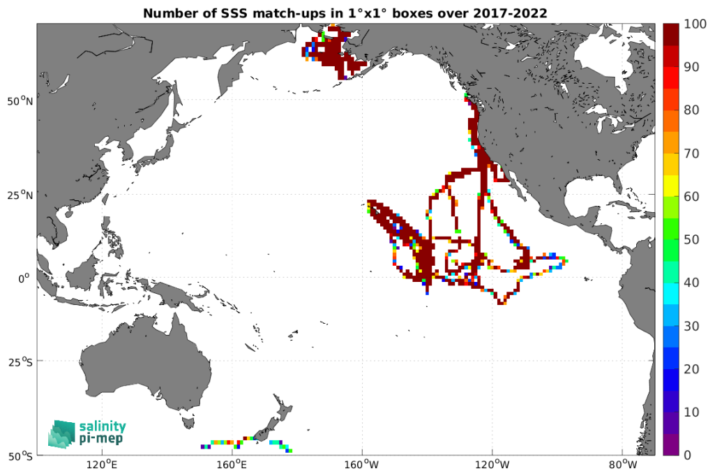
Figure 4: Number of SSS match-ups between Saildrone SSS and the CCI SSS L4 Merged-OI v4.4 - 30-day running (ESA) SSS product for the Pacific Ocean Pi-MEP region over 1^\circ \times 1^\circ boxes and for the full satellite product period.
