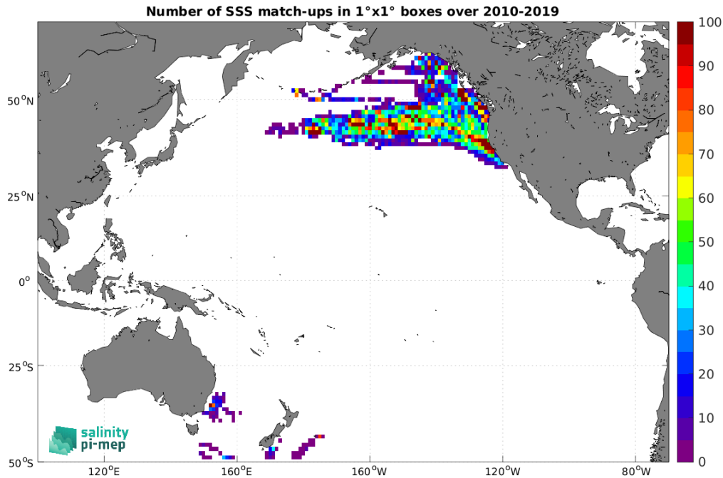
Figure 4: Number of SSS match-ups between Marine mammals SSS and the CCI SSS L4 Merged-OI v4.4 - 30-day running (ESA) SSS product for the Pacific Ocean Pi-MEP region over 1^\circ \times 1^\circ boxes and for the full satellite product period.
