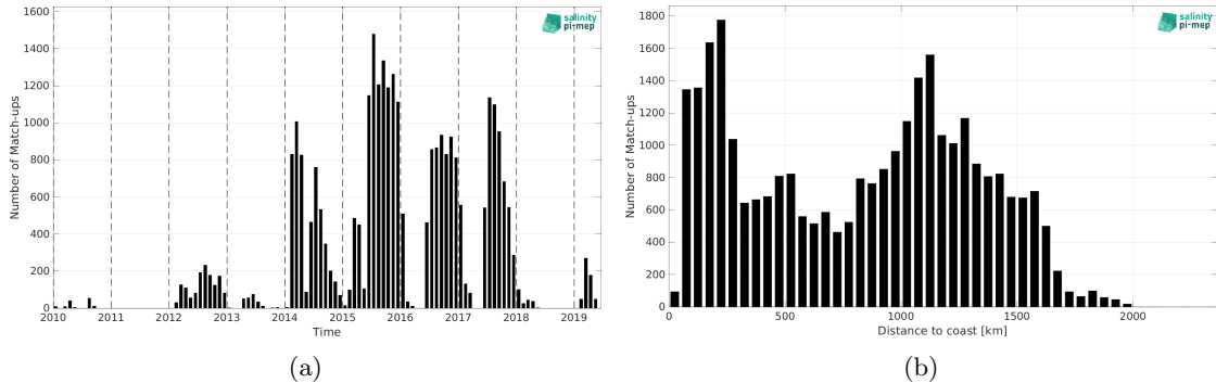
Figure 1: Number of match-ups between Marine mammals and CCI SSS L4 Merged-OI v4.4 - 30-day running (ESA) SSS as a function of time (a) and as function of the distance to coast (b) over the Pacific Ocean Pi-MEP region and for the full satellite product period.
