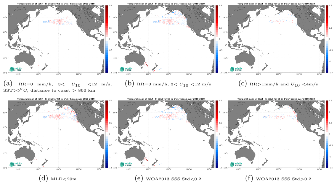
Figure 12: Temporal mean gridded over spatial boxes of size 1^\circ \times 1^\circ of \Delta SSS (CCI SSS L4 Merged-OI v4.4 - 30-day running (ESA) - Marine mammals) for 6 different subdatasets corresponding to:RR=0 mm/h, 3 < U_{10} < 12 m/s, SST > 5^\circ C, distance to coast > 800 km (a), RR=0 mm/h, 3 < U_{10} < 12 m/s (b), RR > 1 mm/h and U_{10} < 4 m/s (c),MLD < 20 m (d),WOA2013 SSS Std < 0.2 (e),WOA2013 SSS Std > 0.2 (f).
