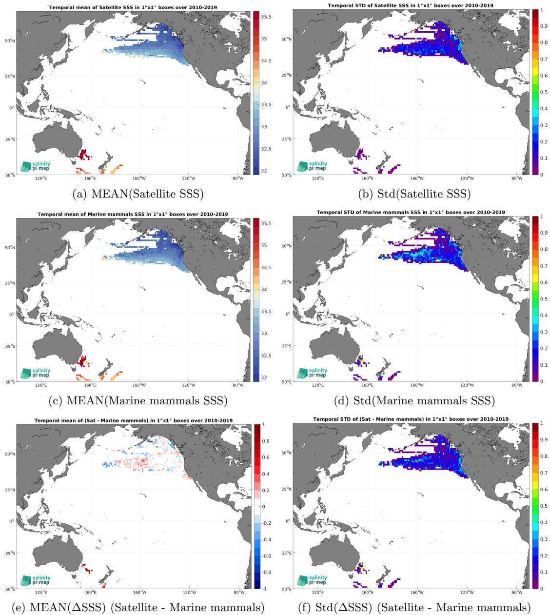
Figure 6: Temporal mean (left) and Std (right) of SSS from CCI SSS L4 Merged-OI v4.4 - 30-day running (ESA) (top), Marine mammals (middle), and of \Delta SSS (Satellite - Marine mammals). Only match-up pairs are used to generate these maps.
