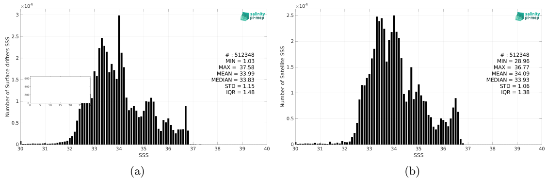
Figure 2: Histograms of SSS from Surface drifters (a) and CCI SSS L4 Merged-OI v4.4 - 30-day running (ESA) (b) considering all match-up pairs per bins of 0.1 over the Pacific Ocean Pi-MEP region and for the full satellite product period.
