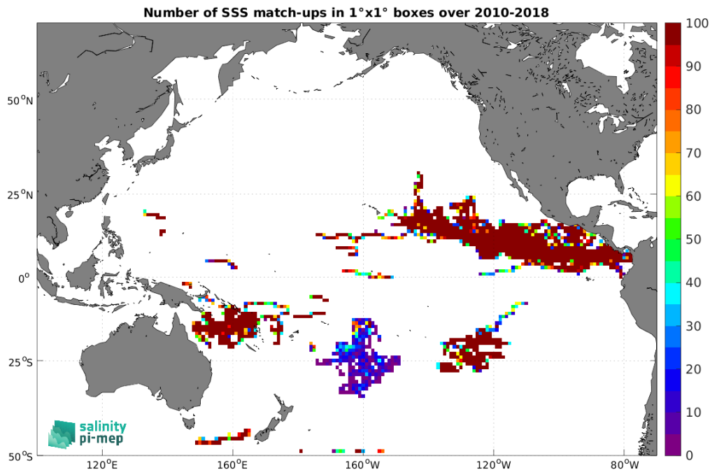
Figure 3: Number of SSS match-ups between Surface drifters SSS and the CCI SSS L4 Merged-OI v4.4 - 30-day running (ESA) SSS product for the Pacific Ocean Pi-MEP region over 1^\circ \times 1^\circ boxes and for the full satellite product period.
