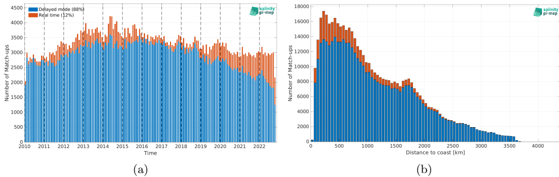
Figure 1: Number of match-ups between Argo and CCI SSS L4 Merged-OI v4.4 - 30-day running (ESA) SSS as a function of time (a) and as function of the distance to coast (b) over the Pacific Ocean Pi-MEP region and for the full satellite product period.
