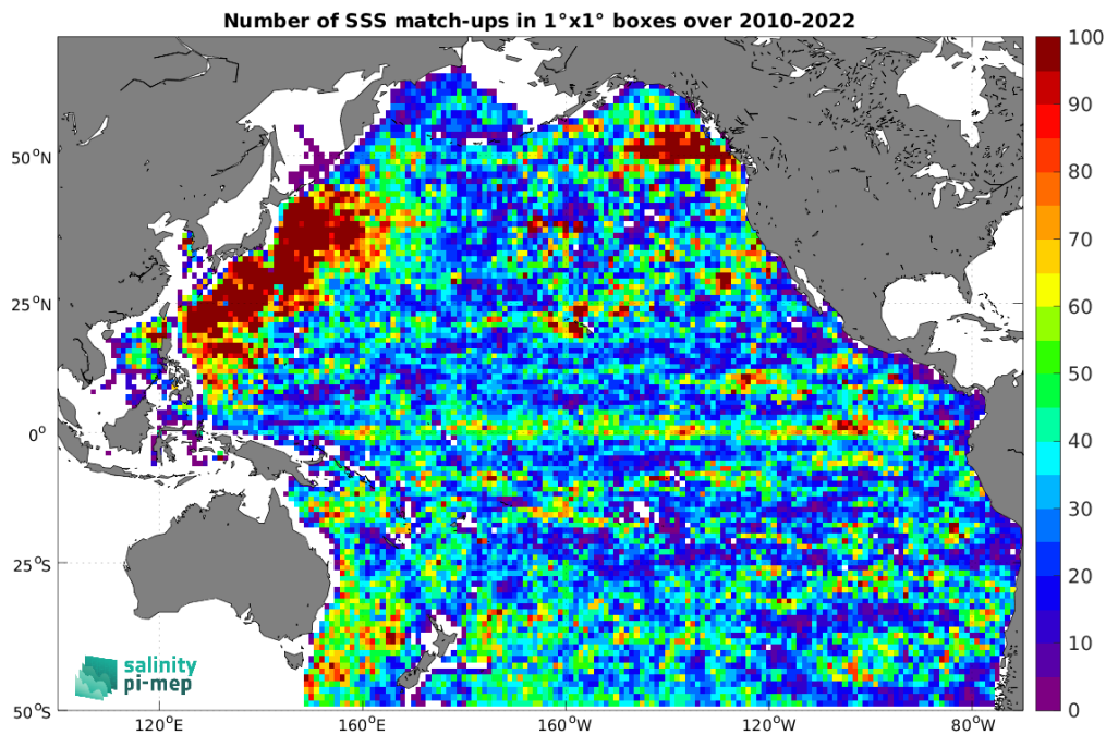
Figure 4: Number of SSS match-ups between Argo SSS and the CCI SSS L4 Merged-OI v4.4 - 30-day running (ESA) SSS product for the Pacific Ocean Pi-MEP region over 1^\circ \times 1^\circ boxes and for the full satellite product period.
