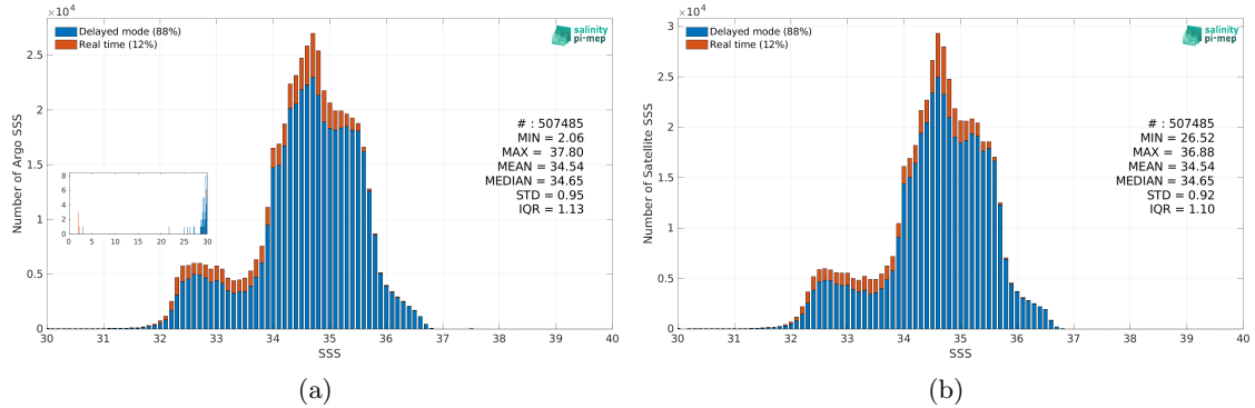
Figure 2: Histograms of SSS from Argo (a) and CCI SSS L4 Merged-OI v4.4 - 30-day running (ESA) (b) considering all match-up pairs per bins of 0.1 over the Pacific Ocean Pi-MEP region and for the full satellite product period.
