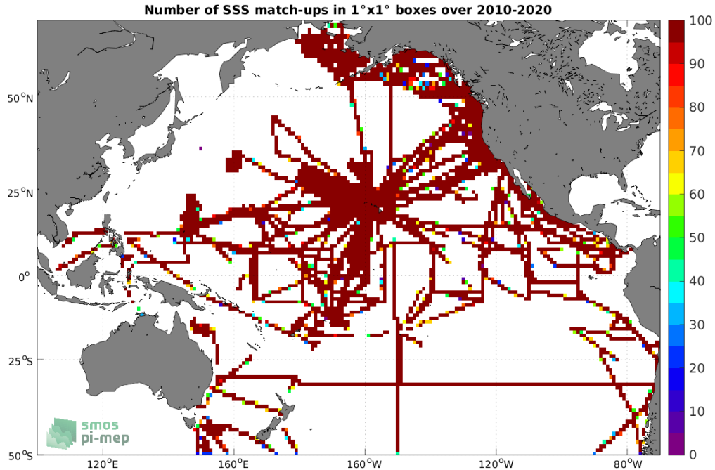
Figure 4: Number of SSS match-ups between TSG (SAMOS) SSS and the CCI SSS L4 Merged-OI v3.2 - 7-day running (ESA) SSS product for the Pacific Ocean Pi-MEP region over 1^\circ \times 1^\circ boxes and for the full satellite product period.
