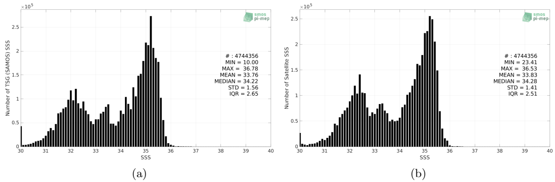
Figure 2: Histograms of SSS from TSG (SAMOS) (a) and CCI SSS L4 Merged-OI v3.2 - 7-day running (ESA) (b) considering all match-up pairs per bins of 0.1 over the Pacific Ocean Pi-MEP region and for the full satellite product period.
