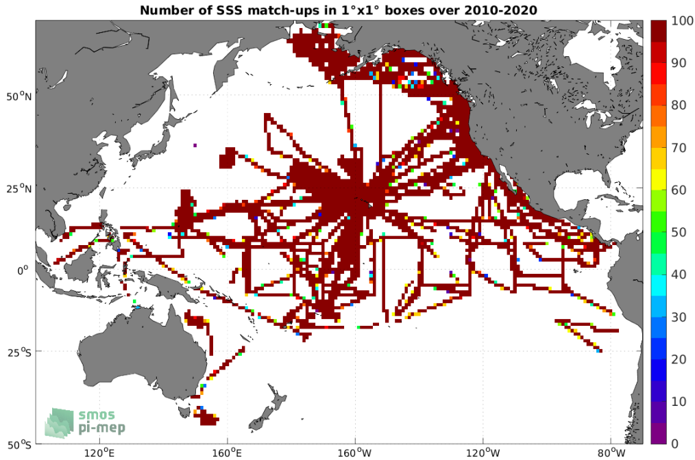
Figure 4: Number of SSS match-ups between TSG (SAMOS) SSS and the CCI SSS L4 Merged-OI v3.2 - 7-day running (ESA) SSS product for the Pacific Ocean Pi-MEP region over 1°x1° boxes and for the full satellite product period.
