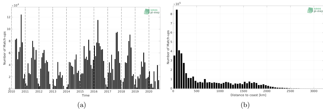
Figure 1: Number of match-ups between TSG (SAMOS) and CCI SSS L4 Merged-OI v3.2 - 7-day running (ESA) SSS as a function of time (a) and as function of the distance to coast (b) over the Pacific Ocean Pi-MEP region and for the full satellite product period.
