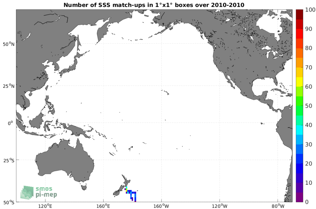
Figure 4: Number of SSS match-ups between TSG (Polarstern) SSS and the CCI SSS L4 Merged-OI v3.2 - 7-day running (ESA) SSS product for the Pacific Ocean Pi-MEP region over 1^\circ \times 1^\circ boxes and for the full satellite product period.
