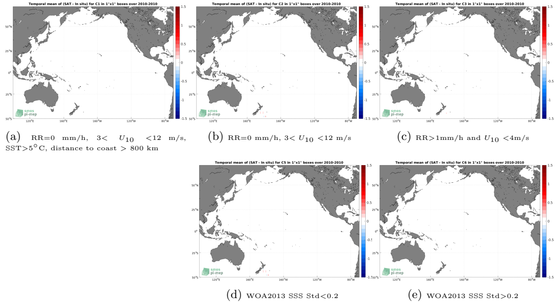
Figure 12: Temporal mean gridded over spatial boxes of size 1^{\circ}\times 1^{\circ} of \Delta\text{SSS} (CCI SSS L4 Merged-OI v3.2 - 7-day running (ESA) - TSG (Polarstern)) for 5 different subdatasets corresponding to:RR=0 mm/h, 3 < U_{10} < 12 m/s, SST >5^{\circ}\text{C} , distance to coast > 800 km (a), RR=0 mm/h, 3 < U_{10} < 12 m/s (b), RR >1 mm/h and U_{10} < 4 m/s (c), WOA2013 SSS Std <0.2 (d), WOA2013 SSS Std >0.2 (e).
