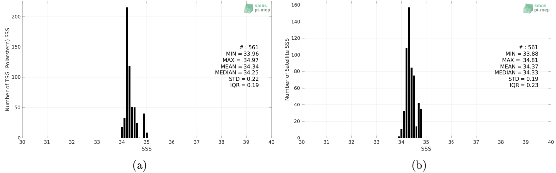
Figure 2: Histograms of SSS from TSG (Polarstern) (a) and CCI SSS L4 Merged-OI v3.2 - 7-day running (ESA) (b) considering all match-up pairs per bins of 0.1 over the Pacific Ocean Pi-MEP region and for the full satellite product period.
