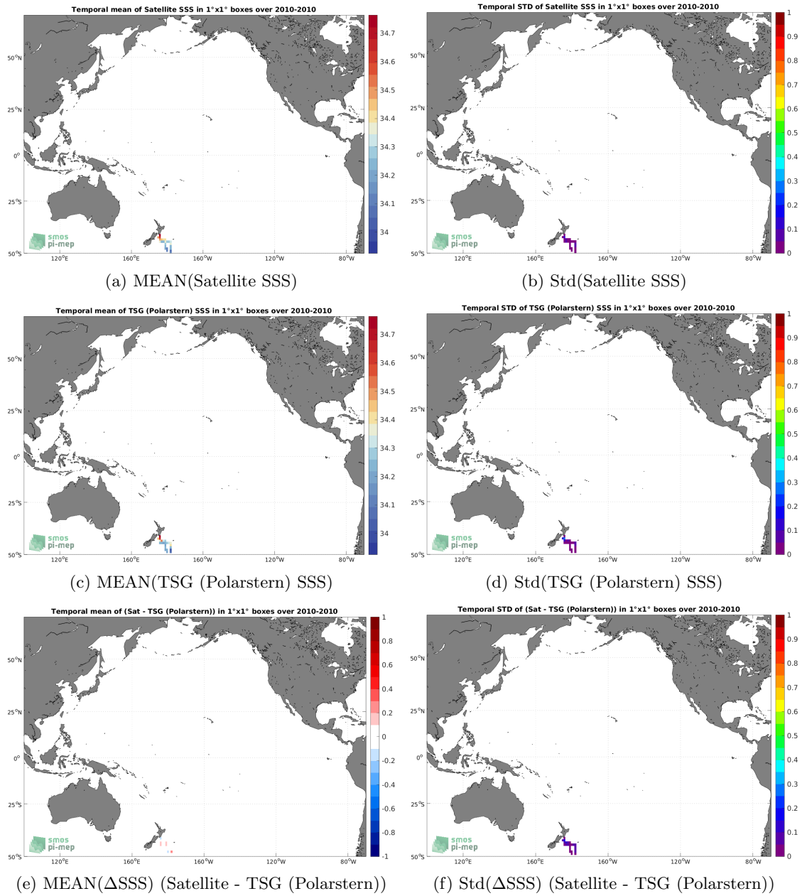
Figure 6: Temporal mean (left) and Std (right) of SSS from CCI SSS L4 Merged-OI v3.2 - 7-day running (ESA) (top), TSG (Polarstern) (middle), and of \Delta SSS (Satellite - TSG (Polarstern)). Only match-up pairs are used to generate these maps.
