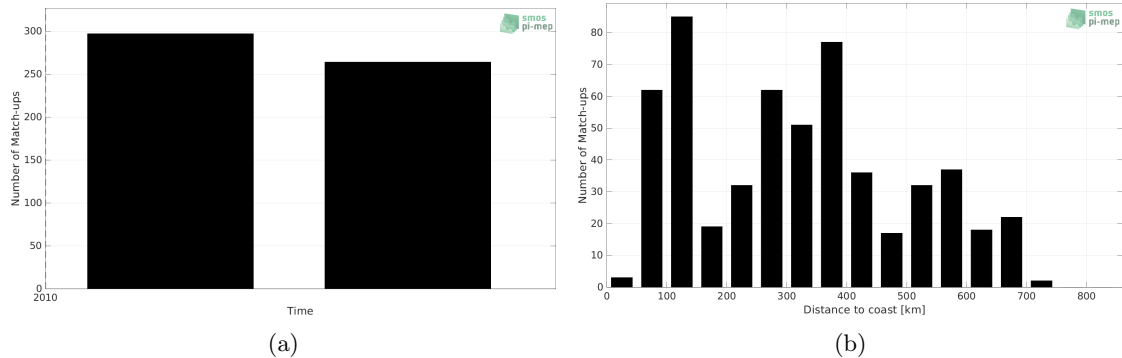
Figure 1: Number of match-ups between TSG (Polarstern) and CCI SSS L4 Merged-OI v3.2 - 7-day running (ESA) SSS as a function of time (a) and as function of the distance to coast (b) over the Pacific Ocean Pi-MEP region and for the full satellite product period.
