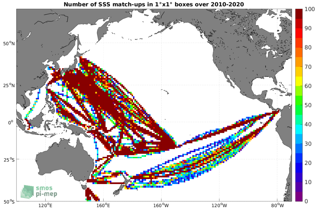
Figure 4: Number of SSS match-ups between TSG (LEGOS-DM) SSS and the CCI SSS L4 Merged-OI v3.2 - 7-day running (ESA) SSS product for the Pacific Ocean Pi-MEP region over 1^\circ \times 1^\circ boxes and for the full satellite product period.
