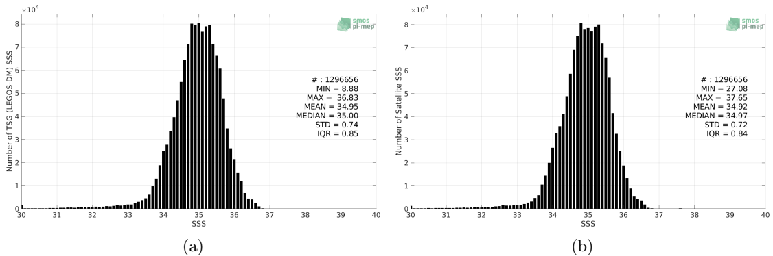
Figure 2: Histograms of SSS from TSG (LEGOS-DM) (a) and CCI SSS L4 Merged-OI v3.2 - 7-day running (ESA) (b) considering all match-up pairs per bins of 0.1 over the Pacific Ocean Pi-MEP region and for the full satellite product period.
