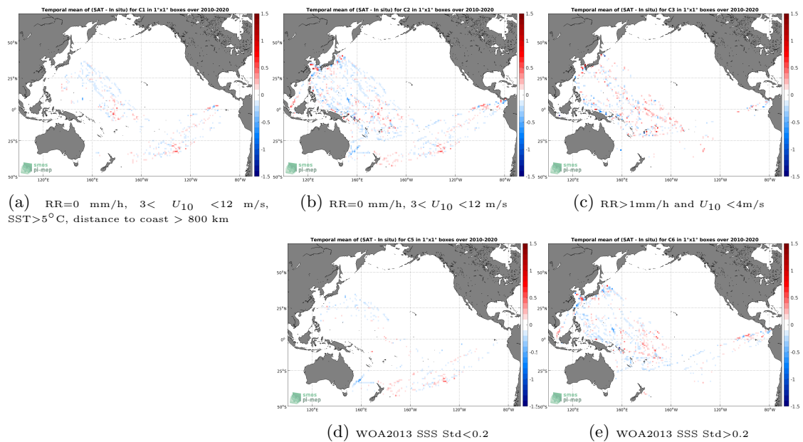
Figure 12: Temporal mean gridded over spatial boxes of size 1^\circ \times 1^\circ of \Delta SSS (CCI SSS L4 Merged-OI v3.2 - 7-day running (ESA) - TSG (LEGOS-DM)) for 5 different subdatasets corresponding to:RR=0 mm/h, 3 < U_{10} < 12 m/s, SST >5^\circ C, distance to coast > 800 km (a), RR=0 mm/h, 3 < U_{10} < 12 m/s (b), RR >1 mm/h and U_{10} < 4 m/s (c), WOA2013 SSS Std <0.2 (d), WOA2013 SSS Std >0.2 (e).
