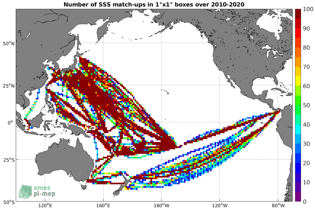
Figure 4: Number of SSS match-ups between TSG (LEGOS-DM) SSS and the CCI SSS L4 Merged-OI v3.2 - 7-day running (ESA) SSS product for the Pacific Ocean Pi-MEP region over 1°x1° boxes and for the full satellite product period.
