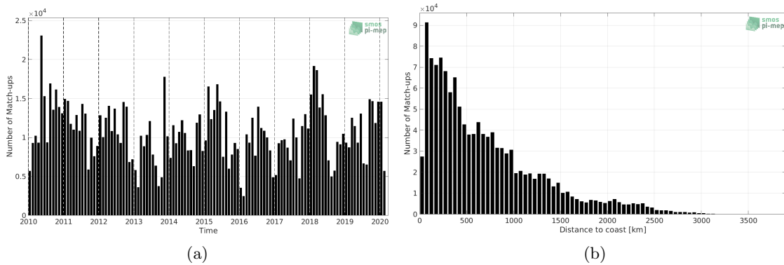
Figure 1: Number of match-ups between TSG (LEGOS-DM) and CCI SSS L4 Merged-OI v3.2 - 7-day running (ESA) SSS as a function of time (a) and as function of the distance to coast (b) over the Pacific Ocean Pi-MEP region and for the full satellite product period.
