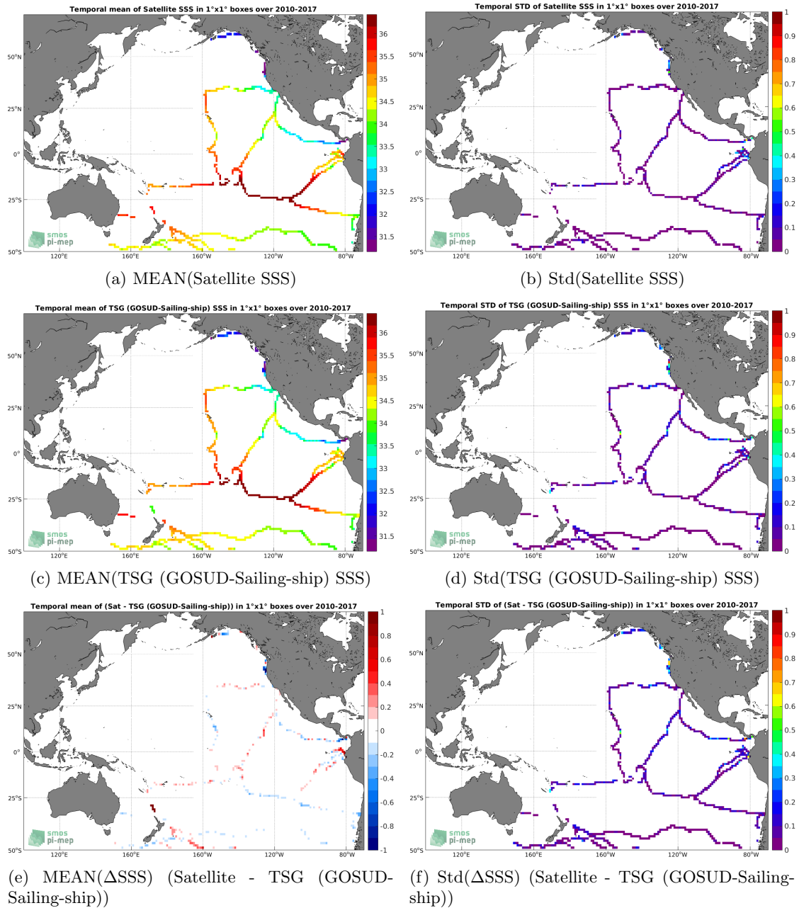
Figure 6: Temporal mean (left) and Std (right) of SSS from CCI SSS L4 Merged-OI v3.2 - 7-day running (ESA) (top), TSG (GOSUD-Sailing-ship) (middle), and of \Delta SSS (Satellite - TSG (GOSUD-Sailing-ship)). Only match-up pairs are used to generate these maps.
