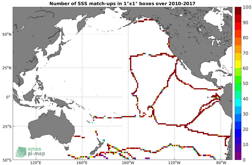
Figure 4: Number of SSS match-ups between TSG (GOSUD-Sailing-ship) SSS and the CCI SSS L4 Merged-OI v3.2 - 7-day running (ESA) SSS product for the Pacific Ocean Pi-MEP region over 1^\circ \times 1^\circ boxes and for the full satellite product period.
