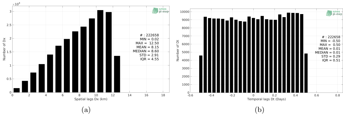
Figure 5: Histograms of the spatial (a) and temporal (b) lags between the location/time of the TSG (GOSUD-Sailing-ship) measurement and the date of the corresponding CCI SSS L4 Merged-OI v3.2 - 7-day running (ESA) SSS pixel.
