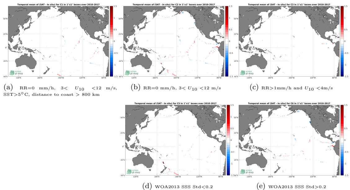
Figure 12: Temporal mean gridded over spatial boxes of size 1^\circ \times 1^\circ of \Delta SSS (CCI SSS L4 Merged-OI v3.2 - 7-day running (ESA) - TSG (GOSUD-Sailing-ship)) for 5 different subdatasets corresponding to: RR=0 mm/h, 3 < U_{10} < 12 m/s, SST > 5°C, distance to coast > 800 km (a), RR=0 mm/h, 3 < U_{10} < 12 m/s (b), RR > 1mm/h and U_{10} < 4 m/s (c), WOA2013 SSS Std < 0.2 (d), WOA2013 SSS Std > 0.2 (e).
