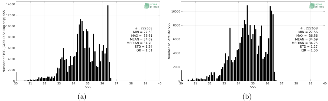
Figure 2: Histograms of SSS from TSG (GOSUD-Sailing-ship) (a) and CCI SSS L4 Merged-OI v3.2 - 7-day running (ESA) (b) considering all match-up pairs per bins of 0.1 over the Pacific Ocean Pi-MEP region and for the full satellite product period.
