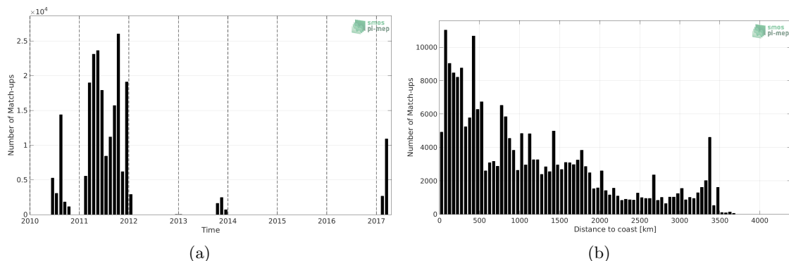
Figure 1: Number of match-ups between TSG (GOSUD-Sailing-ship) and CCI SSS L4 Merged-OI v3.2 - 7-day running (ESA) SSS as a function of time (a) and as function of the distance to coast (b) over the Pacific Ocean Pi-MEP region and for the full satellite product period.
