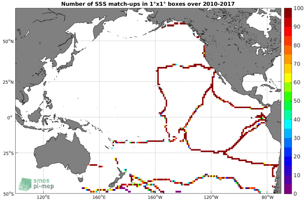
Figure 4: Number of SSS match-ups between TSG (GOSUD-Sailing-ship) SSS and the CCI SSS L4 Merged-OI v3.2 - 7-day running (ESA) SSS product for the Pacific Ocean Pi-MEP region over 1°x1° boxes and for the full satellite product period.
