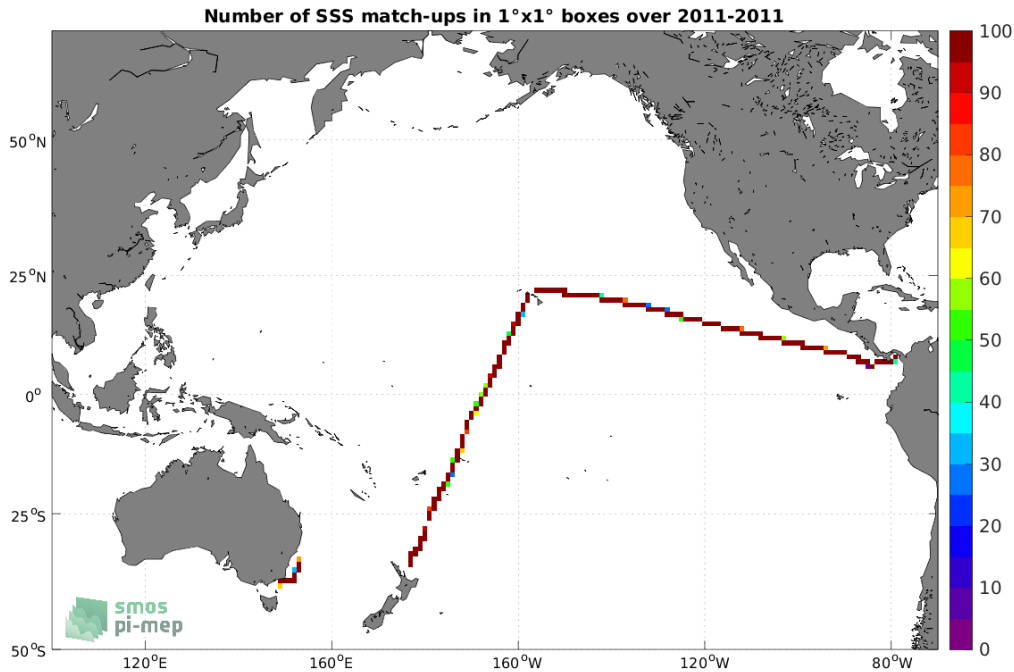
Figure 4: Number of SSS match-ups between TSG (CSIC-UTM) SSS and the CCI SSS L4 Merged-OI v3.2 - 7-day running (ESA) SSS product for the Pacific Ocean Pi-MEP region over 1^\circ \times 1^\circ boxes and for the full satellite product period.
