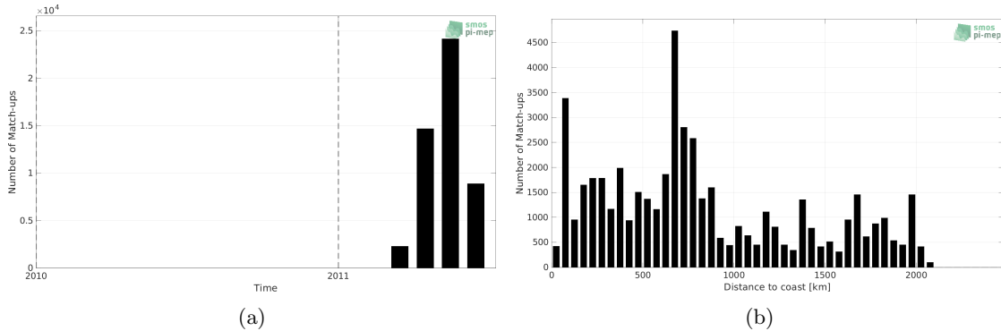
Figure 1: Number of match-ups between TSG (CSIC-UTM) and CCI SSS L4 Merged-OI v3.2 - 7-day running (ESA) SSS as a function of time (a) and as function of the distance to coast (b) over the Pacific Ocean Pi-MEP region and for the full satellite product period.
