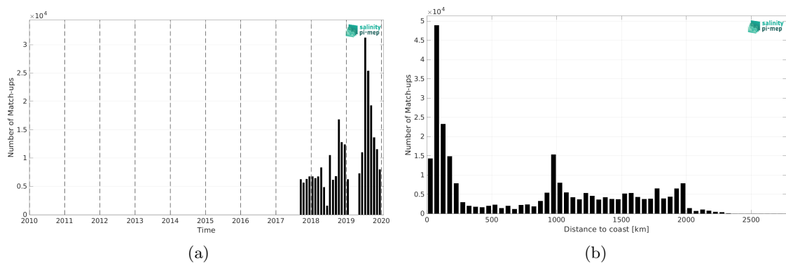
Figure 1: Number of match-ups between Sailability and CCI SSS L4 Merged-OI v3.2 - 7-day running (ESA) SSS as a function of time (a) and as function of the distance to coast (b) over the Pacific Ocean Pi-MEP region and for the full satellite product period.
