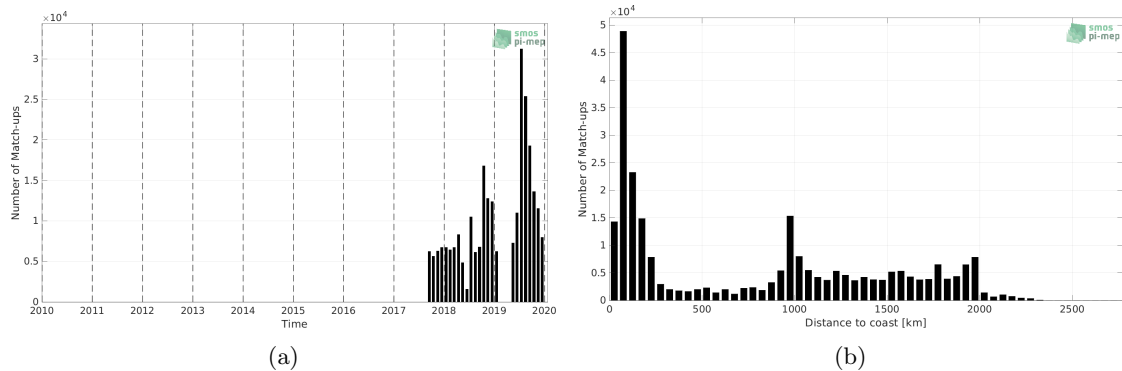
Figure 1: Number of match-ups between Saildrone and CCI SSS L4 Merged-OI v3.2 - 7-day running (ESA) SSS as a function of time (a) and as function of the distance to coast (b) over the Pacific Ocean Pi-MEP region and for the full satellite product period.
