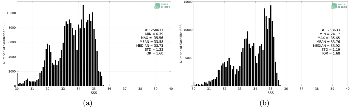
Figure 2: Histograms of SSS from Saildrone (a) and CCI SSS L4 Merged-OI v3.2 - 7-day running (ESA) (b) considering all match-up pairs per bins of 0.1 over the Pacific Ocean Pi-MEP region and for the full satellite product period.
