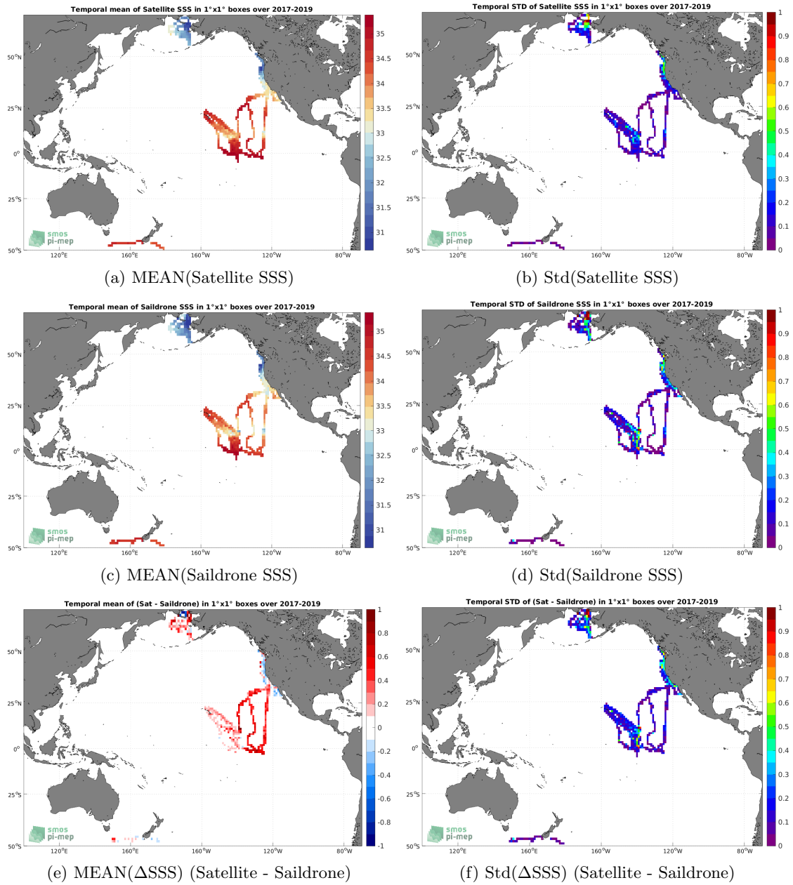
Figure 6: Temporal mean (left) and Std (right) of SSS from CCI SSS L4 Merged-OI v3.2 - 7-day running (ESA) (top), Saildrone (middle), and of \Delta SSS (Satellite - Saildrone). Only match-up pairs are used to generate these maps.
