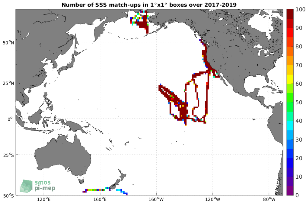
Figure 4: Number of SSS match-ups between Saildrone SSS and the CCI SSS L4 Merged-OI v3.2 - 7-day running (ESA) SSS product for the Pacific Ocean Pi-MEP region over 1^\circ \times 1^\circ boxes and for the full satellite product period.
