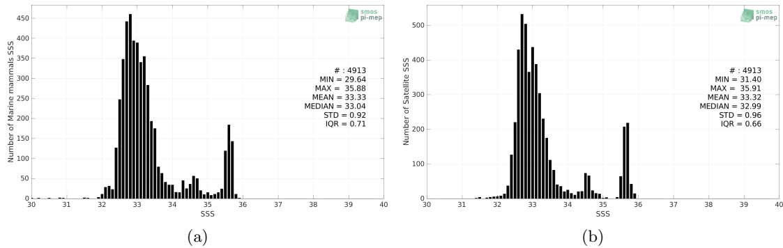
Figure 2: Histograms of SSS from Marine mammals (a) and CCI SSS L4 Merged-OI v3.2 - 7-day running (ESA) (b) considering all match-up pairs per bins of 0.1 over the Pacific Ocean Pi-MEP region and for the full satellite product period.
