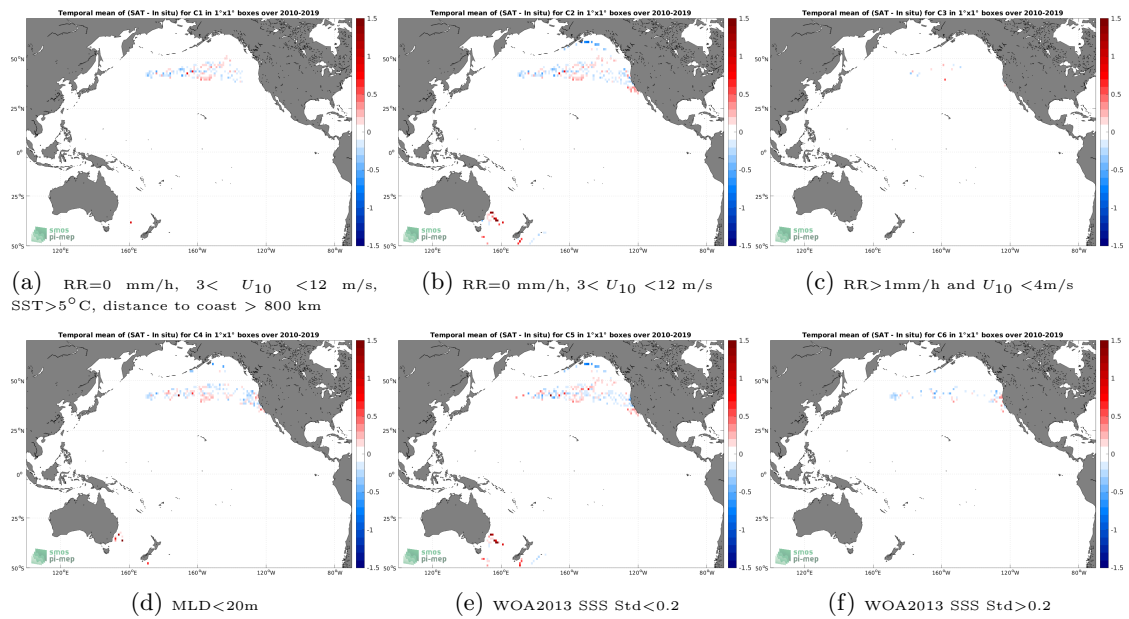
Figure 12: Temporal mean gridded over spatial boxes of size 1^\circ \times 1^\circ of \Delta SSS (CCI SSS L4 Merged-OI v3.2 - 7-day running (ESA) - Marine mammals) for 6 different subdatasets corresponding to:RR=0 mm/h, 3 < U_{10} < 12 m/s, SST >5^\circ C, distance to coast > 800 km (a), RR=0 mm/h, 3 < U_{10} < 12 m/s (b), RR >1 mm/h and U_{10} < 4 m/s (c),MLD <20 m (d),WOA2013 SSS Std <0.2 (e),WOA2013 SSS Std >0.2 (f).
