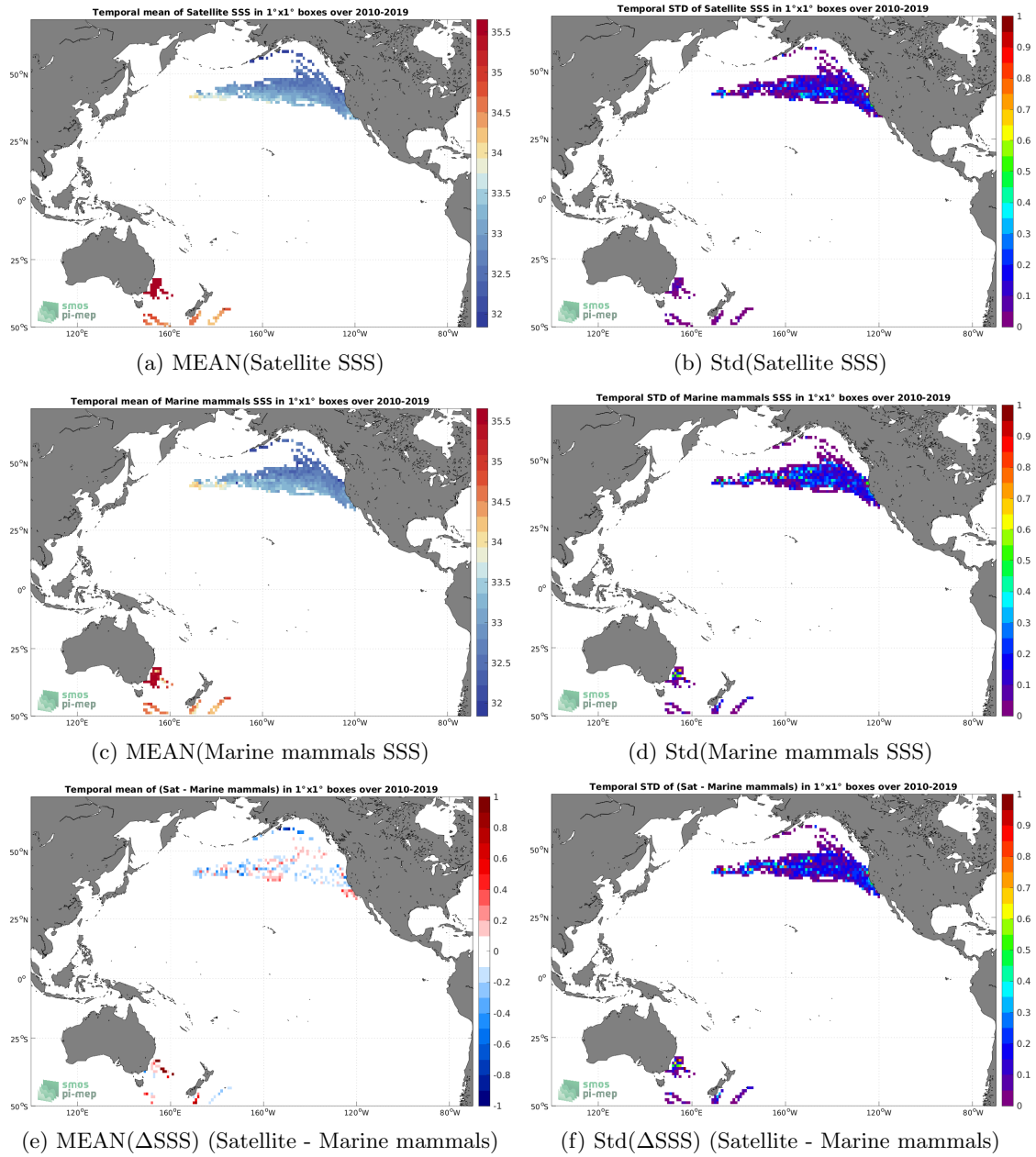
Figure 6: Temporal mean (left) and Std (right) of SSS from CCI SSS L4 Merged-OI v3.2 - 7-day running (ESA) (top), Marine mammals (middle), and of \Delta SSS (Satellite - Marine mammals). Only match-up pairs are used to generate these maps.
