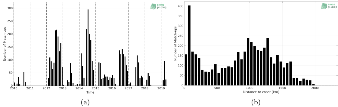
Figure 1: Number of match-ups between Marine mammals and CCI SSS L4 Merged-OI v3.2 - 7-day running (ESA) SSS as a function of time (a) and as function of the distance to coast (b) over the Pacific Ocean Pi-MEP region and for the full satellite product period.
