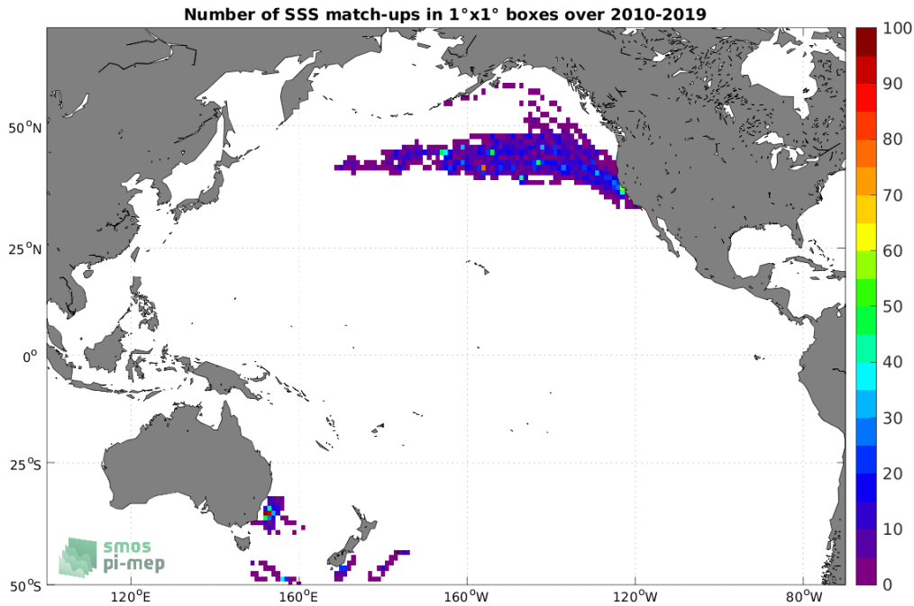
Figure 4: Number of SSS match-ups between Marine mammals SSS and the CCI SSS L4 Merged-OI v3.2 - 7-day running (ESA) SSS product for the Pacific Ocean Pi-MEP region over 1^\circ \times 1^\circ boxes and for the full satellite product period.
