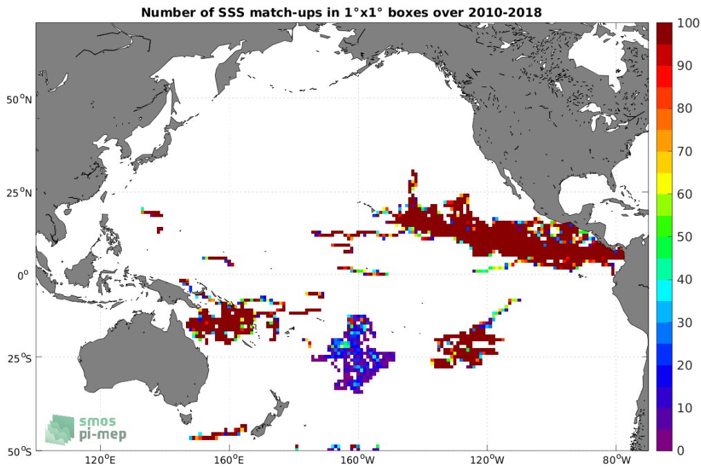
Figure 3: Number of SSS match-ups between Surface drifters SSS and the CCI SSS L4 Merged-OI v3.2 - 7-day running (ESA) SSS product for the Pacific Ocean Pi-MEP region over 1^\circ \times 1^\circ boxes and for the full satellite product period.
