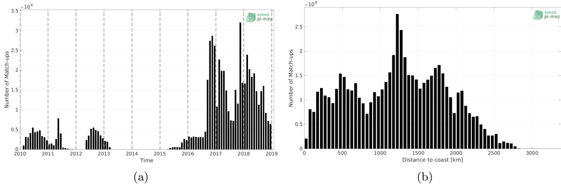
Figure 1: Number of match-ups between Surface drifters and CCI SSS L4 Merged-OI v3.2 - 7-day running (ESA) SSS as a function of time (a) and as function of the distance to coast (b) over the Pacific Ocean Pi-MEP region and for the full satellite product period.
