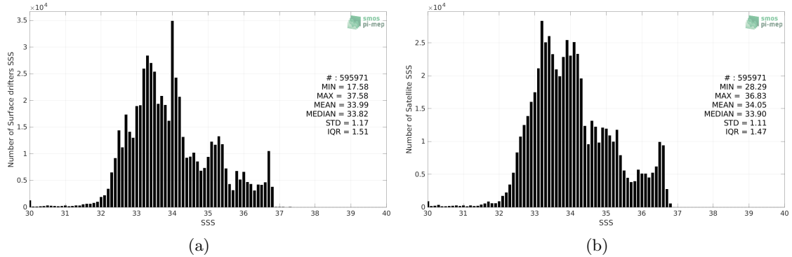
Figure 2: Histograms of SSS from Surface drifters (a) and CCI SSS L4 Merged-OI v3.2 - 7-day running (ESA) (b) considering all match-up pairs per bins of 0.1 over the Pacific Ocean Pi-MEP region and for the full satellite product period.
