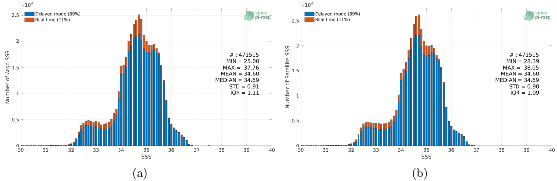
Figure 2: Histograms of SSS from Argo (a) and CCI SSS L4 Merged-OI v3.2 - 7-day running (ESA) (b) considering all match-up pairs per bins of 0.1 over the Pacific Ocean Pi-MEP region and for the full satellite product period.
