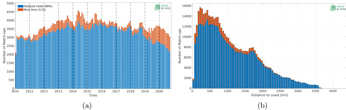
Figure 1: Number of match-ups between Argo and CCI SSS L4 Merged-OI v3.2 - 7-day running (ESA) SSS as a function of time (a) and as function of the distance to coast (b) over the Pacific Ocean Pi-MEP region and for the full satellite product period.
