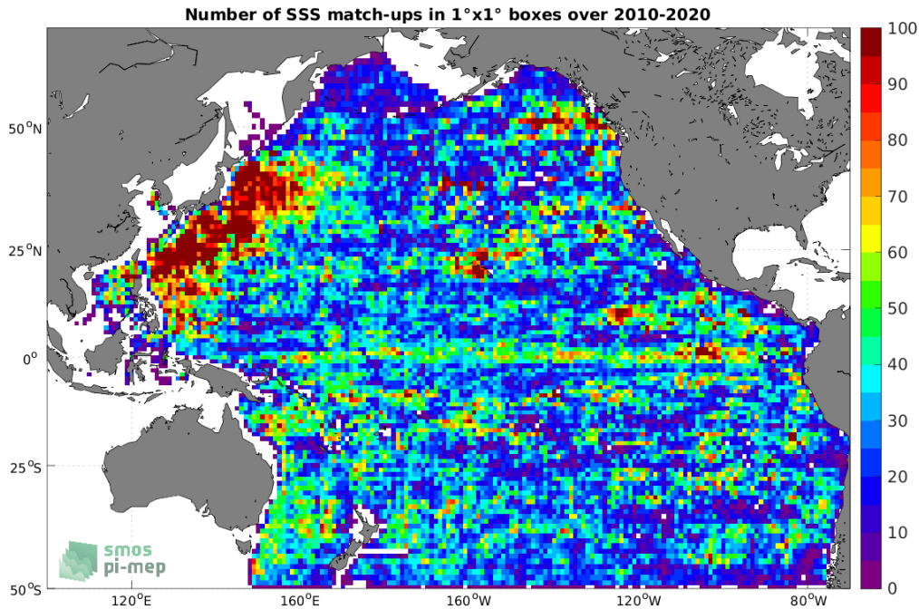
Figure 4: Number of SSS match-ups between Argo SSS and the CCI SSS L4 Merged-OI v3.2 - 7-day running (ESA) SSS product for the Pacific Ocean Pi-MEP region over 1^\circ \times 1^\circ boxes and for the full satellite product period.
