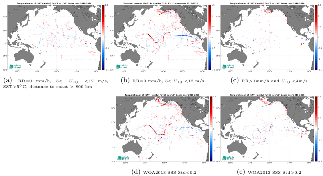
Figure 12: Temporal mean gridded over spatial boxes of size 1^\circ \times 1^\circ of \Delta\text{SSS} (CCI SSS L4 Merged-OI v3.2 - 30-day running (ESA) - TSG (SAMOS)) for 5 different subdatasets corresponding to:RR=0 mm/h, 3 < U_{10} < 12 m/s, SST > 5^\circ\text{C} , distance to coast > 800 km (a), RR=0 mm/h, 3 < U_{10} < 12 m/s (b), RR > 1 mm/h and U_{10} < 4 m/s (c), WOA2013 SSS Std < 0.2 (d), WOA2013 SSS Std > 0.2 (e).
