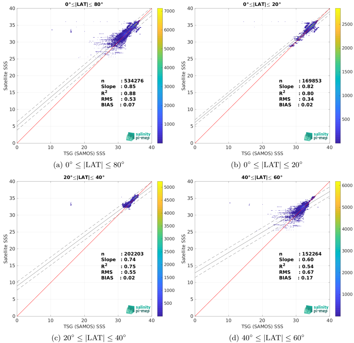
Figure 9: Contour maps of the concentration of CCI SSS L4 Merged-OI v3.2 - 30-day running (ESA) SSS (y-axis) versus TSG (SAMOS) SSS (x-axis) at match-up pairs for different latitude bands. For each plot, the red line shows x=y . The black thin and dashed lines indicate a linear fit through the data cloud and the \pm 95\% confidence levels, respectively. The number match-up pairs n , the slope and R^2 coefficient of the linear fit, the root mean square (RMS) and the mean bias between satellite and in situ data are indicated for each latitude band in each plots.
