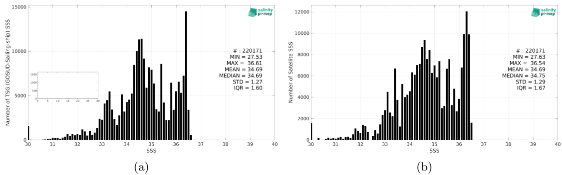
Figure 2: Histograms of SSS from TSG (GOSUD-Sailing-ship) (a) and CCI SSS L4 Merged-OI v3.2 - 30-day running (ESA) (b) considering all match-up pairs per bins of 0.1 over the Pacific Ocean Pi-MEP region and for the full satellite product period.
