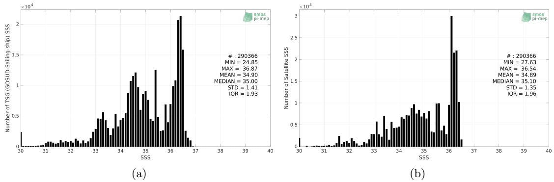
Figure 2: Histograms of SSS from TSG (GOSUD-Sailing-ship) (a) and CCI SSS L4 Merged-OI v3.2 - 30-day running (ESA) (b) considering all match-up pairs per bins of 0.1 over the Pacific Ocean Pi-MEP region and for the full satellite product period.
