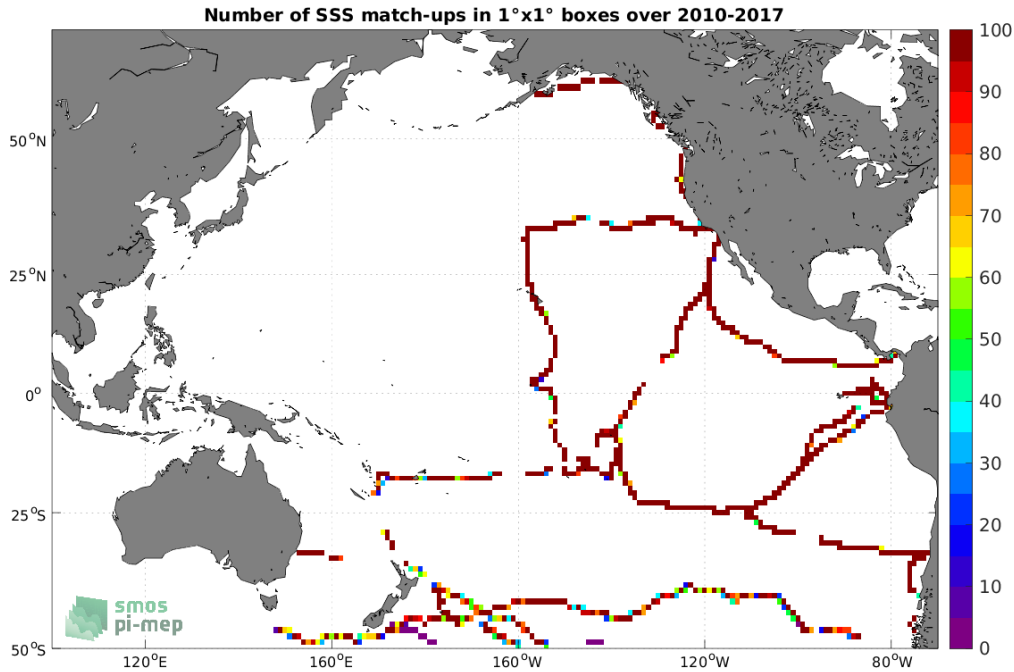
Figure 4: Number of SSS match-ups between TSG (GOSUD-Sailing-ship) SSS and the CCI SSS L4 Merged-OI v3.2 - 30-day running (ESA) SSS product for the Pacific Ocean Pi-MEP region over 1^\circ \times 1^\circ boxes and for the full satellite product period.
