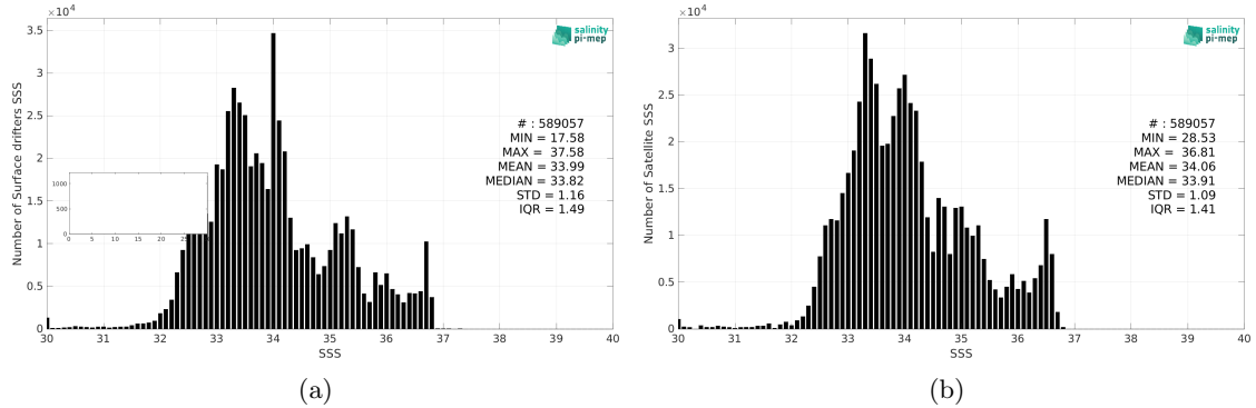
Figure 2: Histograms of SSS from Surface drifters (a) and CCI SSS L4 Merged-OI v3.2 - 30-day running (ESA) (b) considering all match-up pairs per bins of 0.1 over the Pacific Ocean Pi-MEP region and for the full satellite product period.
