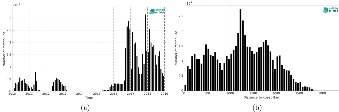
Figure 1: Number of match-ups between Surface drifters and CCI SSS L4 Merged-OI v3.2 - 30-day running (ESA) SSS as a function of time (a) and as function of the distance to coast (b) over the Pacific Ocean Pi-MEP region and for the full satellite product period.
