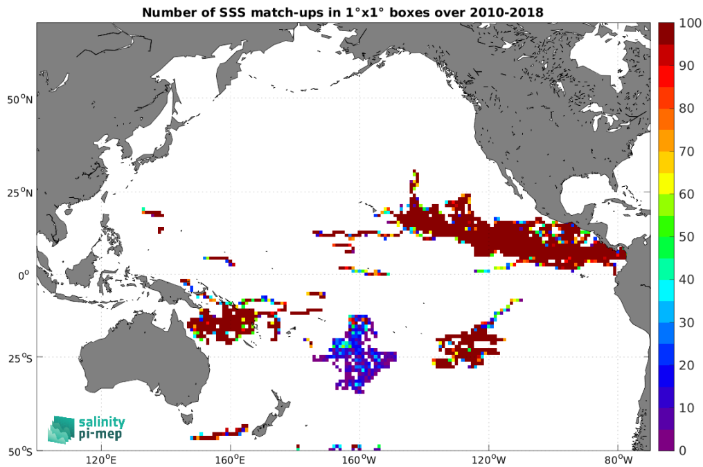
Figure 3: Number of SSS match-ups between Surface drifters SSS and the CCI SSS L4 Merged-OI v3.2 - 30-day running (ESA) SSS product for the Pacific Ocean Pi-MEP region over 1^\circ \times 1^\circ boxes and for the full satellite product period.
