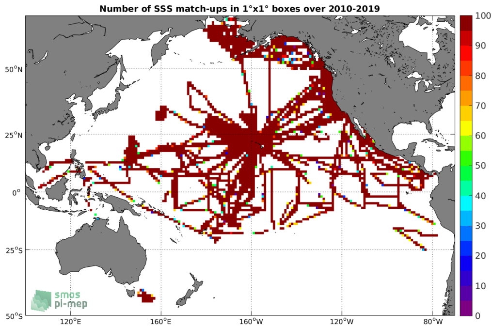
Figure 4: Number of SSS match-ups between TSG (SAMOS) SSS and the CCI L4 Merged-OI v2.31 - 7-day running (ESA) SSS product for the Pacific Ocean Pi-MEP region over 1^\circ \times 1^\circ boxes and for the full satellite product period.
