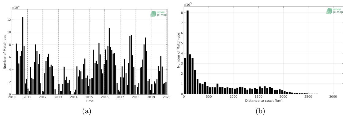
Figure 1: Number of match-ups between TSG (SAMOS) and CCI L4 Merged-OI v2.31 - 7-day running (ESA) SSS as a function of time (a) and as function of the distance to coast (b) over the Pacific Ocean Pi-MEP region and for the full satellite product period.
