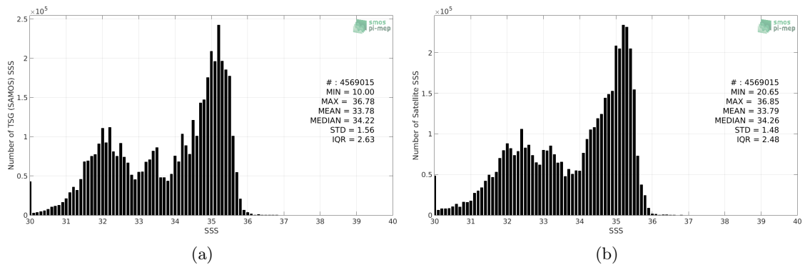
Figure 2: Histograms of SSS from TSG (SAMOS) (a) and CCI L4 Merged-OI v2.31 - 7-day running (ESA) (b) considering all match-up pairs per bins of 0.1 over the Pacific Ocean Pi-MEP region and for the full satellite product period.
