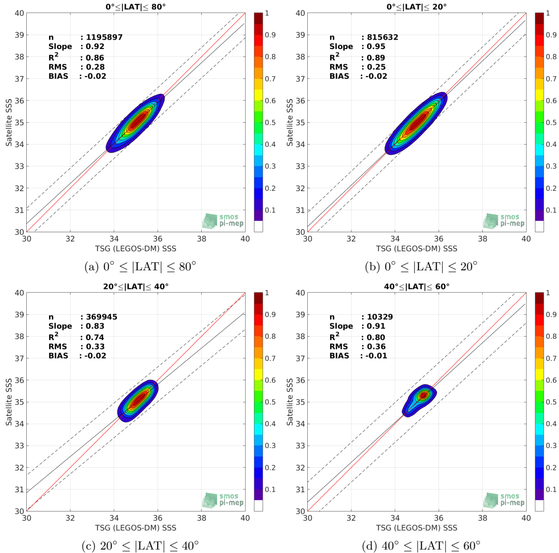
Figure 9: Contour maps of the concentration of CCI SSS L4 Merged-OI v2.31 - 7-day running (ESA) SSS (y-axis) versus TSG (LEGOS-DM) SSS (x-axis) at match-up pairs for different latitude bands. For each plot, the red line shows x=y . The black thin and dashed lines indicate a linear fit through the data cloud and the \pm 95\% confidence levels, respectively. The number match-up pairs n , the slope and R^2 coefficient of the linear fit, the root mean square (RMS) and the mean bias between satellite and in situ data are indicated for each latitude band in each plots.
