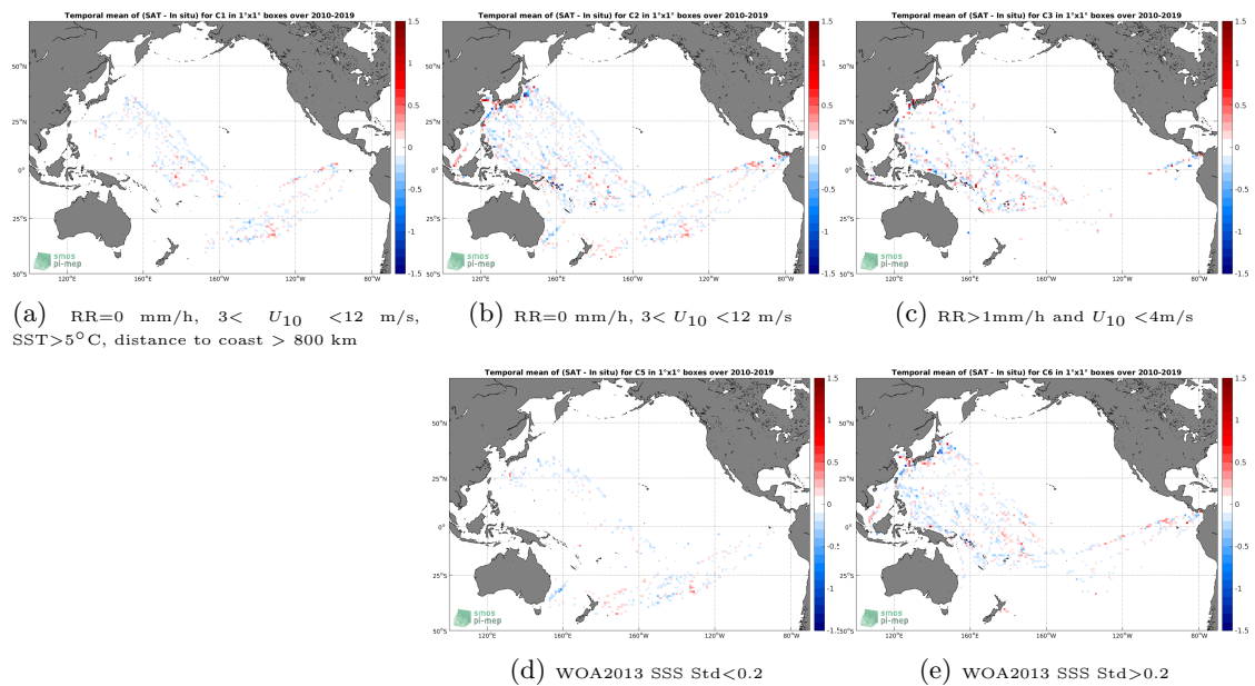
Figure 12: Temporal mean gridded over spatial boxes of size 1^\circ \times 1^\circ of \Delta SSS (CCI SSS L4 Merged-OI v2.31 - 7-day running (ESA) - TSG (LEGOS-DM)) for 5 different subdatasets corresponding to:RR=0 mm/h, 3 < U_{10} < 12 m/s, SST>5°C, distance to coast > 800 km (a), RR=0 mm/h, 3 < U_{10} < 12 m/s (b), RR>1mm/h and U_{10} < 4 m/s (c), WOA2013 SSS Std<0.2 (d), WOA2013 SSS Std>0.2 (e).
