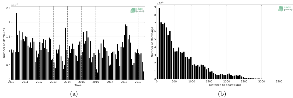
Figure 1: Number of match-ups between TSG (LEGOS-DM) and CCI SSS L4 Merged-OI v2.31 - 7-day running (ESA) SSS as a function of time (a) and as function of the distance to coast (b) over the Pacific Ocean Pi-MEP region and for the full satellite product period.
