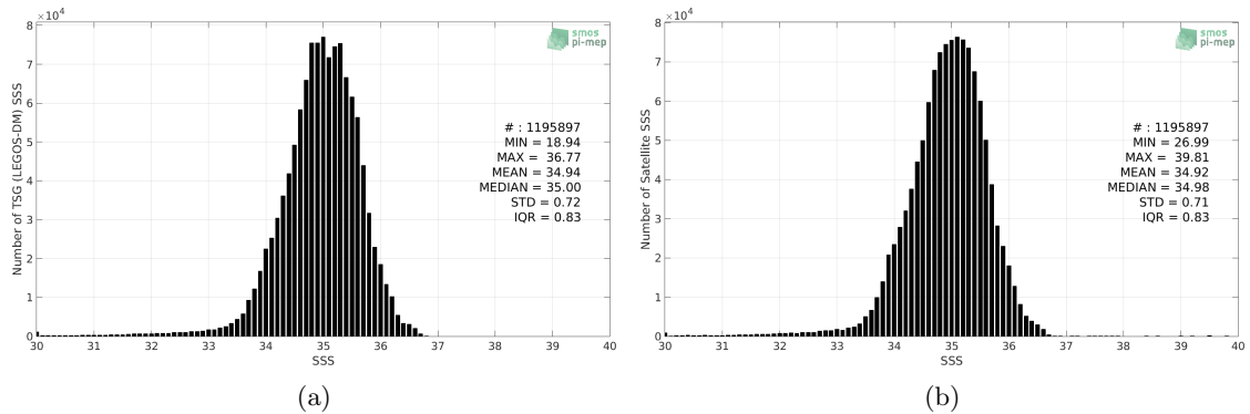
Figure 2: Histograms of SSS from TSG (LEGOS-DM) (a) and CCI SSS L4 Merged-OI v2.31 - 7-day running (ESA) (b) considering all match-up pairs per bins of 0.1 over the Pacific Ocean Pi-MEP region and for the full satellite product period.
