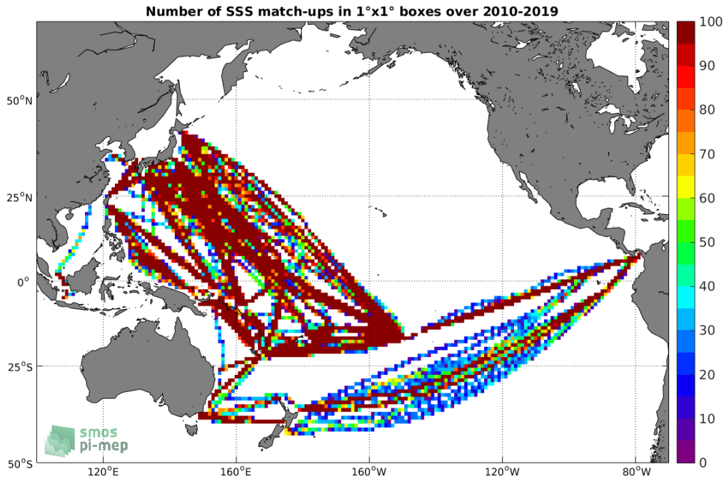
Figure 4: Number of SSS match-ups between TSG (LEGOS-DM) SSS and the CCI SSS L4 Merged-OI v2.31 - 7-day running (ESA) SSS product for the Pacific Ocean Pi-MEP region over 1°x1° boxes and for the full satellite product period.
