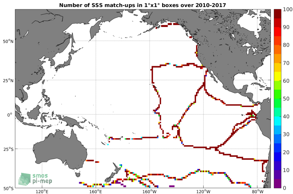
Figure 4: Number of SSS match-ups between TSG (GOSUD-Sailing-ship) SSS and the CCI SSS L4 Merged-OI v2.31 - 7-day running (ESA) SSS product for the Pacific Ocean Pi-MEP region over 1^\circ \times 1^\circ boxes and for the full satellite product period.
