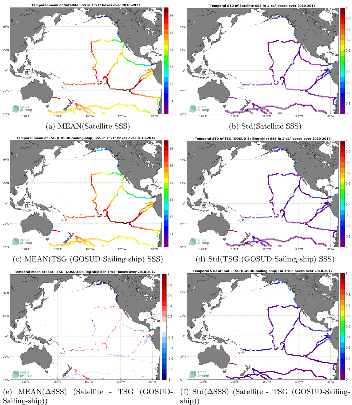
Figure 6: Temporal mean (left) and Std (right) of SSS from CCI SSS L4 Merged-OI v2.31 - 7-day running (ESA) (top), TSG (GOSUD-Sailing-ship) (middle), and of \Delta SSS (Satellite - TSG (GOSUD-Sailing-ship)). Only match-up pairs are used to generate these maps.
