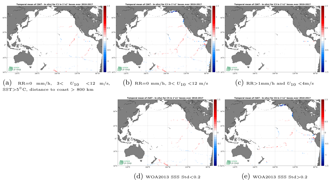
Figure 12: Temporal mean gridded over spatial boxes of size 1^\circ \times 1^\circ of \Delta SSS (CCI SSS L4 Merged-OI v2.31 - 7-day running (ESA) - TSG (GOSUD-Sailing-ship)) for 5 different subdatasets corresponding to:RR=0 mm/h, 3 < U_{10} < 12 m/s, SST>5°C, distance to coast > 800 km (a), RR=0 mm/h, 3 < U_{10} < 12 m/s (b), RR>1mm/h and U_{10} < 4 m/s (c), WOA2013 SSS Std<0.2 (d), WOA2013 SSS Std>0.2 (e).
