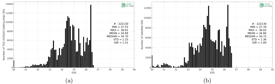
Figure 2: Histograms of SSS from TSG (GOSUD-Sailing-ship) (a) and CCI SSS L4 Merged-OI v2.31 - 7-day running (ESA) (b) considering all match-up pairs per bins of 0.1 over the Pacific Ocean Pi-MEP region and for the full satellite product period.
