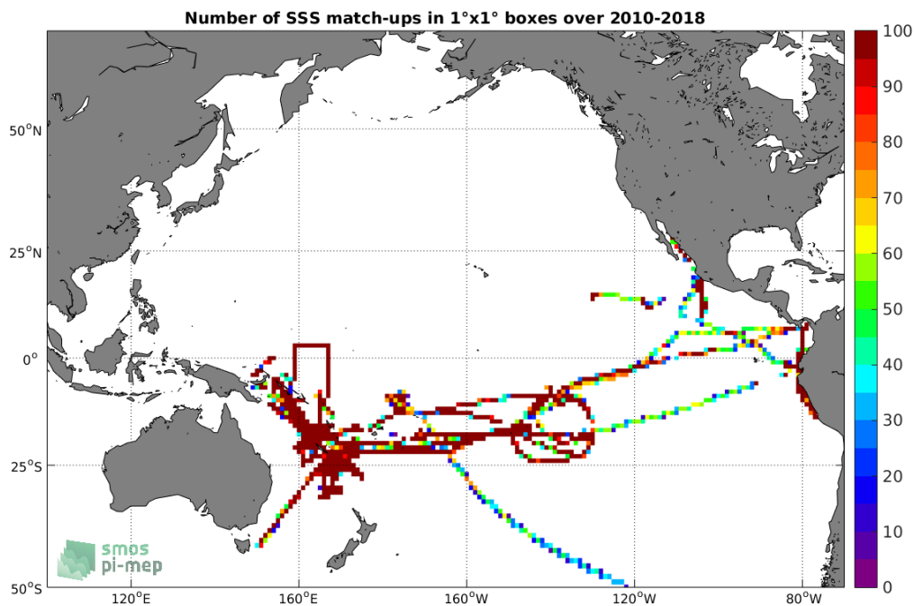
Figure 4: Number of SSS match-ups between TSG (GOSUD-Research-vessel) SSS and the CCI SSS L4 Merged-OI v2.31 - 7-day running (ESA) SSS product for the Pacific Ocean Pi-MEP region over 1^\circ \times 1^\circ boxes and for the full satellite product period.
