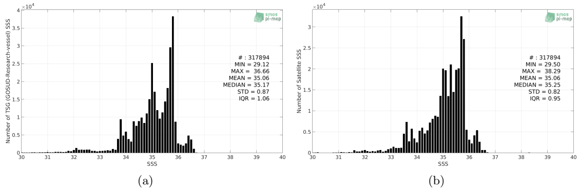
Figure 2: Histograms of SSS from TSG (GOSUD-Research-vessel) (a) and CCI SSS L4 Merged-OI v2.31 - 7-day running (ESA) (b) considering all match-up pairs per bins of 0.1 over the Pacific Ocean Pi-MEP region and for the full satellite product period.
