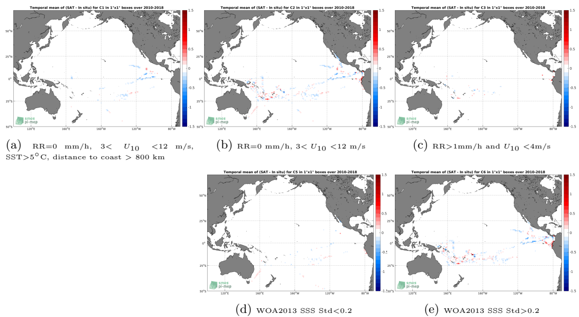
Figure 12: Temporal mean gridded over spatial boxes of size 1^\circ \times 1^\circ of \Delta SSS (CCI SSS L4 Merged-OI v2.31 - 7-day running (ESA) - TSG (GOSUD-Research-vessel)) for 5 different subdatasets corresponding to: RR=0 mm/h, 3 < U_{10} < 12 m/s, SST > 5°C, distance to coast > 800 km (a), RR=0 mm/h, 3 < U_{10} < 12 m/s (b), RR > 1mm/h and U_{10} < 4 m/s (c), WOA2013 SSS Std < 0.2 (d), WOA2013 SSS Std > 0.2 (e).
