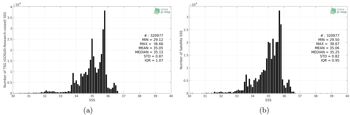
Figure 2: Histograms of SSS from TSG (GOSUD-Research-vessel) (a) and CCI L4 Merged-OI v2.31 - 7-day running (ESA) (b) considering all match-up pairs per bins of 0.1 over the Pacific Ocean Pi-MEP region and for the full satellite product period.
