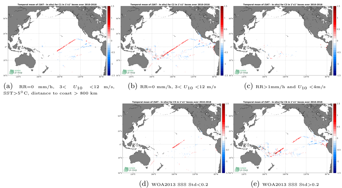
Figure 12: Temporal mean gridded over spatial boxes of size 1^\circ \times 1^\circ of \Delta SSS (CCI L4 Merged-OI v2.31 - 7-day running (ESA) - TSG (GOSUD-Research-vessel)) for 5 different subdatasets corresponding to: RR=0 mm/h, 3 < U_{10} < 12 m/s, SST > 5°C, distance to coast > 800 km (a), RR=0 mm/h, 3 < U_{10} < 12 m/s (b), RR > 1mm/h and U_{10} < 4 m/s (c), WOA2013 SSS Std < 0.2 (d), WOA2013 SSS Std > 0.2 (e).
