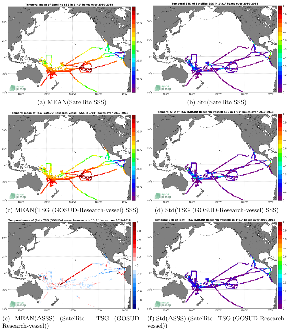
Figure 6: Temporal mean (left) and Std (right) of SSS from CCI L4 Merged-OI v2.31 - 7-day running (ESA) (top), TSG (GOSUD-Research-vessel) (middle), and of \Delta SSS (Satellite - TSG (GOSUD-Research-vessel)). Only match-up pairs are used to generate these maps.
