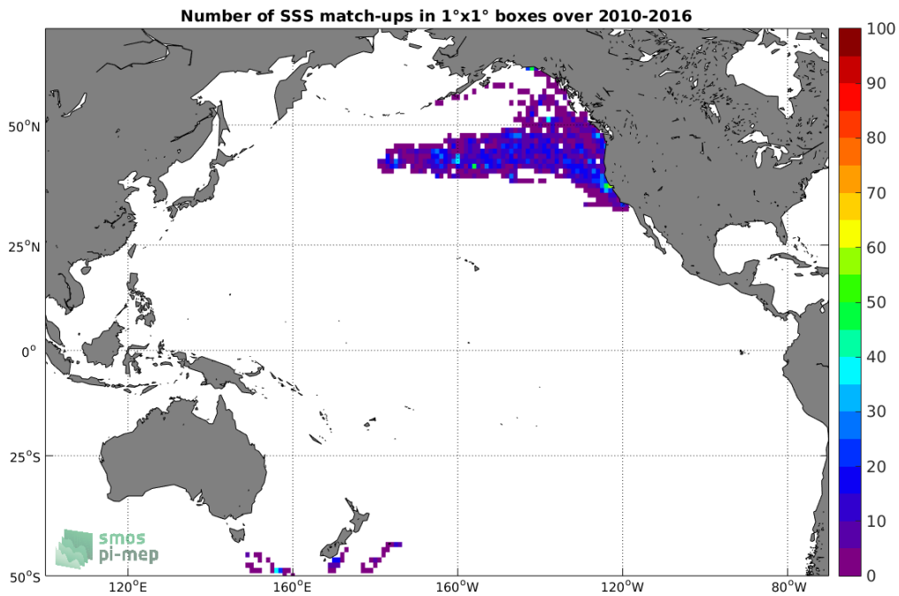
Figure 4: Number of SSS match-ups between Sea mammals SSS and the CCI SSS L4 Merged-OI v2.31 - 7-day running (ESA) SSS product for the Pacific Ocean Pi-MEP region over 1°x1° boxes and for the full satellite product period.
