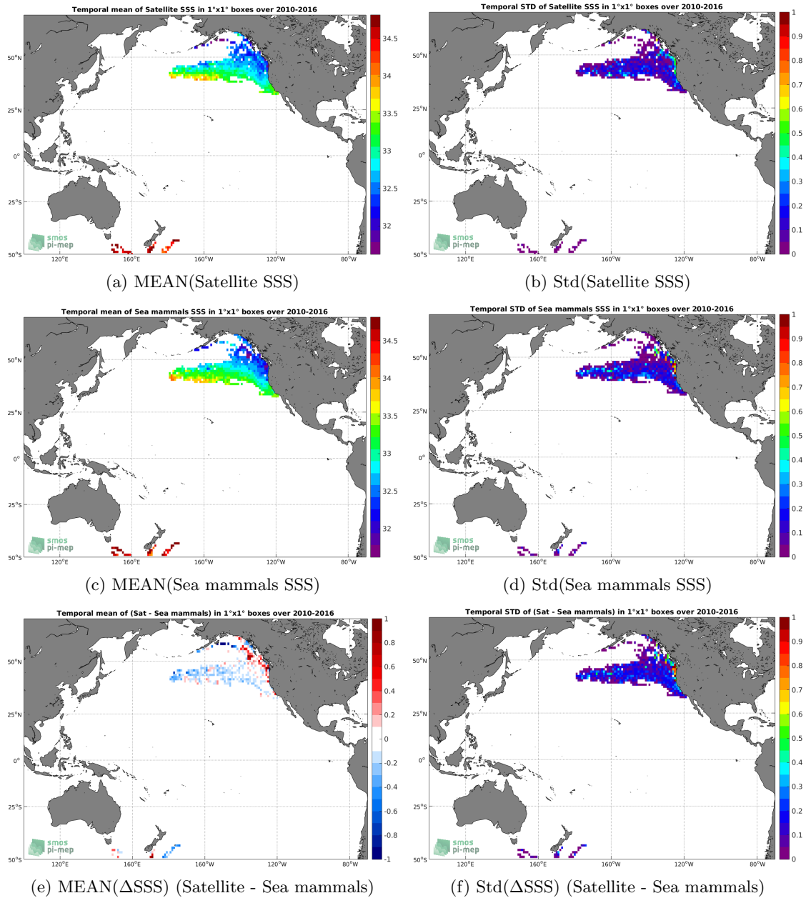
Figure 6: Temporal mean (left) and Std (right) of SSS from CCI SSS L4 Merged-OI v2.31 - 7-day running (ESA) (top), Sea mammals (middle), and of \Delta SSS (Satellite - Sea mammals). Only match-up pairs are used to generate these maps.
