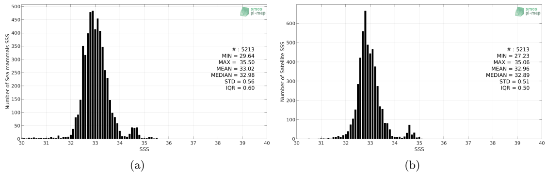
Figure 2: Histograms of SSS from Sea mammals (a) and CCI SSS L4 Merged-OI v2.31 - 7-day running (ESA) (b) considering all match-up pairs per bins of 0.1 over the Pacific Ocean Pi-MEP region and for the full satellite product period.
