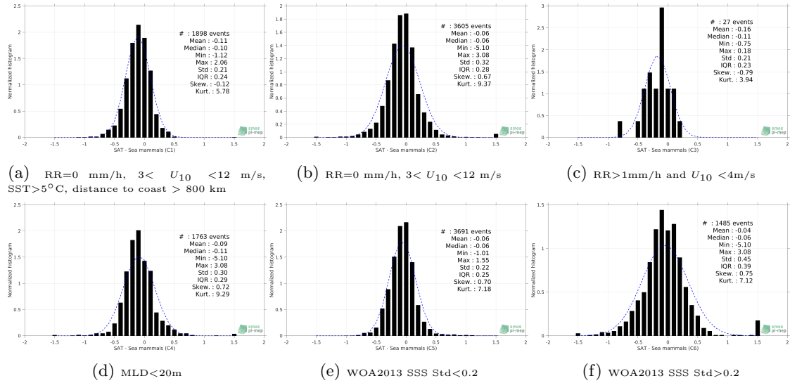
Figure 13: Normalized histogram of \Delta\text{SSS} (CCI SSS L4 Merged-OI v2.31 - 7-day running (ESA) - Sea mammals) for 6 different subdatasets corresponding to: RR=0 mm/h, 3 < U_{10} < 12 m/s, SST>5°C, distance to coast > 800 km (a), RR=0 mm/h, 3 < U_{10} < 12 m/s (b), RR>1mm/h and U_{10} < 4 m/s (c), MLD<20m (d), WOA2013 SSS Std<0.2 (e), WOA2013 SSS Std>0.2 (f).
