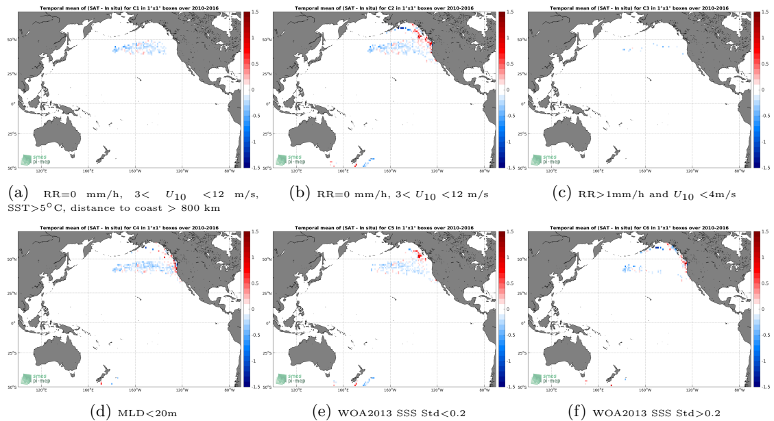
Figure 12: Temporal mean gridded over spatial boxes of size 1^\circ \times 1^\circ of \Delta SSS (CCI SSS L4 Merged-OI v2.31 - 7-day running (ESA) - Sea mammals) for 6 different subdatasets corresponding to:RR=0 mm/h, 3 < U_{10} < 12 m/s, SST >5^\circ C, distance to coast > 800 km (a), RR=0 mm/h, 3 < U_{10} < 12 m/s (b), RR >1 mm/h and U_{10} < 4 m/s (c),MLD <20 m (d),WOA2013 SSS Std <0.2 (e),WOA2013 SSS Std >0.2 (f).
