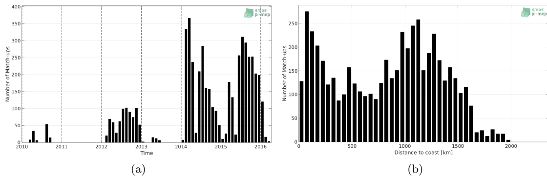
Figure 1: Number of match-ups between Sea mammals and CCI SSS L4 Merged-OI v2.31 - 7-day running (ESA) SSS as a function of time (a) and as function of the distance to coast (b) over the Pacific Ocean Pi-MEP region and for the full satellite product period.
