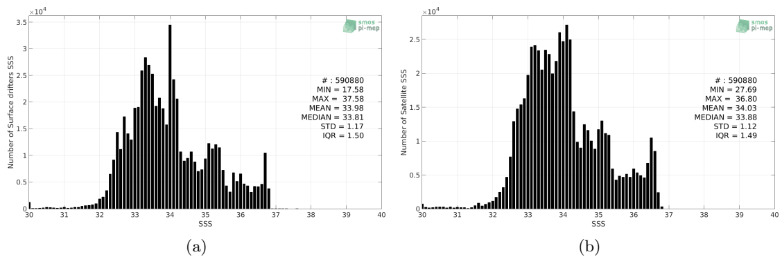
Figure 2: Histograms of SSS from Surface drifters (a) and CCI SSS L4 Merged-OI v2.31 - 7-day running (ESA) (b) considering all match-up pairs per bins of 0.1 over the Pacific Ocean Pi-MEP region and for the full satellite product period.
