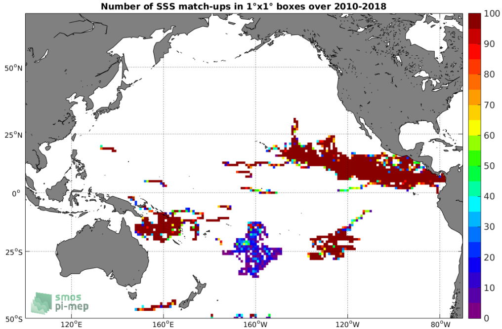
Figure 3: Number of SSS match-ups between Surface drifters SSS and the CCI SSS L4 Merged-OI v2.31 - 7-day running (ESA) SSS product for the Pacific Ocean Pi-MEP region over 1°x1° boxes and for the full satellite product period.
