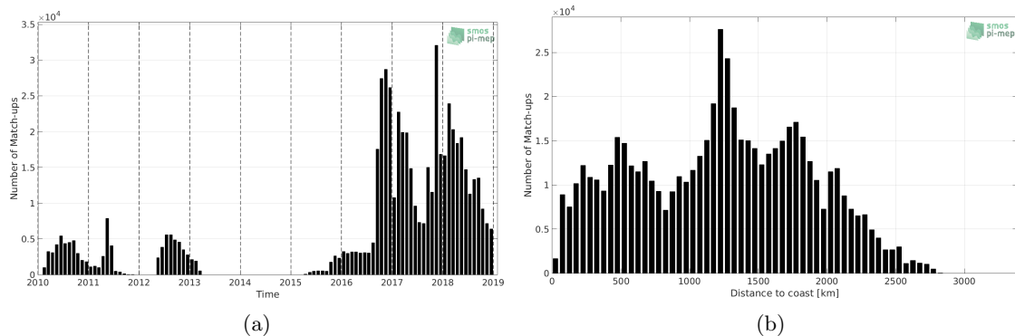
Figure 1: Number of match-ups between Surface drifters and CCI SSS L4 Merged-OI v2.31 - 7-day running (ESA) SSS as a function of time (a) and as function of the distance to coast (b) over the Pacific Ocean Pi-MEP region and for the full satellite product period.
