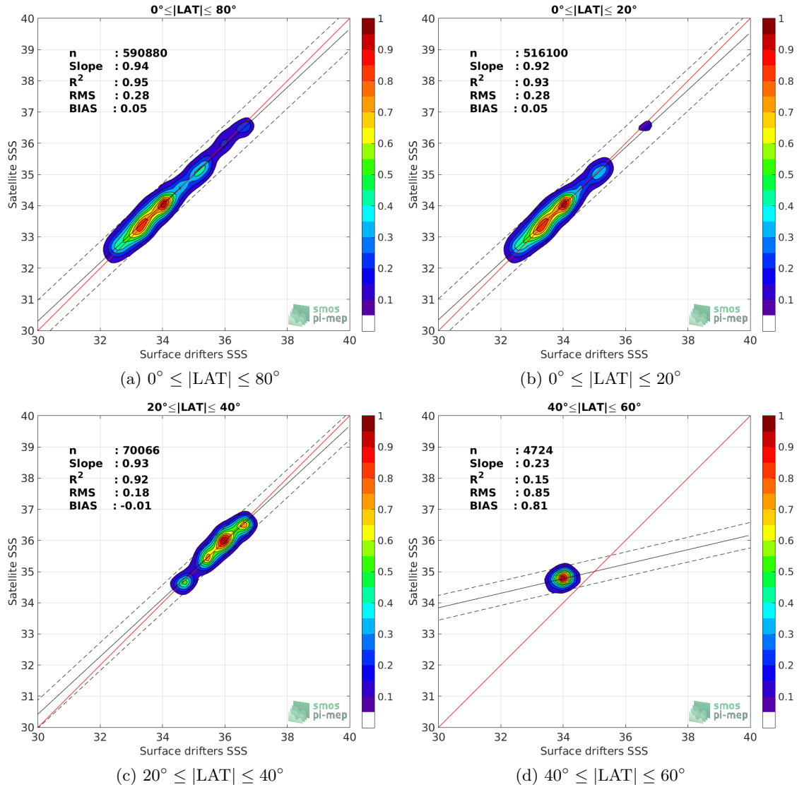
Figure 8: Contour maps of the concentration of CCI L4 Merged-OI v2.31 - 7-day running (ESA) SSS (y-axis) versus Surface drifters SSS (x-axis) at match-up pairs for different latitude bands. For each plot, the red line shows x=y . The black thin and dashed lines indicate a linear fit through the data cloud and the \pm 95\% confidence levels, respectively. The number match-up pairs n , the slope and R^2 coefficient of the linear fit, the root mean square (RMS) and the mean bias between satellite and in situ data are indicated for each latitude band in each plots.
