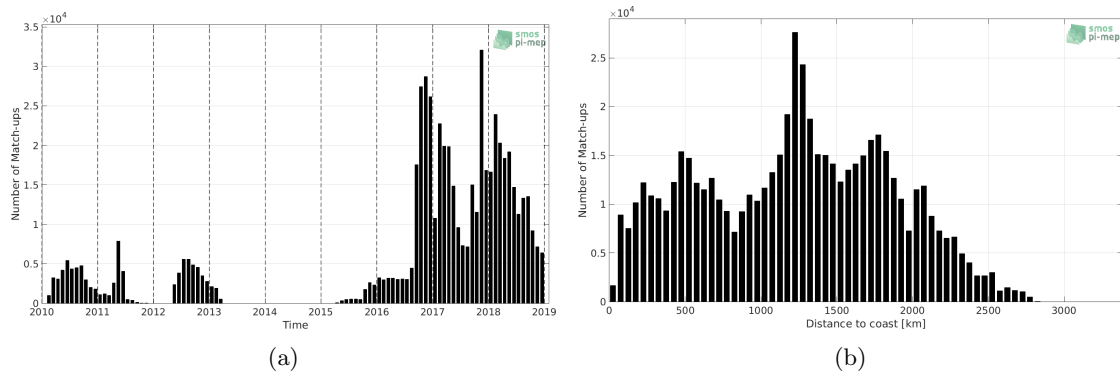
Figure 1: Number of match-ups between Surface drifters and CCI L4 Merged-OI v2.31 - 7-day running (ESA) SSS as a function of time (a) and as function of the distance to coast (b) over the Pacific Ocean Pi-MEP region and for the full satellite product period.
