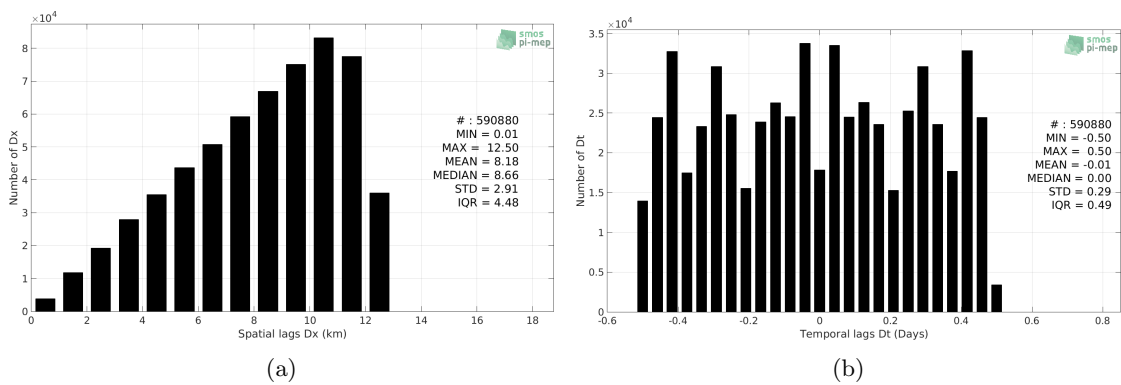
Figure 4: Histograms of the spatial (a) and temporal (b) lags between the time of the Surface drifters measurements and the date of the corresponding CCI L4 Merged-OI v2.31 - 7-day running (ESA) SSS product.
