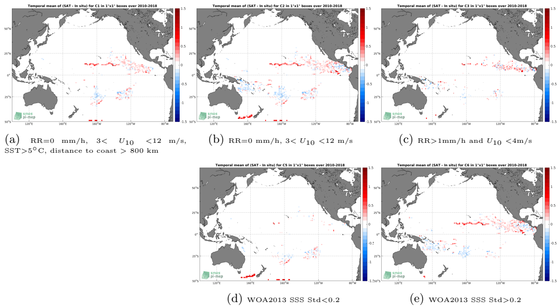
Figure 11: Temporal mean gridded over spatial boxes of size 1°x1° of \Delta SSS (CCI L4 Merged-OI v2.31 - 7-day running (ESA) - Surface drifters) for 5 different subdatasets corresponding to:RR=0 mm/h, 3 < U_{10} < 12 m/s, SST > 5°C, distance to coast > 800 km (a), RR=0 mm/h, 3 < U_{10} < 12 m/s (b), RR > 1mm/h and U_{10} < 4 m/s (c), WOA2013 SSS Std < 0.2 (d), WOA2013 SSS Std > 0.2 (e).
