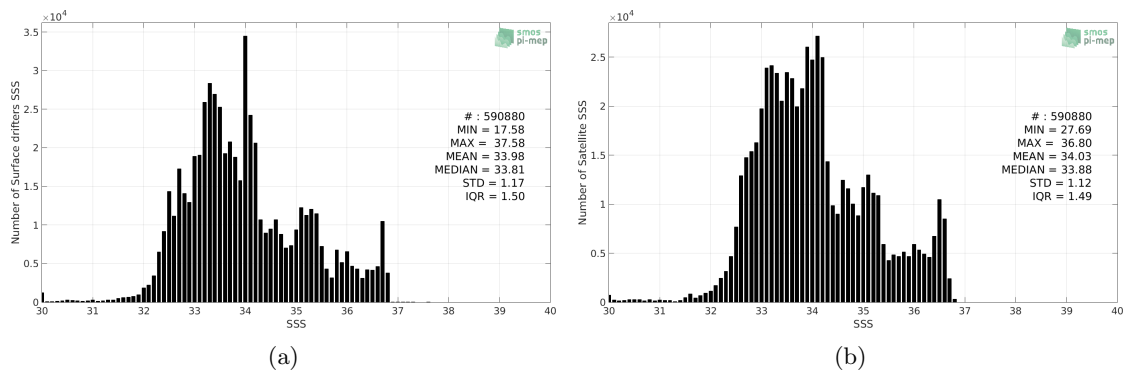
Figure 2: Histograms of SSS from Surface drifters (a) and CCI L4 Merged-OI v2.31 - 7-day running (ESA) (b) considering all match-up pairs per bins of 0.1 over the Pacific Ocean Pi-MEP region and for the full satellite product period.
