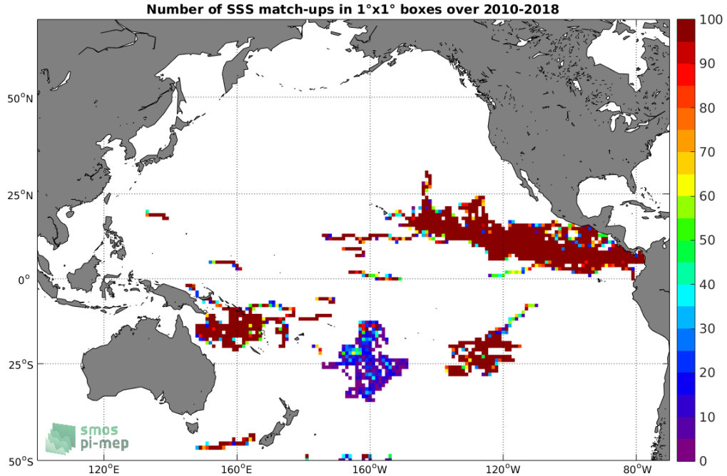
Figure 3: Number of SSS match-ups between Surface drifters SSS and the CCI L4 Merged-OI v2.31 - 7-day running (ESA) SSS product for the Pacific Ocean Pi-MEP region over 1^\circ \times 1^\circ boxes and for the full satellite product period.
