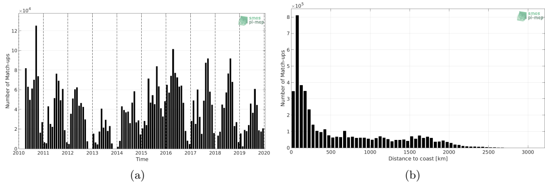
Figure 1: Number of match-ups between TSG (SAMOS) and CCI L4 Merged-OI v2.31 - 30-day running (ESA) SSS as a function of time (a) and as function of the distance to coast (b) over the Pacific Ocean Pi-MEP region and for the full satellite product period.
