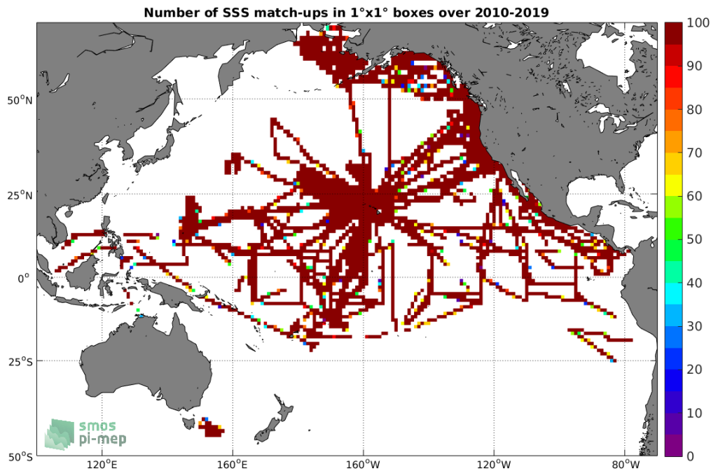
Figure 4: Number of SSS match-ups between TSG (SAMOS) SSS and the CCI L4 Merged-OI v2.31 - 30-day running (ESA) SSS product for the Pacific Ocean Pi-MEP region over 1^\circ \times 1^\circ boxes and for the full satellite product period.
