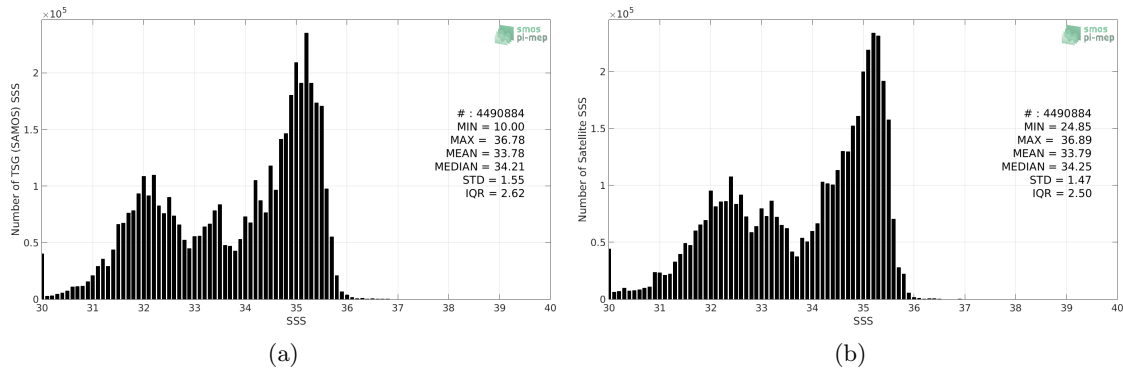
Figure 2: Histograms of SSS from TSG (SAMOS) (a) and CCI L4 Merged-OI v2.31 - 30-day running (ESA) (b) considering all match-up pairs per bins of 0.1 over the Pacific Ocean Pi-MEP region and for the full satellite product period.
